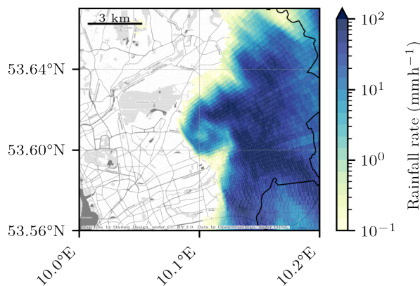
Figure 9. Rainfall pattern during a Tornado event on 07.06.2016 at 16:20:30 UTC. The rainfall rate is shown for a north-eastern section of the measurement domain in Hamburg.
