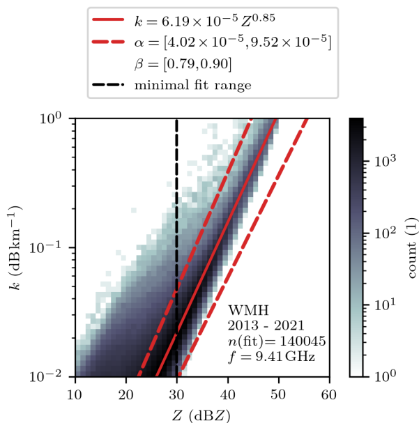
Figure 4. Relation between the specific attenuation k and the radar reflectivity dBZ estimated from micro rain radar measurements at 105 m height and 10s temporal resolution. Only measurements at temperatures above 0^{\circ}\text{C} are used to exclude ice phase. The radar variables are computed at the X-band frequency from measured drop size distributions with T-matrix calculations (Waterman, 1965) implemented by Leinonen (2014) using raindrop axis ratios from Brandes et al. (2002), a canting angle distribution with zero mean and 10^{\circ} width, and the complex refractive index of water from Liebe et al. (1991) at a temperature of 15^{\circ}\text{C} . The power-law fit for the k - Z relation is based on measurements above 30 dBZ (dashed black line) and is shown with a red solid line, including uncertainties indicated as dashed red line.
