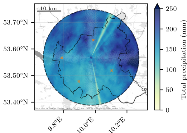
Figure 10. Three-month total precipitation measured by the LAWWR during June, July, and August 2019. The radar estimates at four rain gauge locations (orange crosses) are 174.7 mm (north), 146.7 mm (east), 132.1 mm (south), and 157.1 mm (west).
