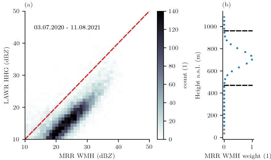
Figure 3. Calibration of X-band radar (LAWR) reflectivities using height averaged micro rain radar (MRR) WMH reflectivities. (a) Comparison of uncalibrated X-band radar (LAWR) reflectivities to calibrated radar reflectivities of the micro rain radar (MRR) WMH of the period 03.07.2020 to 11.08.2021 (Table 4). (b) Weights (dots) to average the MRR WMH reflectivity profile within the LAWV HHG beam (indicated by black dashed line) measuring at a beam elevation of 3.5^\circ .
