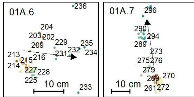
255 Figure 8. Position changes of the stake 01A.6 and 01A.7. The numbers and colours (from red to dark green) indicates subsequent measurements.
