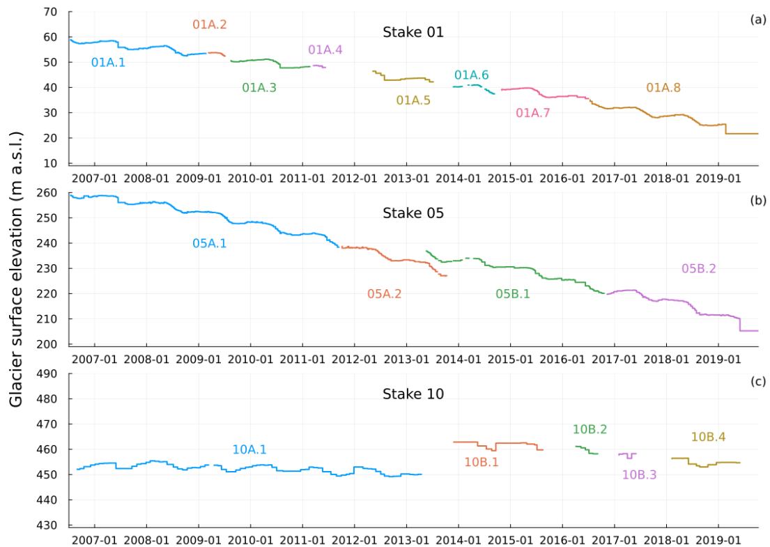
315 Figure 7. Representative dataset of height measurements of stake 01, 05, 10.
