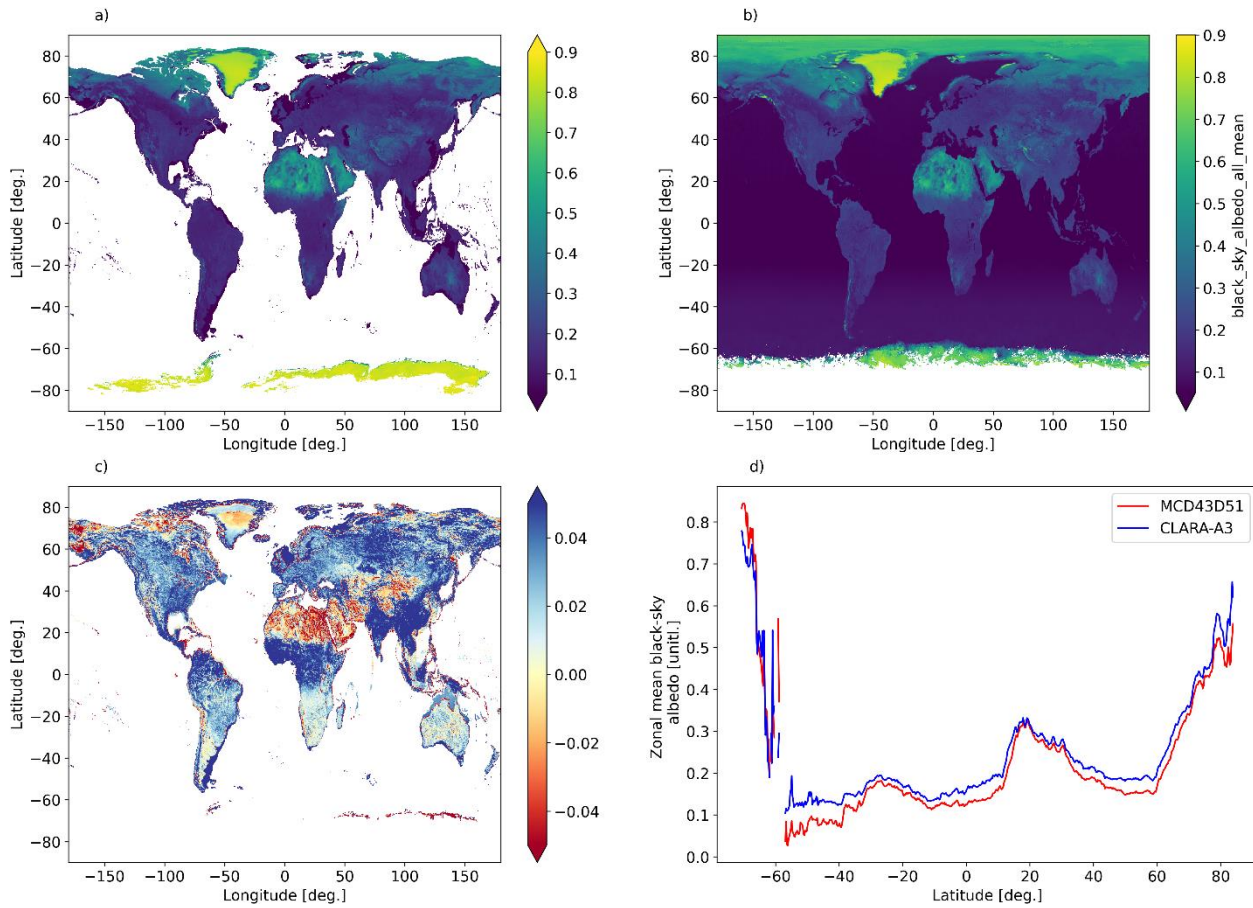
Figure 1140: Intercomparison of CLARA-A3 and MCD43D51 black-sky albedo estimates. Data shown corresponds to the mean of April-September 2015. (a) MCD43D51, (b) CLARA-A3, (c) difference (CLARA-MCD43), (d) zonal means of MCD43D51 and CLARA-A3.
