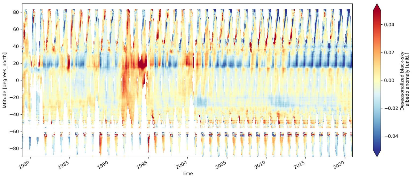
Figure 134: Deseasonalized zonal monthly mean black-sky surface albedo anomalies against 1982-1998 mean. Data shown only for land & snow surfaces with >85% zonal coverage during the evaluated month.
