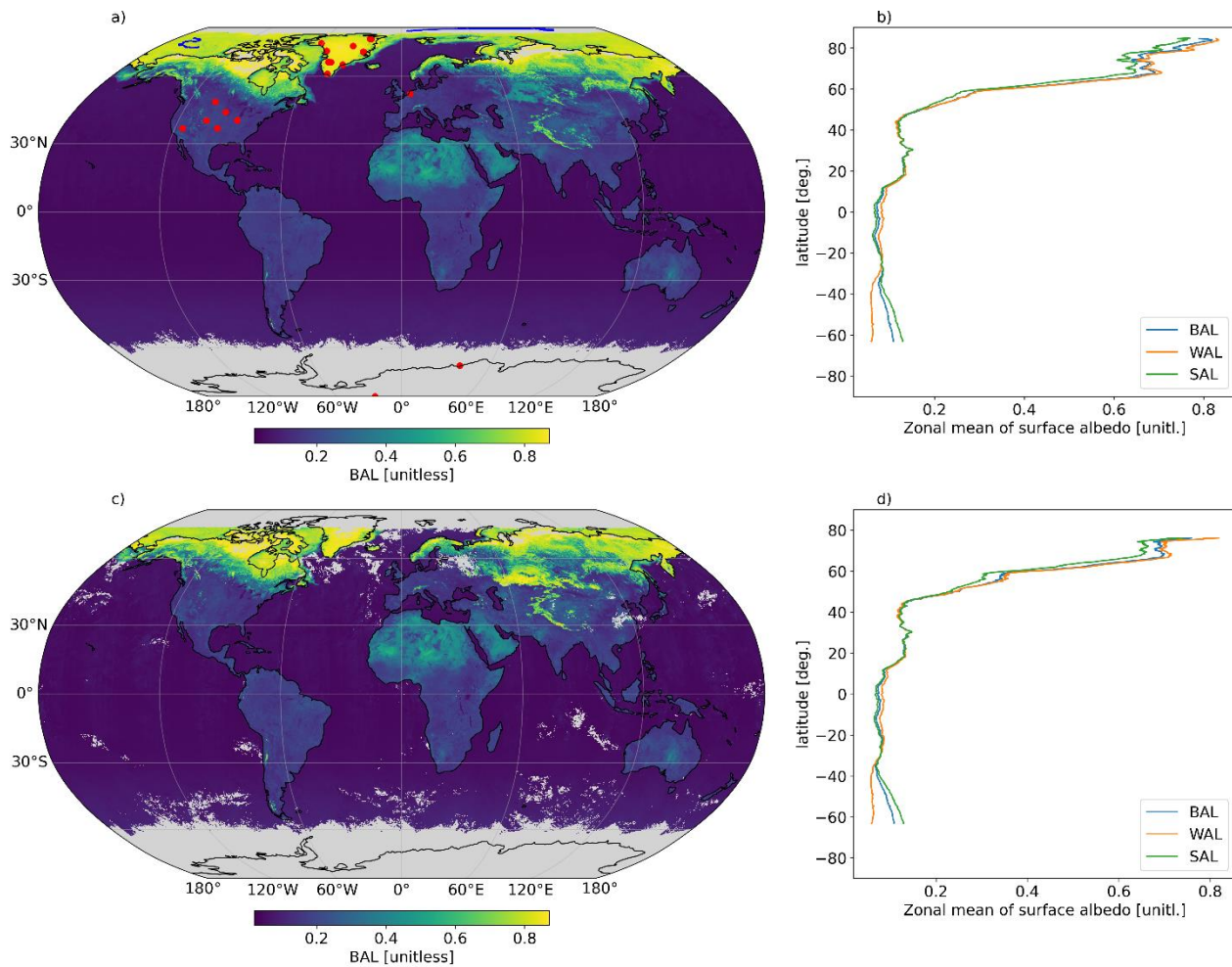
Figure 1: (a) an example of the monthly mean blue-sky (BAL) surface albedo from April 2015. (b) the zonal means of the blue-sky (BAL, blue, thick), white-sky (WAL, orange), and black-sky (SAL, green) surface albedo. Subplots c) and d) show the same visualizations for the pentad mean starting April 1, 2015. Red circles in subplot a) further show the validation sites used in this study, and blue lines show the drift tracks of the SHEBA and Tara ice camps across the Arctic Ocean during the validation periods.
