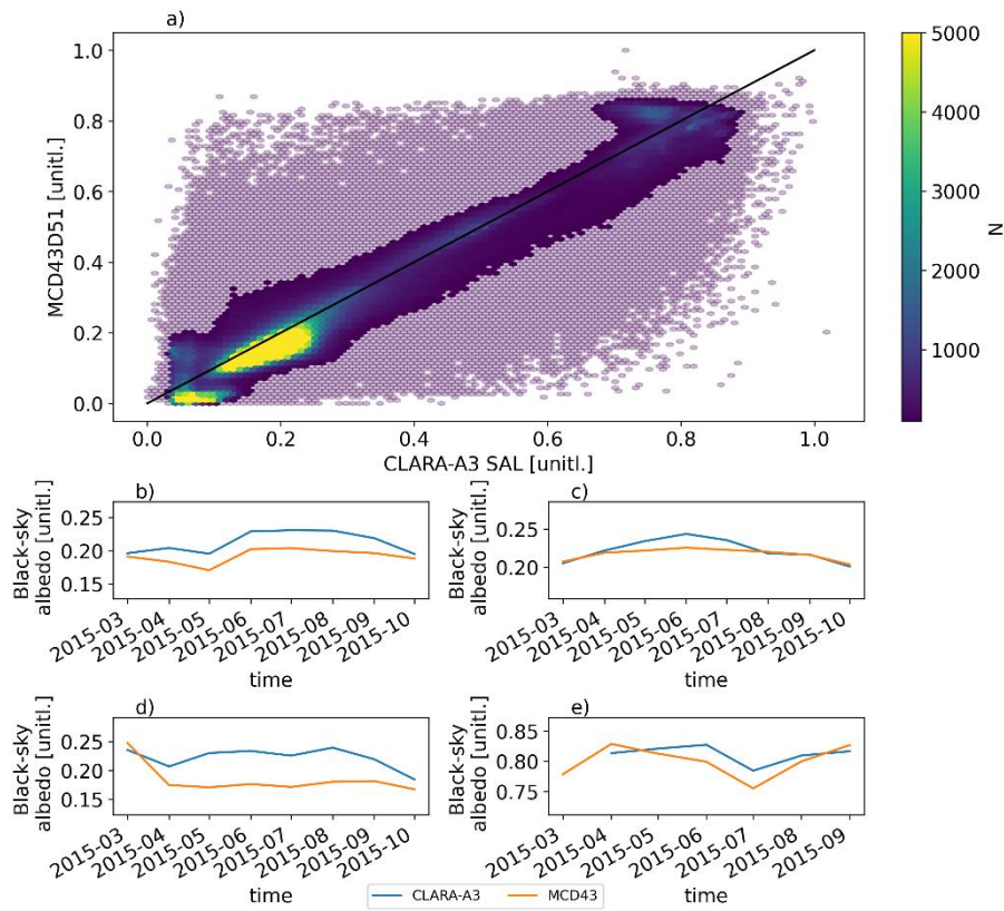
Figure 12: a) Density-colored (semitransparent for N < 100 ) scatter plot of CLARA-A3 SAL monthly mean black-sky albedo (x-axis) versus MCD43D51 (y-axis) during March-October 2015, and time series representations of monthly mean black-sky albedo retrievals at select BSRN and PROMICE sites, b) E13, c) DRA, d) BOU, and e) CEN (ice sheet).
