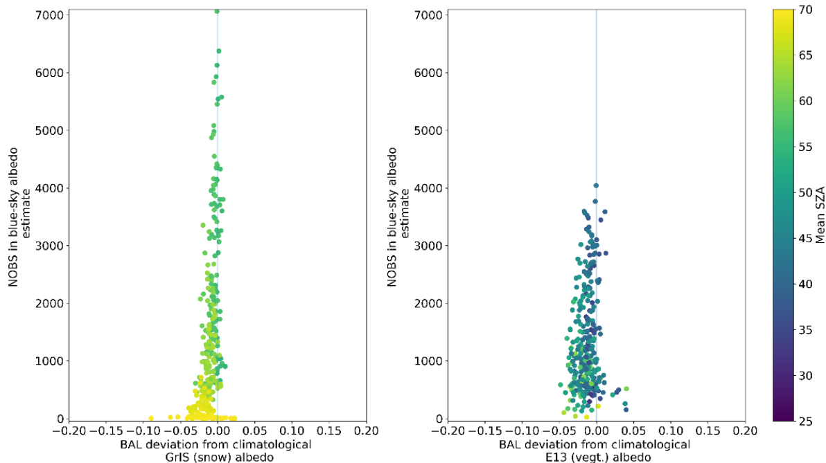
270 Figure 5: (a) Deviation of monthly mean BAL from climatologically expected surface albedos over central GrIS and the Kansas plains containing the E13 BSRN site (b) as a function of sampling count and mean SZA (marker color).
