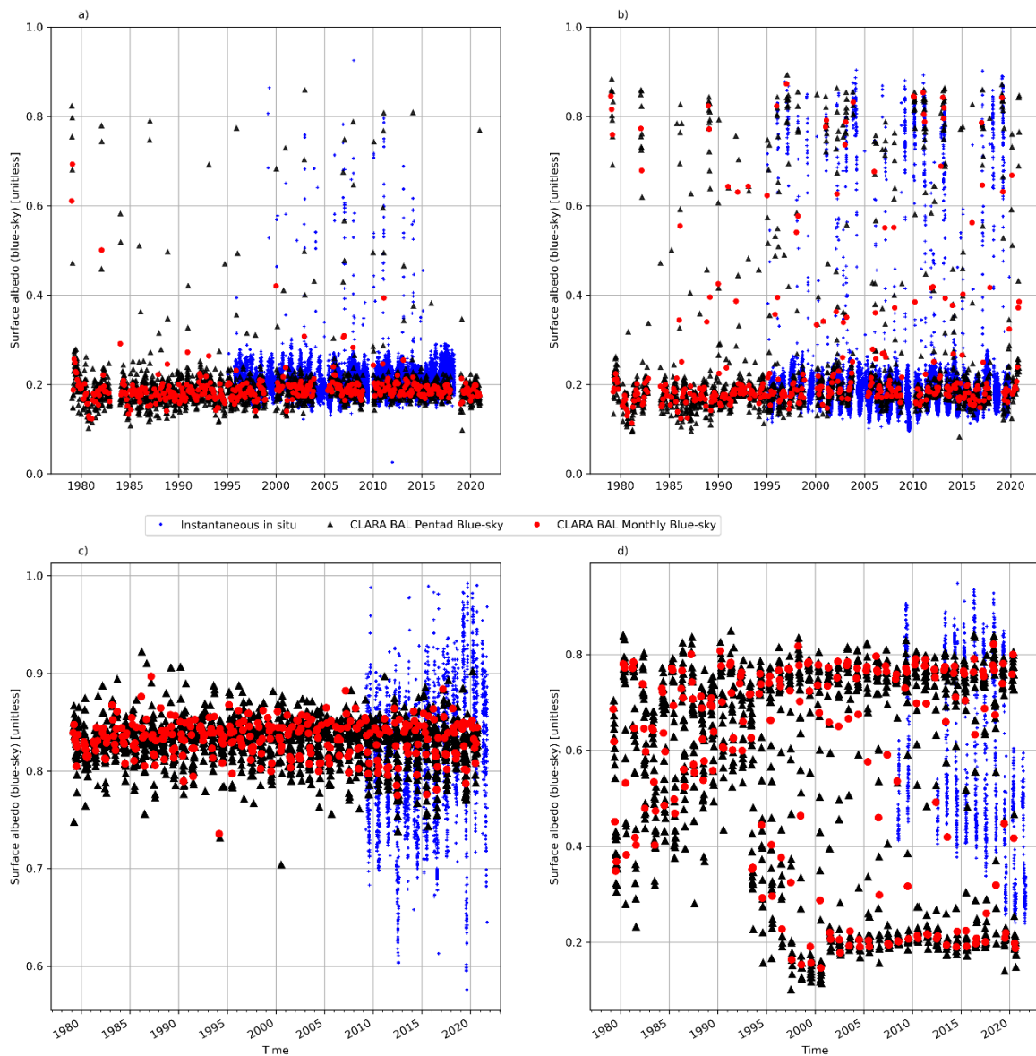
410 Figure 8: Retrieved CLARA-A3 monthly means (red circles) and pentad means (black triangles) of blue-sky surface albedo (BAL) over BSRN site E13 (a) and FPE (b), as well as PROMICE ice sheet sites KAN U (c) and KPC L (d). Blue markers indicate in situ-measured blue-sky albedos at sub-daily (BSRN) or daily (PROMICE) resolutions.
