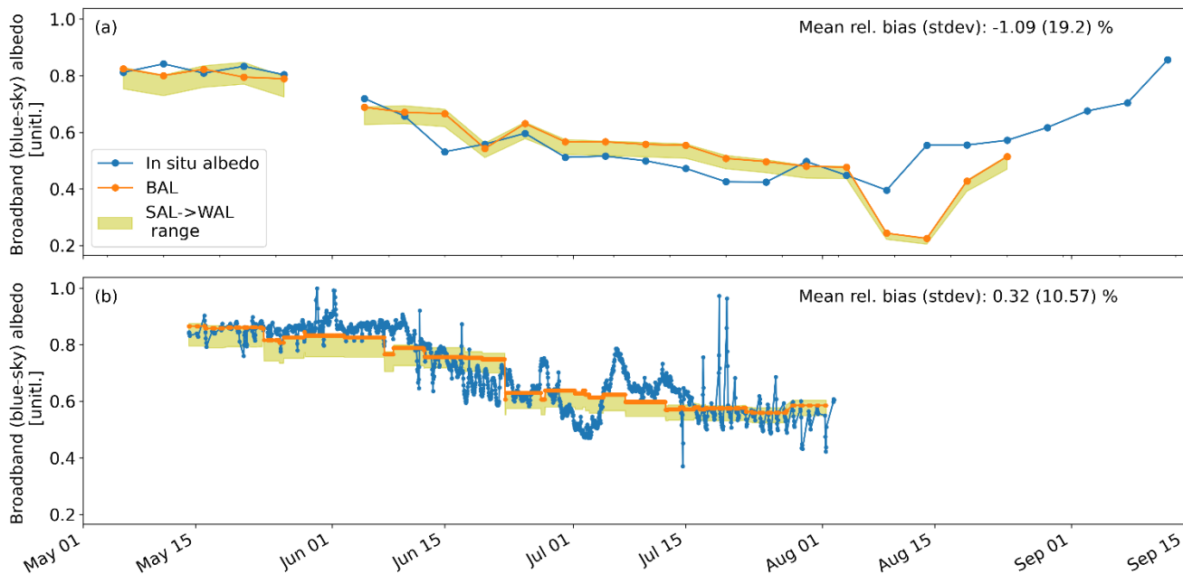
Figure 109: In situ measured surface albedo of Arctic sea ice (blue) and the corresponding grid cell scale 5-day CLARA-A3 estimates (orange) for the (a) SHEBA expedition during summer 1998, and (b) for the Tara-Arctic expedition during summer 2007. The yellow shading illustrates the range between the associated grid cell's black-sky and white-sky CLARA albedo estimates for each sampled period.
