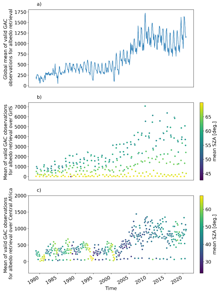
Figure 4: (a) The global mean of valid clear-sky GAC-resolution AVHRR observations (NOBS) in monthly mean SAL. (b) The mean amount of valid observations over a small region in the central part of the Greenland Ice Sheet (72-74° N, 39-41° W). (c) The mean amount of valid observations over a region in the central part of Africa (-2 – 0° N, 18-20° E). Each marker represents a monthly mean, color-coded by the mean Sun Zenith Angle (SZA) of the observations.
