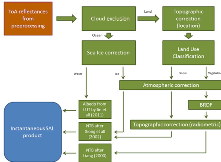
Figure 2: Flowchart of level 2 processing for black-sky albedo (SAL) in CLARA-A3.
