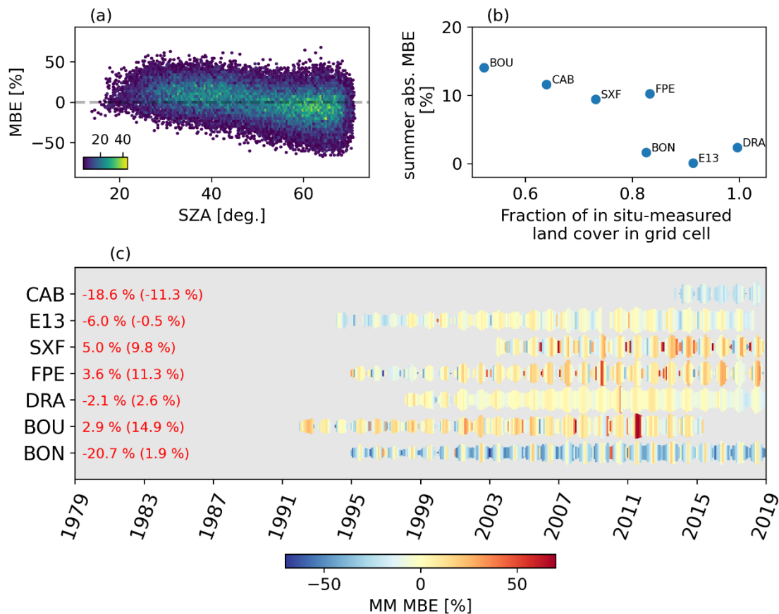
Figure 6: (a) Relative retrieval error (MBE) as a function of SZA for all tracked level 2 snow-free blue-sky albedo (BAL) estimates over the representative land surface BSRN sites (N=93620). Outliers with <5 occurrences are omitted for clarity. (b) Mean absolute MBE of summer (JJA) CLARA level 3 (i.e. 0.25 degree resolution) data as a function of fraction of land cover in the CLARA grid cell which matches the land cover being measured at the BSRN site. (c) Monthly mean MBE over the representative BSRN sites through time. Sizes-The heights of the colored rectangular markers indicate the amount of valid clear-sky AVHRR data of each month. Text in red shows annual mean MBE (summer MBE).
