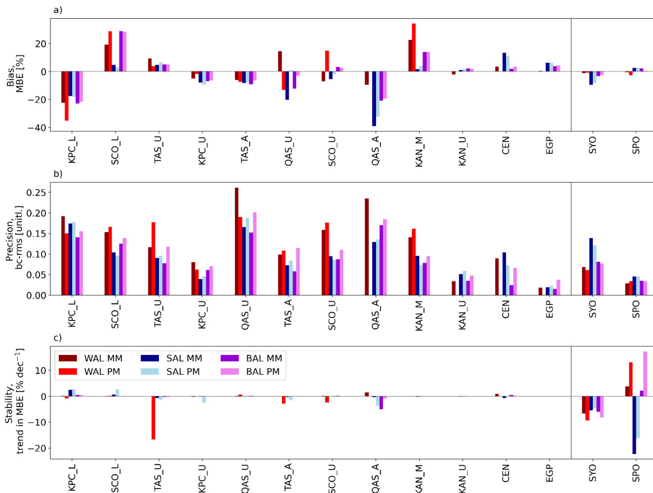
Figure 98: Bias (MBE; panel a), precision (bc-rms; panel b) and stability (decadal trend in MBE; panel c) of the CLARA-A3 pentad and monthly mean albedo estimates over the PROMICE and BSRN snow/ice sites. Red for WAL, blue for SAL, and violet for BAL. Dark colors indicate monthly means and light colors pentad means. Sites with less than 90% snow/ice cover in their CLARA grid cell are shown as partially transparent. SAL stability for EGP is not shown due to a very low number of available samples. The vertical grey line separates PROMICE and BSRN sites.
