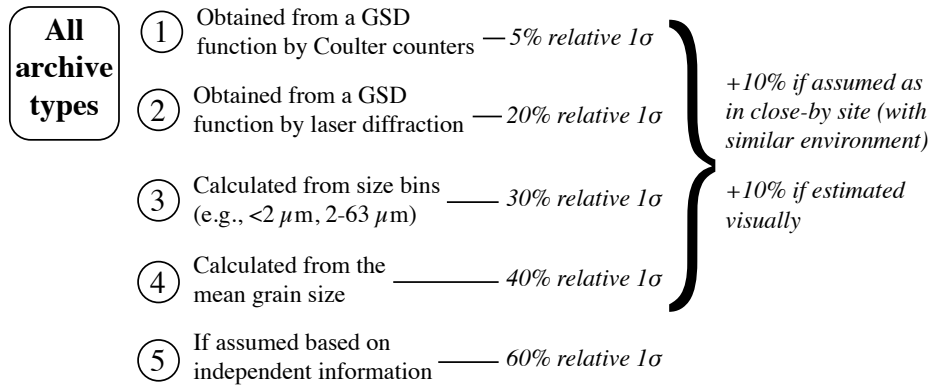
Figure 3: Criteria for assigning uncertainty to the <10\text{-}\mu\text{m} grain size fraction. GSD: grain size distribution.
