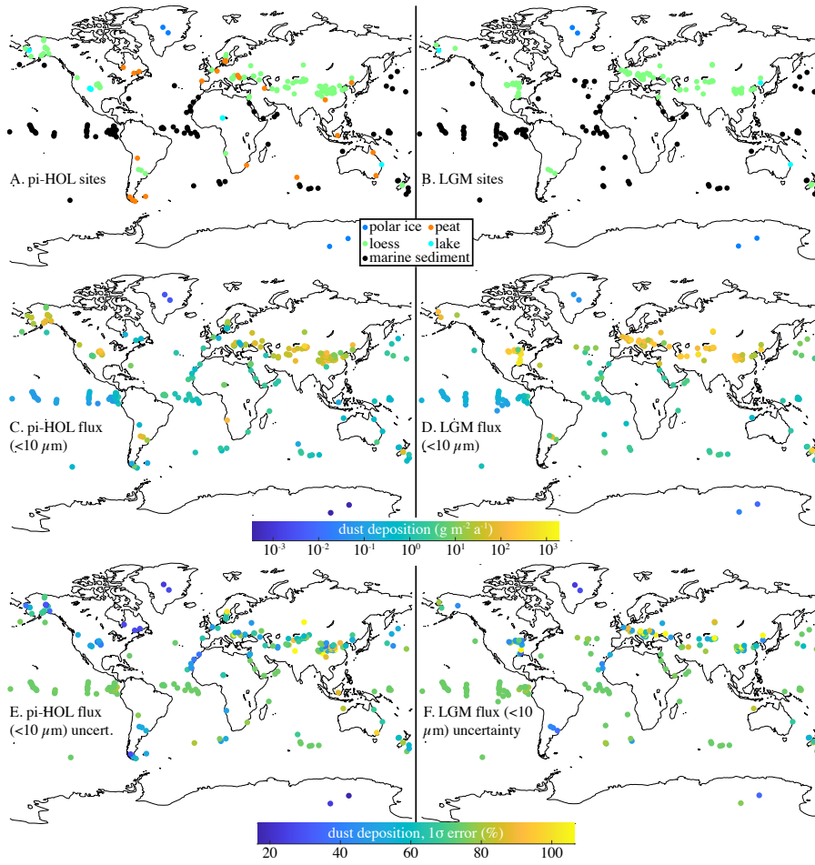
085 Figure 5: Distribution of sites for the (a) pre-industrial Holocene (pi-HOL) and (b) Last Glacial Maximum (LGM) time periods, (c) pi-HOL and (d) LGM <math><10\text{-}\mu\text{m}</math> dust deposition rate, and (e) pi-HOL and (f) LGM <math><10\text{-}\mu\text{m}</math> dust deposition rate uncertainty. The coastlines for all panels correspond to those of the present day.
