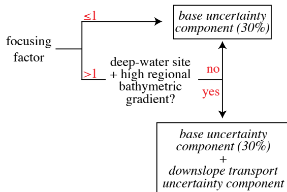
1075 Figure 4: Criteria for assigning uncertainty to the sediment bulk mass accumulation rate when using the ^{230}\text{Th} normalization technique for deriving dust fluxes from marine sediment cores.
