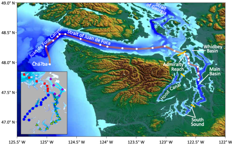
Figure 1: Map of the southern Salish Sea and its boundary waters with all study basins named. The subset of sampling stations tracing a path between the Chá7ba mooring on the Washington state (USA) continental shelf and the Main Basin of Puget Sound constitute the Sound-to-Sea (S2S) transects. Inset map shows station groupings used for analyses of Puget Sound cruises: Admiralty Reach (AR, red squares), Main Basin–South Sound (MB–SS, green triangles), Whidbey Basin (WB, purple diamonds), and Hood Canal (HC, blue circles). Yellow dashes in the main figure denote locations of glacial sills. Topographic and bathymetric data were extracted from the NOAA National Centers for Environmental Information Grid Extract Coastal Relief Model (3-second resolution, https://www.ncei.noaa.gov/maps/grid-extract/ , accessed Nov. 13, 2014). Data were gridded in Surfer using a minimum curve gridding technique.
