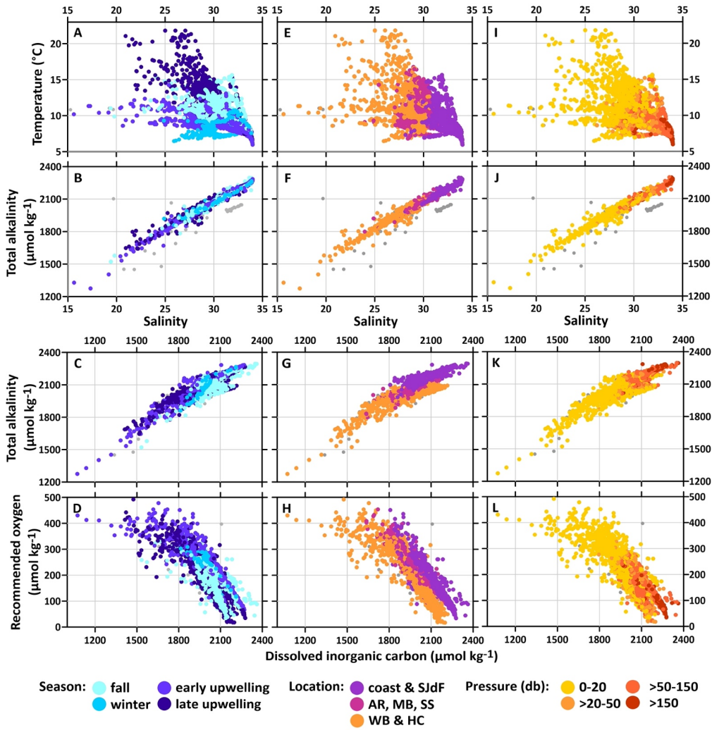
Figure 3: Property-property plots of oceanographic parameters used to delineate spatial, seasonal, and depth variability: salinity (CTDSAL_PSS78) vs. temperature (CTDTMP_DEG_C_ITS90) by season (A), location (E), and pressure (~depth, I); salinity vs. total
