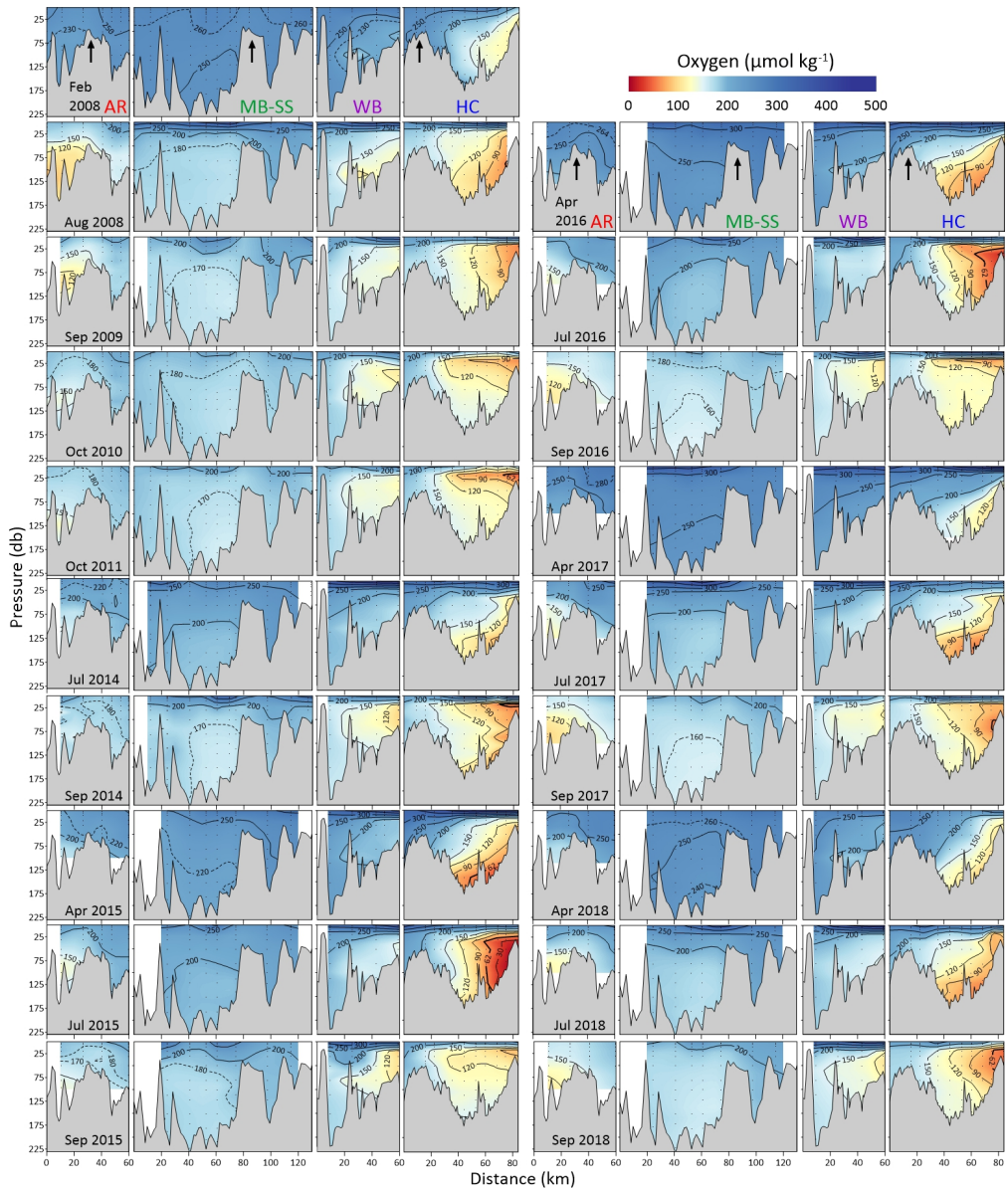
625 Figure 9: Depth transect plots from all Puget Sound cruises for adjusted CTD oxygen content ( O_2 , \mu\text{mol kg}^{-1} ). The bold contour at 62 \mu\text{mol kg}^{-1} represents a commonly used hypoxia threshold. Figure organization is the same as in Figure 5.
