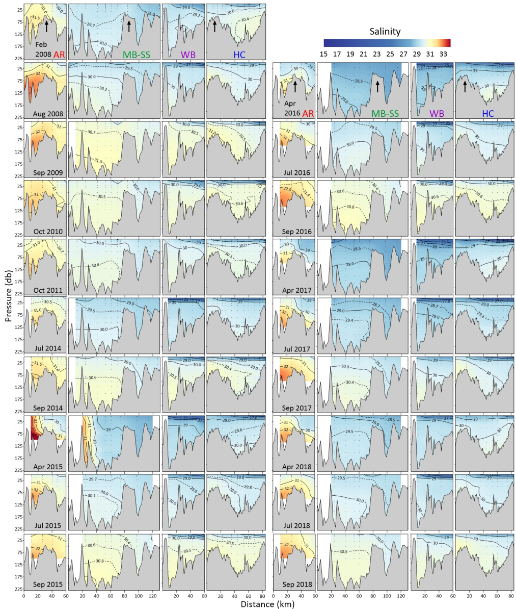
615 Figure 6: Depth transect plots from all Puget Sound cruises for salinity. Figure organization is the same as in Figure 5.
