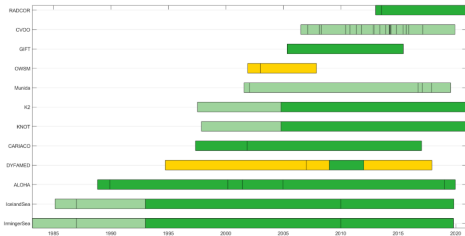
Figure 4: Time-dependency of assigned SOP flag of each time-series program exemplarily shown for nitrate. Vertical black lines indicate method changes, captured and non-captured (e.g. instrument change) by the SOP flags. The color scheme used,
