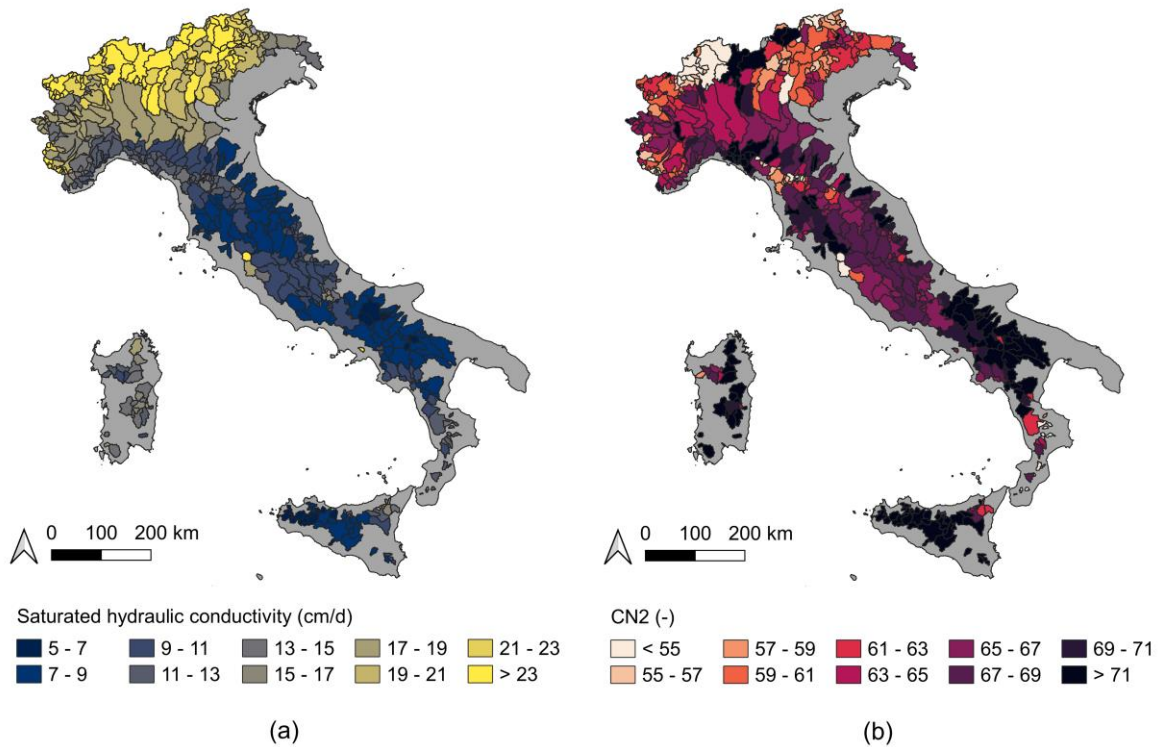
300 Figure 4. Mean areal values of the saturated hydraulic conductivity (a) and the Curve Number in average conditions, i.e. CN2 (b). Administrative boundaries: GADM v3.6.
