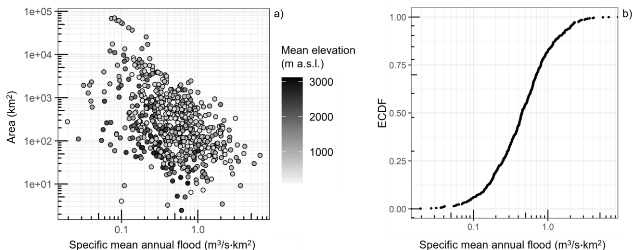
450 Figure 10. Relation among area, specific peak discharge and mean elevation of the catchments (a) and empirical cumulative distribution function (ECDF) of the specific mean annual flood (b).
