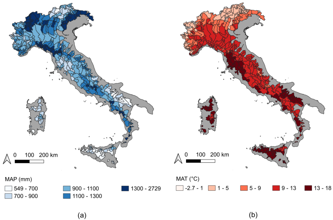
350 Figure 6. Spatial representation of the mean annual precipitation (a) and mean annual temperature (b). Administrative boundaries: GADM v3.6.
