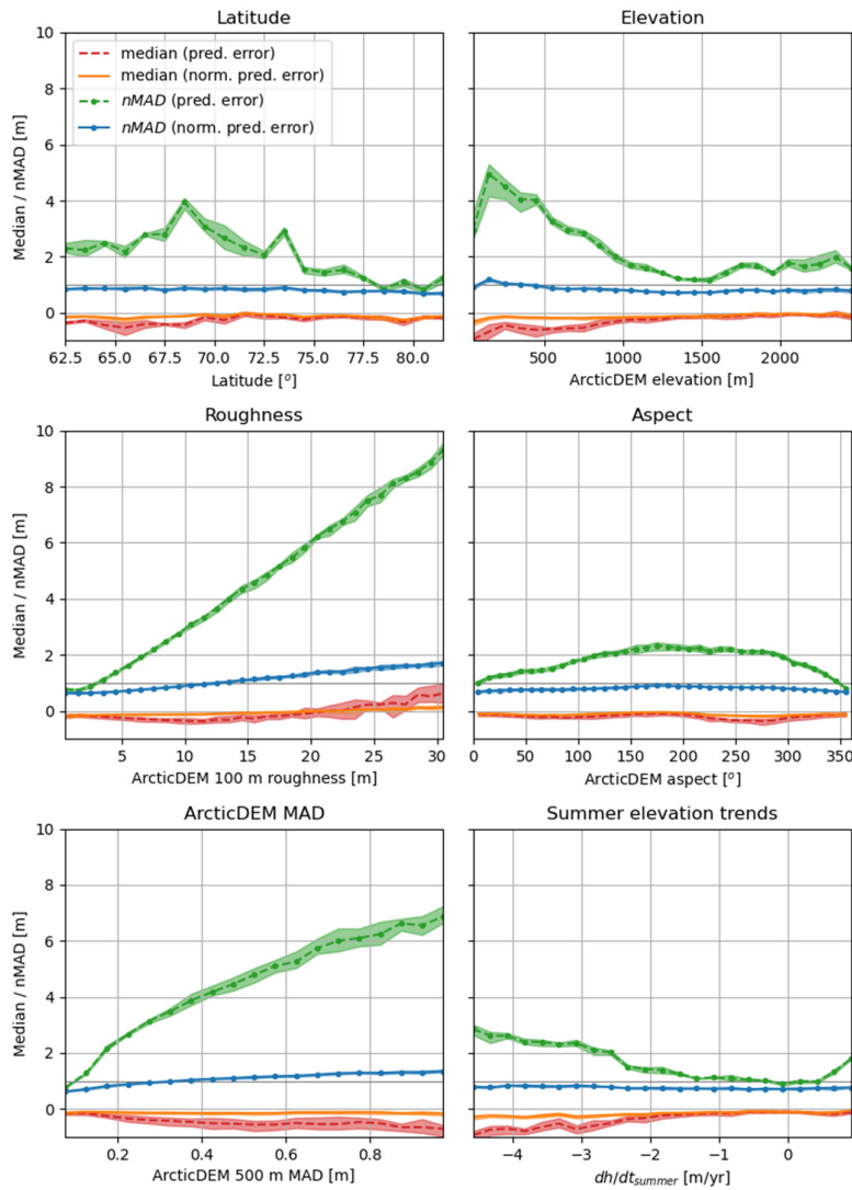
685 Figure 11: Descriptive measures (median and nMAD) of the distribution of PRODEM19 raw (dashed lines) and normalized prediction errors (solid lines), when stratified relative to various location and terrain properties that may impact the PRODEM product performance. Lines correspond to mean values over the four-year PRODEM series, with the envelope showing minimum and maximum values for the four years. Bins are created to cover the 5 to 95 percentiles of each data set. The ArcticDEM MAD value is the median absolute deviation of the DEMs contributing to ArcticDEM at a given location, thereby providing an elevation uncertainty estimate. Summer elevation trends from Slater et al (Slater et al., 2021a). 690
