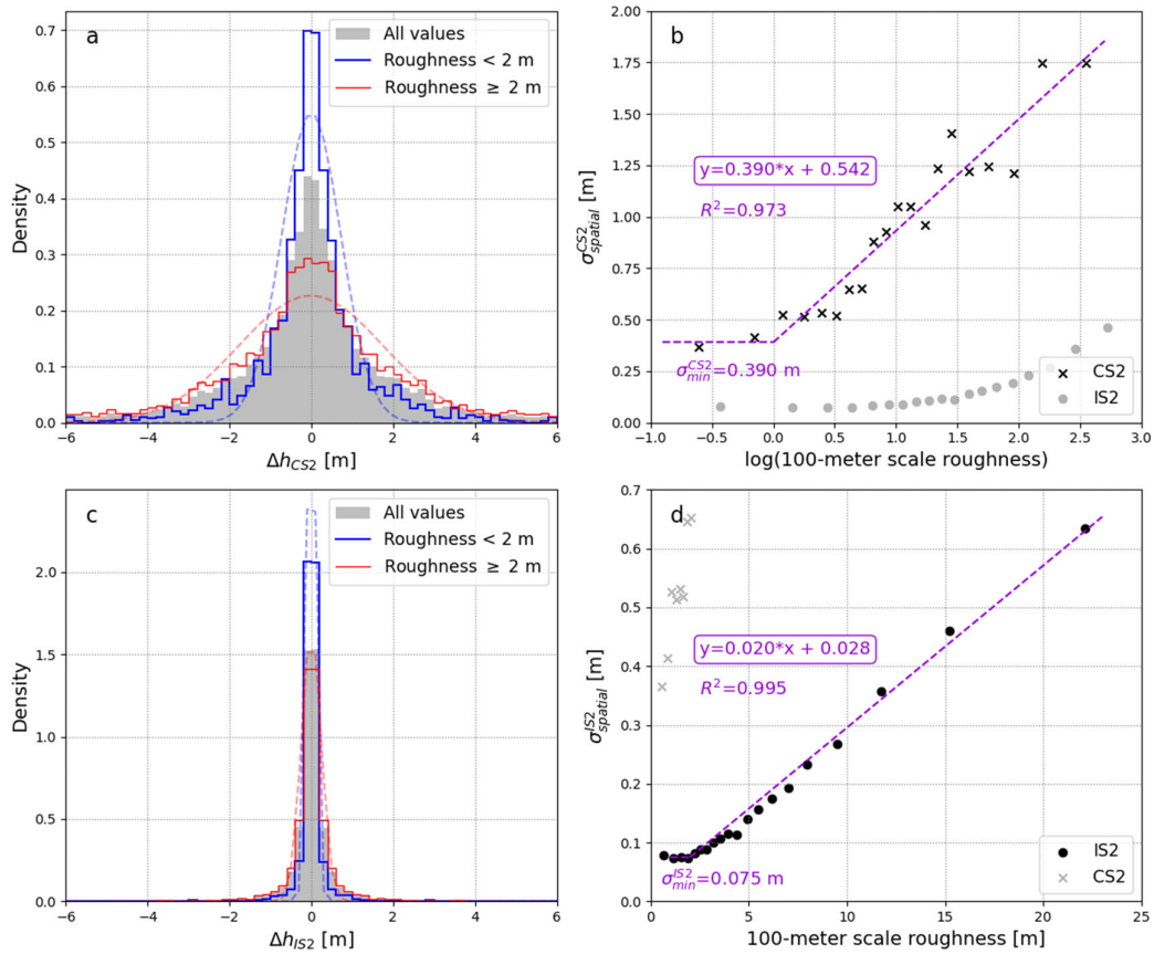
260 Figure 2: a, c) Distribution of measured elevation differences ( \Delta h ) close to CS2 (a) and IS2 (c) intersecting satellite tracks within the 265 entire study area (grey), and from intersecting tracks in areas with roughness higher (red) or lower (blue) than 2 m, respectively. Dashed lines are approximate normal distributions based on calculated median and nMAD. Only data from temporally close acquisitions is included. b, d) For CS2 (b), a linear relationship (dashed violet line) exists between the logarithm to the local 100m- scale roughness and the estimated spatial uncertainty based on the dispersion of associated elevation differences (Eq. 1). For IS2 (d), on the other hand, we observe a linear correlation directly between the roughness and estimated spatial uncertainty. To ease the comparison between the derived CS2 and IS2 uncertainties, data from the other satellite is included in b and d (light grey). All uncertainty models are based on data from the summers of 2019 through 2022.
