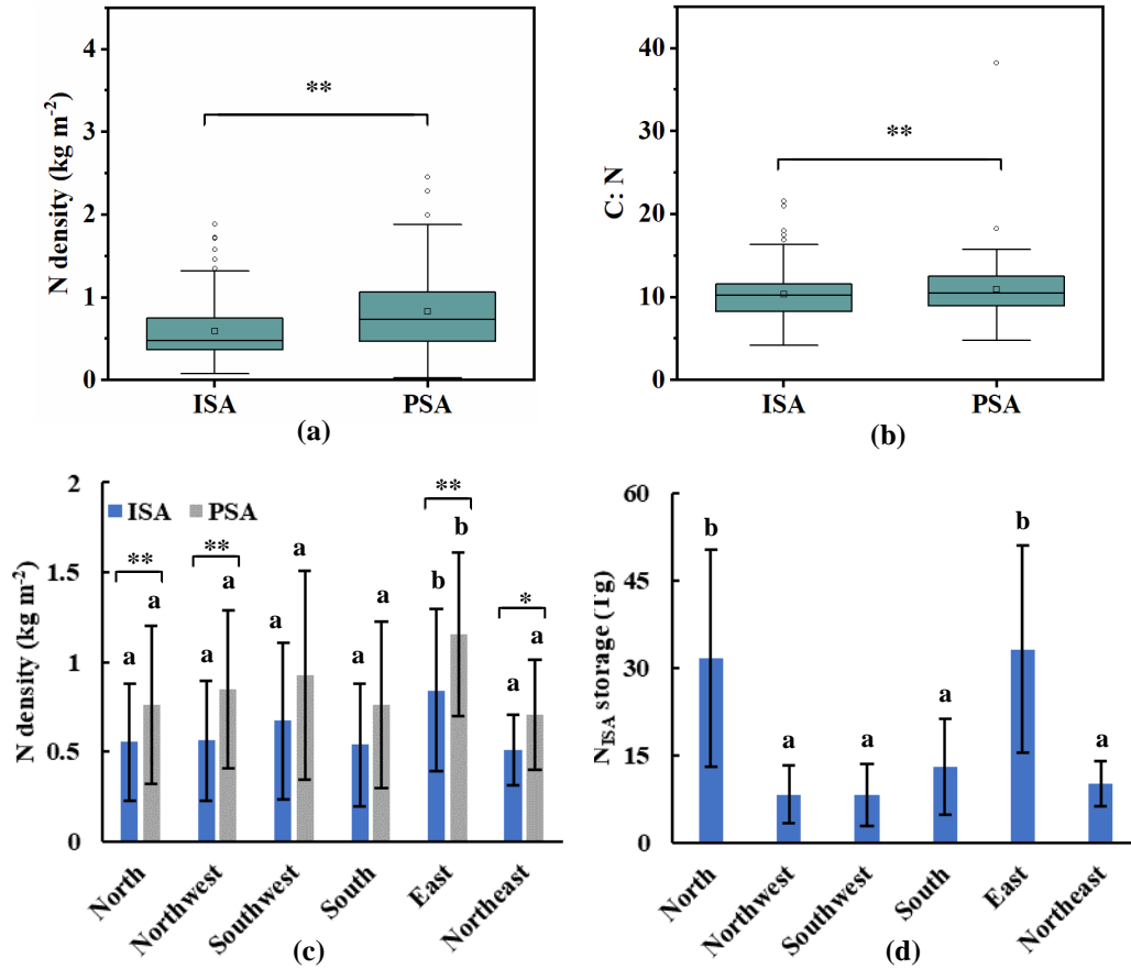
Figure 3: The N density, N storage and C:N ratio of the ISA in China. The soil N density and C:N in the ISA and the reference PSA are compared in (a) and (b), respectively. The square box shows median and quad values, the inner small rectangle is the mean value. The regional mean N_{ISA} density and N_{PSA} density in different subregions are compared in (c). The regional N_{ISA} storage of different subregions are compared in (d). The letters indicate the significance of the difference among the subregions. * and ** indicate significant differences between ISA and PSA, p < 0.05 and p < 0.01 , respectively.
