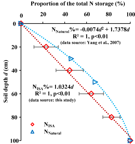
275 Figure 6: Comparing the vertical distribution pattern of N between the sealed soil ( N_{ISA} ) and the natural soil ( N_{Natural} ) in China (refer to Section 2.4 Equation 4).
