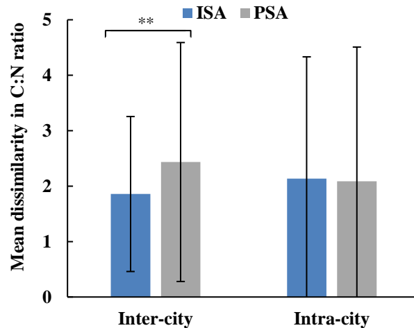
250 Figure 4: Comparing the inter–city variation and the intra–city variation of C:N ratios between the ISA and PSA. The variations were measured by the dissimilarity of (or the Euclidean distance between) paired observations. For intra–city variation, the soil C:N dissimilarity between each pair of different sampling sites within the same city were calculated and averaged; for inter-city variation, the soil C:N dissimilarity between each pair of different cities under investigation were calculated and averaged. ** 255 indicate significant differences between ISA and PSA ( p < 0.01 ).
