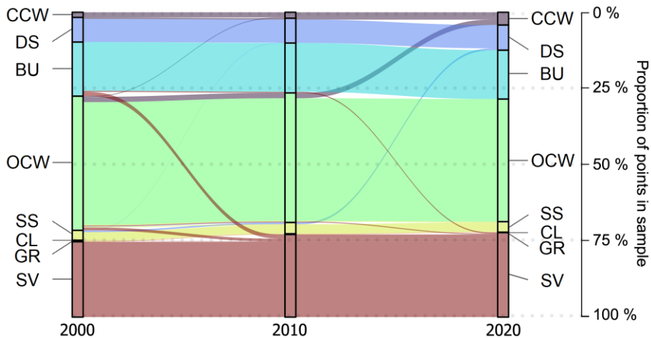
Figure 13: Decadal vegetation transition between 2000-2020 of 48,280 random pixels with potentially valid land cover transitions as defined in our state transition model for the three selected years. Land cover classes are presented in Table 1. Color codes were assigned to land cover classes present in the locations in year 2020 in order to track changes between decades.
