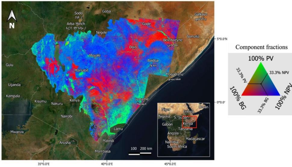
Figure 16: Landsat derived 30 m resolution fractional cover estimations for the short dry season of 2020, with mixtures of PV: Photosynthetic vegetation, NPV: non-photosynthetic vegetation, and BG: bare ground for our entire AOI (see legend on figure). Basemap: ©MapTiler, https://www.maptiler.com/copyright/ .
