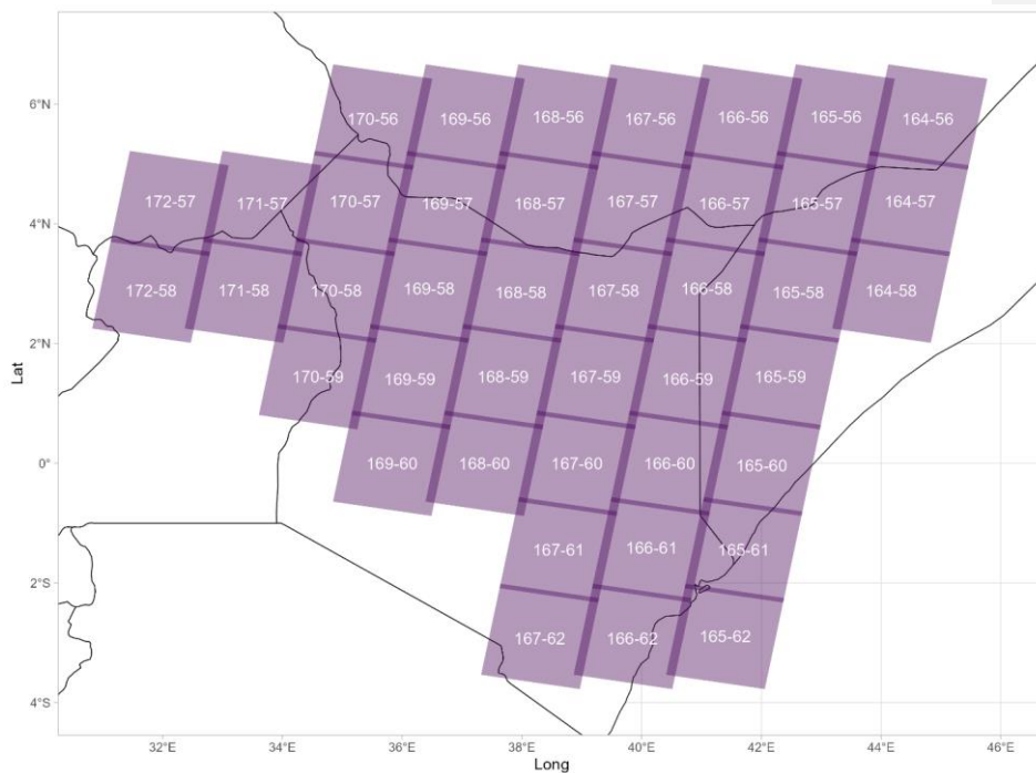
Figure 4: Spatial coverage of Landsat tiles used in this study spanning from 2000-2022. Numbers within each tile correspond to the PATH and ROW used in the Landsat data storage protocol.
