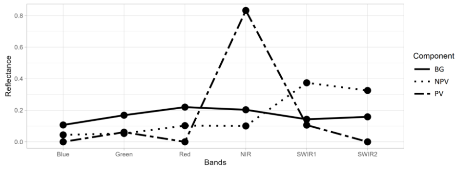
790 Figure 14: Estimated spectral endmembers for fractional cover estimation.
