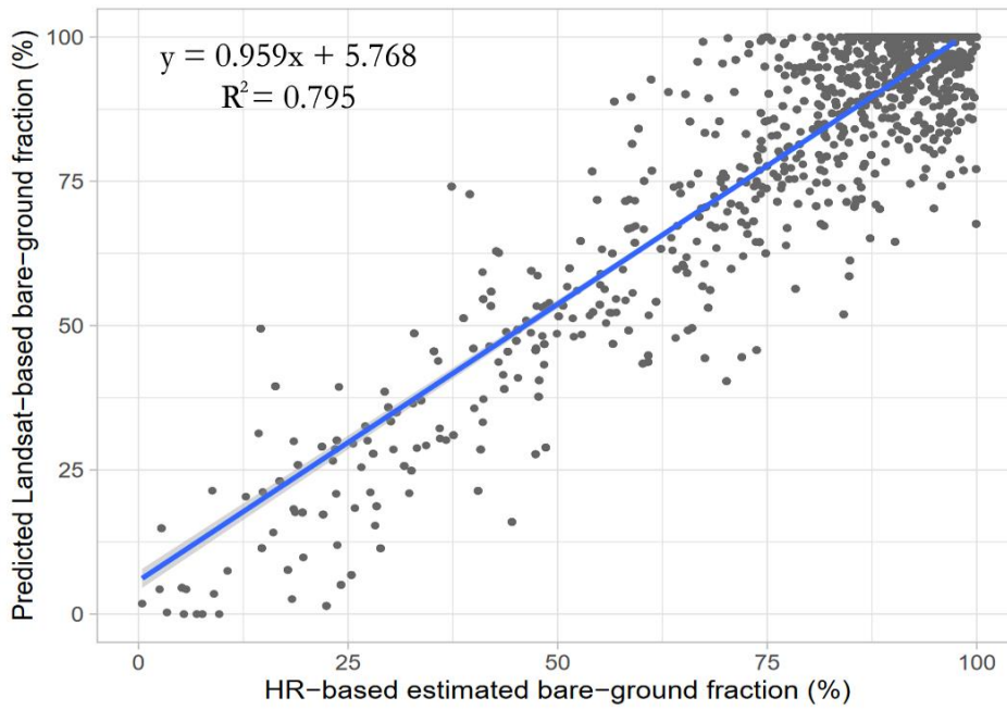
795 Figure 15: Spatial-temporal correlation between HR imagery and Landsat-based predictions of bare ground fractional cover (n = 2,190) at Landsat scale of 30 m from 2016 to 2020. F = 9,201.1 on 1 and 2152 DF with p-value: < 2.2e-16.
