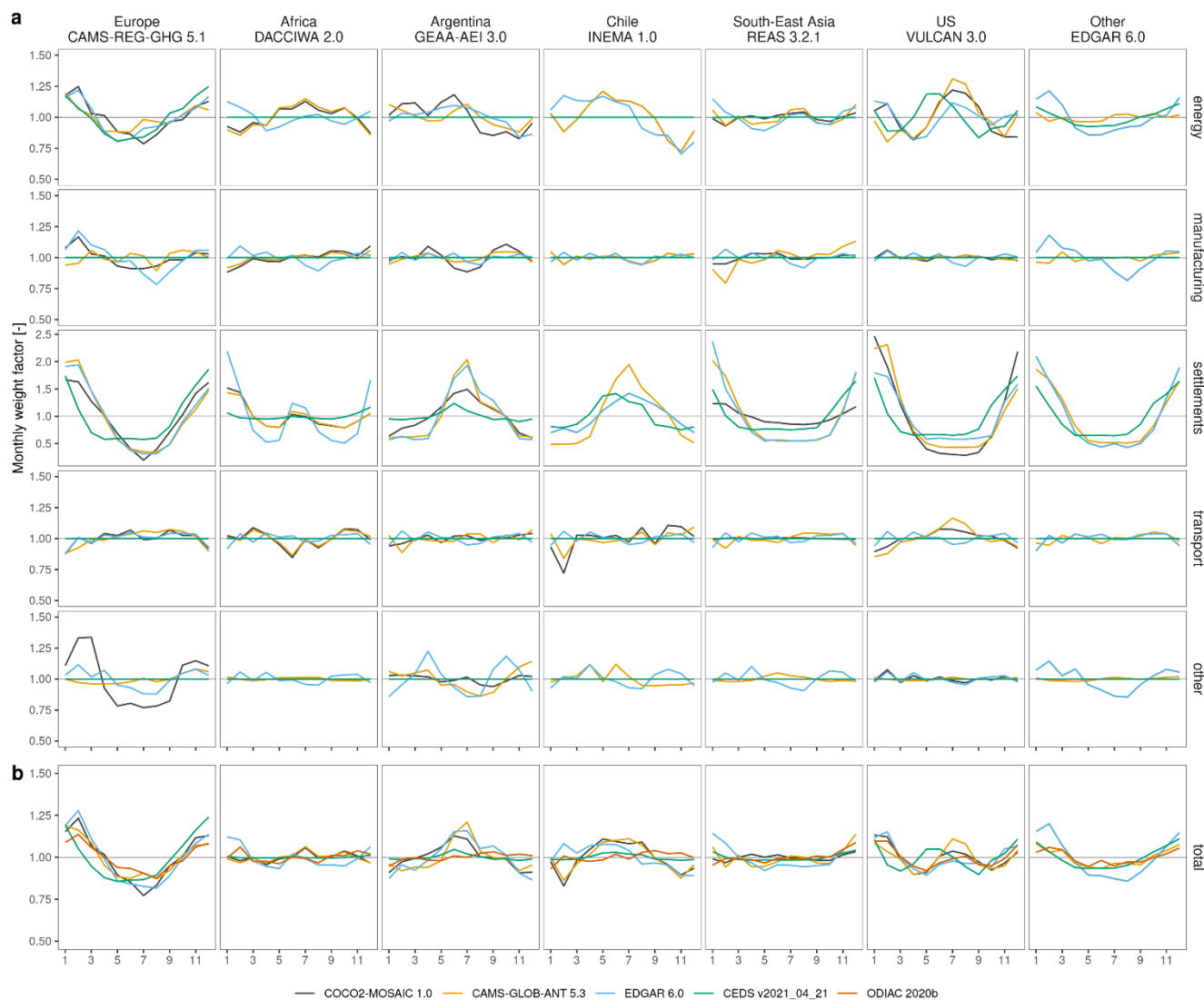
Figure 4 Monthly CO 2 ff weight factors per sector and region in 2015. Factors are calculated with the total monthly emissions per region and sector (monthly weight factor = total monthly emissions per region / total annual emissions per region). Note that the settlement sector has a different scale due to its larger seasonality.
