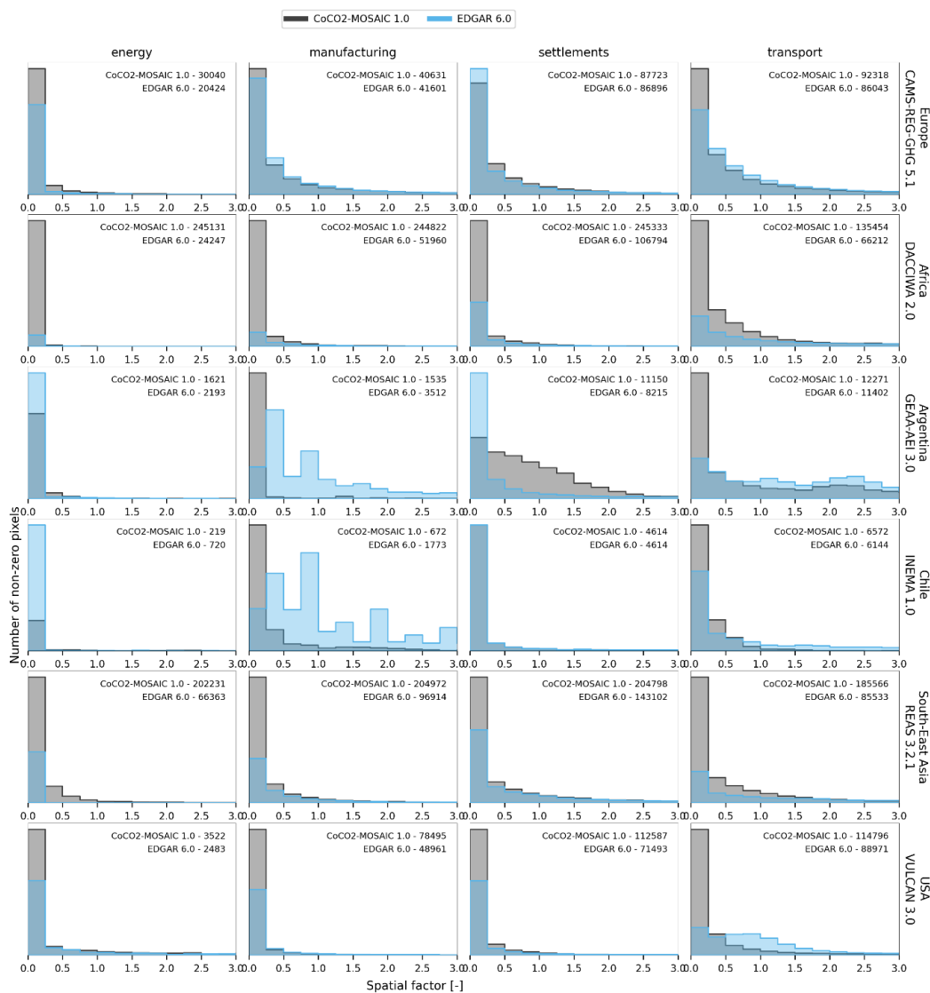
420 Figure 5 Histogram of annual CO 2 ff spatial weight factors (pixel emission flux / average emission flux in the region) during 2015 per region and sector. The annotation shows the number of pixels with non-zero emissions. Pixels with zero emissions are excluded from the histograms.
