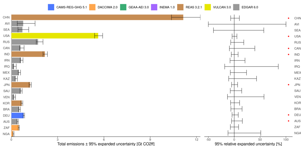
540 Figure 8 Total emissions \pm 95% expanded uncertainty and 95% relative expanded uncertainty of CoCO 2 -MOSAIC 1.0 CO 2 ff emissions in the 20 countries with the largest absolute uncertainty. Countries are ranked top down according to their absolute uncertainty. Red points indicate countries with a well-developed statistical system (WDS).
