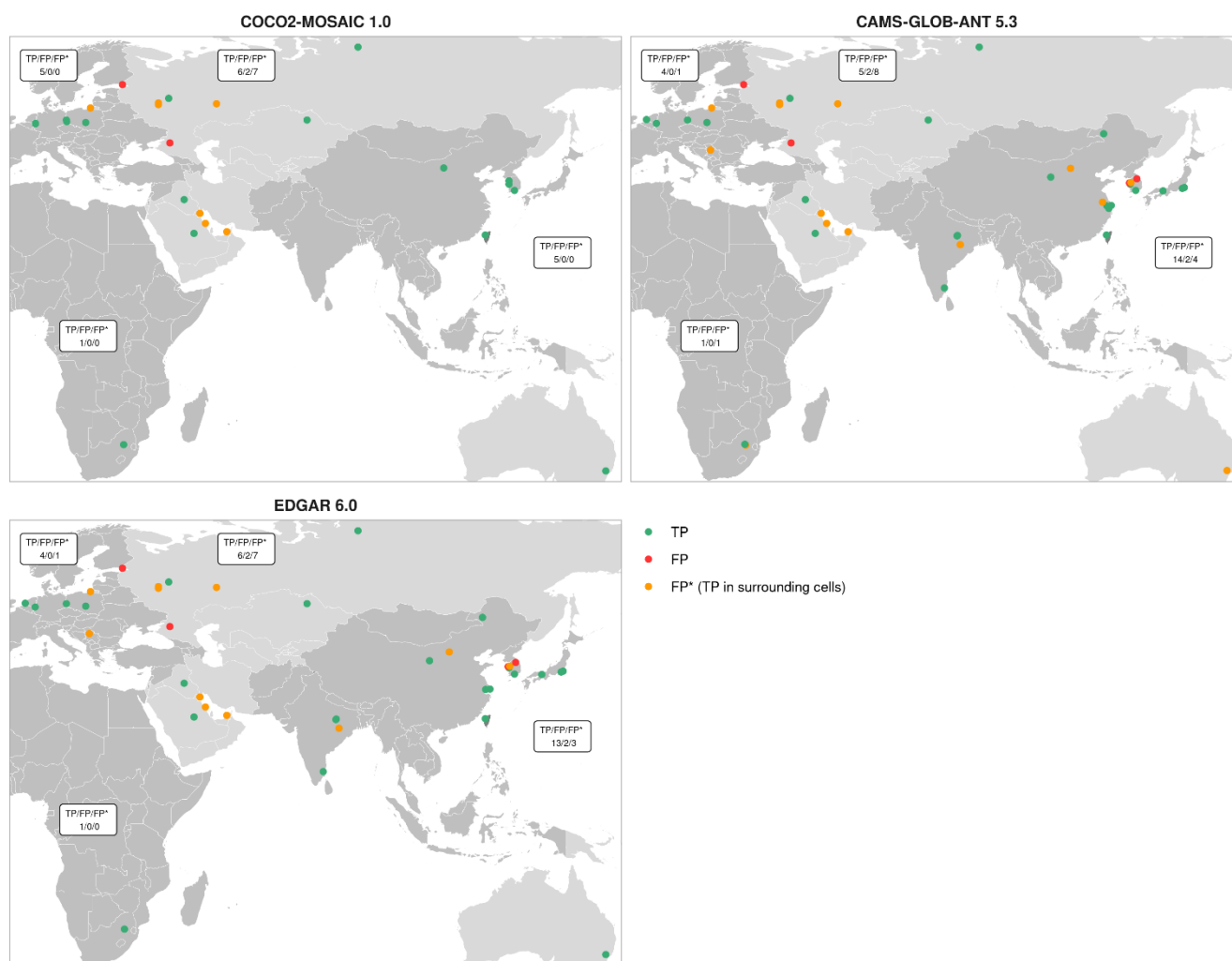
480 Figure 6 Comparison of the location of super-emitting pixels from global inventories (test datasets) against the CoCO2 1.0 power plant database (reference dataset). TP = true positive, FP = false positive, FP* = false positive, with a TP in the surrounding pixels.
