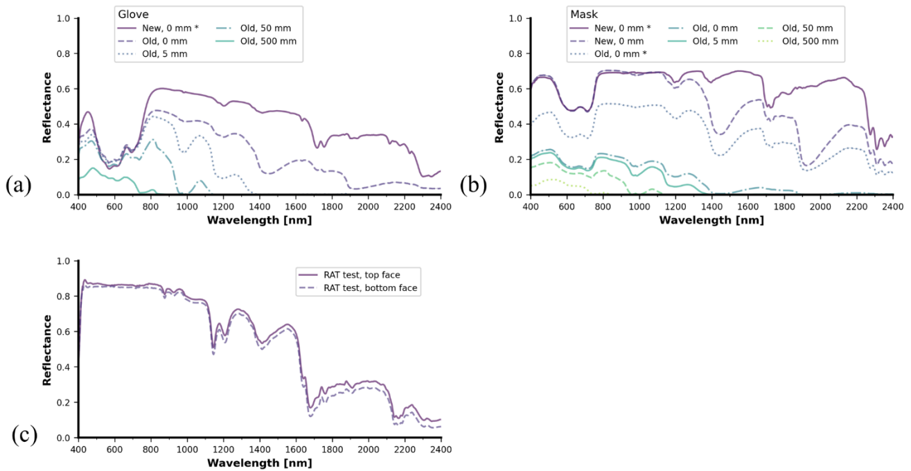
285 Figure 13 Spectral reflectance data from COVID-19-related medical waste in varying conditions: old and new surgical gloves from 0 to 500 mm depth (a), old and new medical masks from 0 to 500 mm depth (b), Rapid Antigen Tests (RAT)(c). For medical masks and gloves, the * denotes that a sample was dry or fully drained after submersion. Note that this study only examines one type of medical gloves and one type of medical mask.
