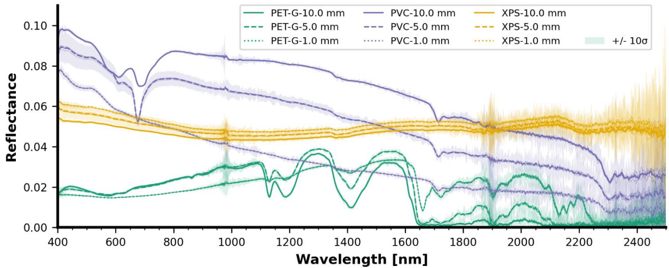
240 Figure 9 Surface-level spectral reflectance of PET-G, PVC and XPS panels with varying thickness. Each curve is the average with the shading representing 10\sigma confidence interval.
