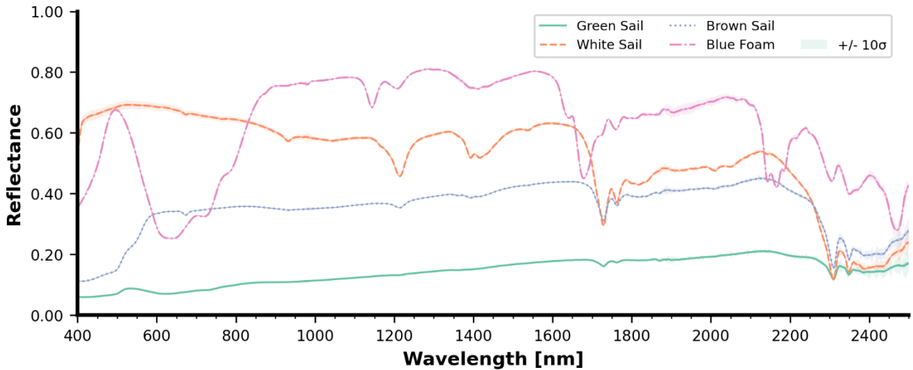
270 Figure 12 Spectral reflectance of dry sailing-related objects, (a): white sail, sample ID 15 in Figure A1. (b): brown sail, sample ID 17 in Figure A1. (c): green sail, sample ID 16 in Figure A1. (d): blue foam, sample ID 14 in Figure A1. Each curve is the average with the shading representing 10\sigma confidence interval.
