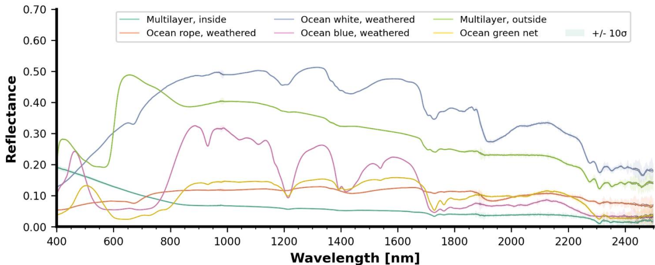
255 Figure 11 Surface-level spectral reflectance of multilayer, blue weathered ocean plastic, white weathered biofouled dried ocean plastic, piece of green ocean net and weathered piece of ocean rope panels with varying thickness. Each curve is the average with the shading representing 10\sigma confidence interval.
