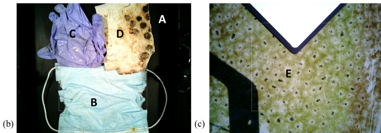
Figure 16 (a) Example spectra, aggregated from the SPECIM IQ hypercube data. For each of the spectral reflectance curves, at least ten points were sampled from the hypercube. The confidence intervals are obtained as the standard deviation of the data points across each sample. (b) The multi-material sample is represented by curves A, B, C, D. (c) Additional 10 mm thickness biofouled PP sample, represented by curve E. Each curve is the average with the shading representing 1\sigma confidence interval.
