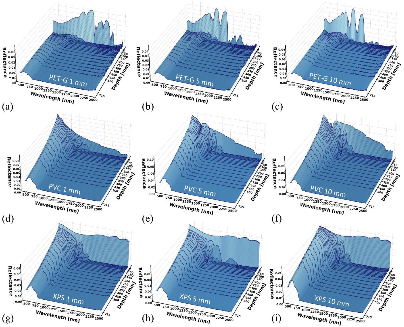
Figure 8 Spectral reflectance at varying depths for (a-c) PET-G, (d-f) PVC, and (g-i) XPS for panel thickness ranging between 1 to 10 mm. Each reflectance curve is the average of five measurements.
