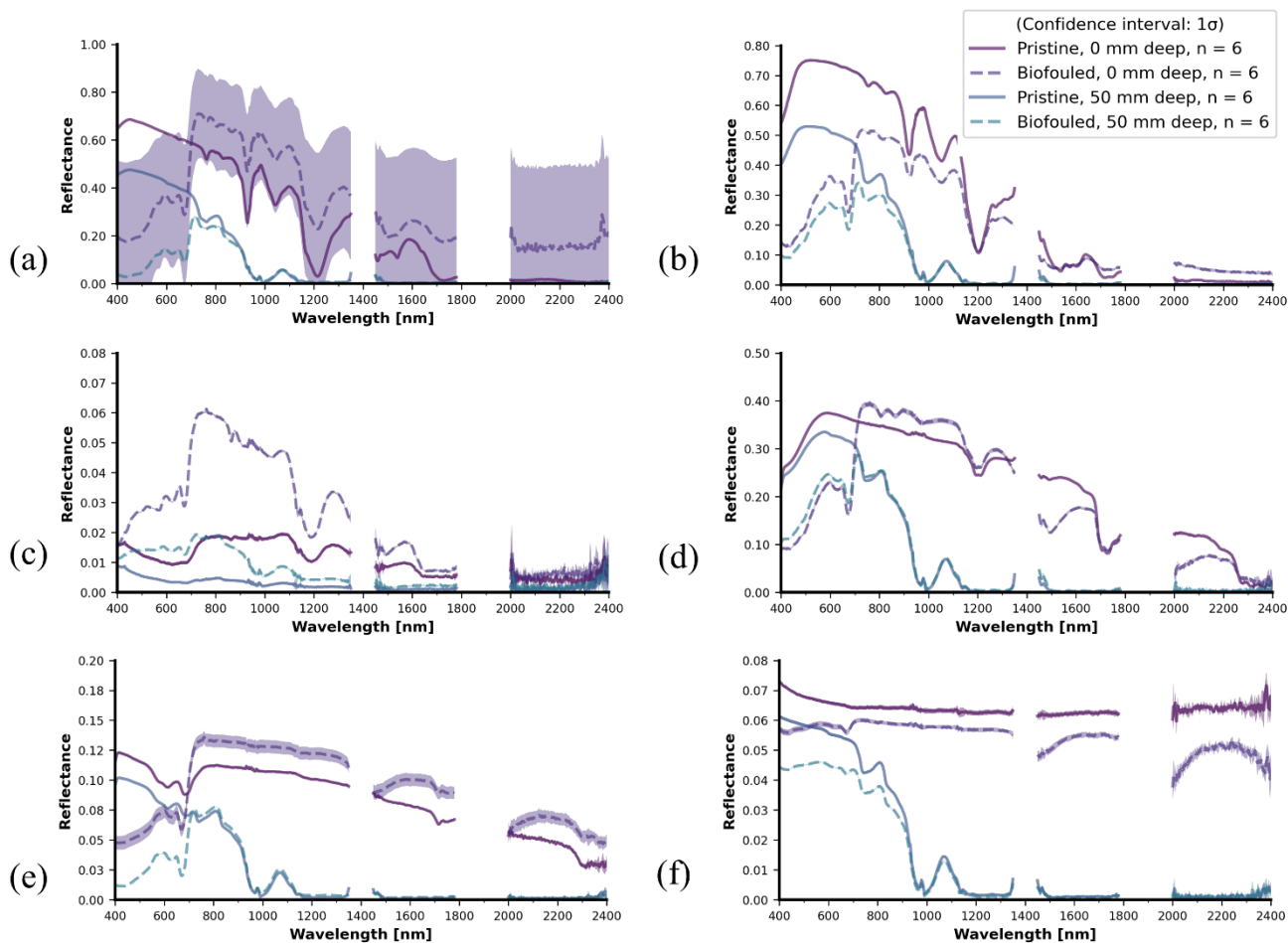
Figure 15 (a) 10 mm thickness HDPE, pristine and biofouled. The main difference occurs in the visible spectrum (400 – 700 nm), which is relatively dark. The biofilm does not obscure any of the typical spectral features; (b) 10 mm thickness PA6, pristine and biofouled. Here, the biofilm generally decreases the spectral reflectance magnitude, with the strongest diminishing effect in the visible (400 – 700) spectrum. Nevertheless, the spectral reflectance shape beyond 700 nm changes minimally; (c) 10 mm thickness PET-G, pristine and biofouled. The reflectance magnitude increases considerably across the entire spectrum for the biofouled sample compared to the pristine sample; (d) 10 mm thickness PP, pristine and biofouled. The main difference occurs in the visible spectrum (400 – 700 nm), which is relatively dark. Spectral features are not influenced by the biofilm; (e) 10 mm thickness PVC, pristine and biofouled. The biofilm mostly decreases the spectral reflectance magnitude in the visible (400 – 700 nm) spectrum. The spectral reflectance shape beyond 700 nm changes minimally; (f) 10 mm thickness XPS, pristine and biofouled. Only minimal differences occur, mainly in the < 700 nm part of the spectrum.
