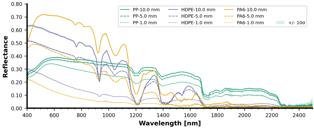
Figure 7 Surface-level spectral reflectance of PP, HDPE and PA6 panels with varying thickness. Each curve is the average with the shading representing 10\sigma confidence interval.
