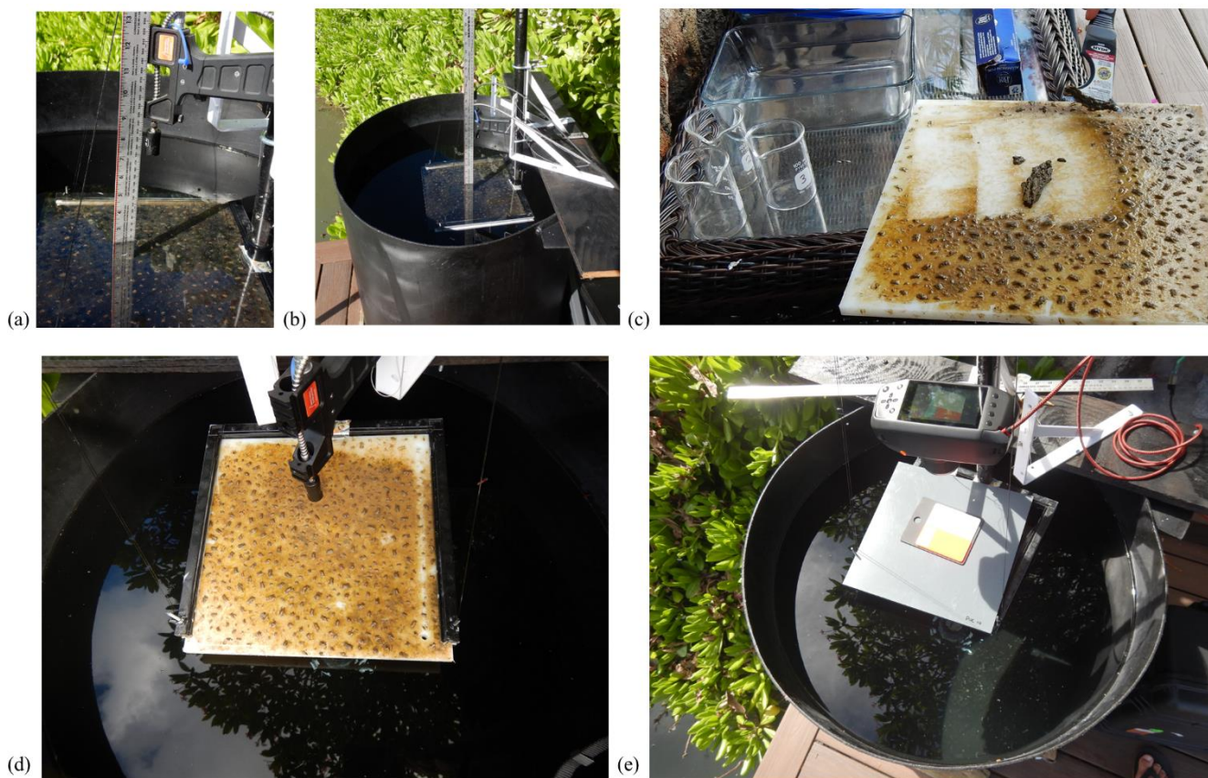
Figure 5 (a-b) Depth of submersion and distance of SEV lens to target measurements, (c) collection of biofilm to determine the biofilm mass for all the biofouled samples, (d) biofouled sample placed in position for SEV reflectance measurements and (e) SPECIM IQ camera collecting with a standard reference target.
