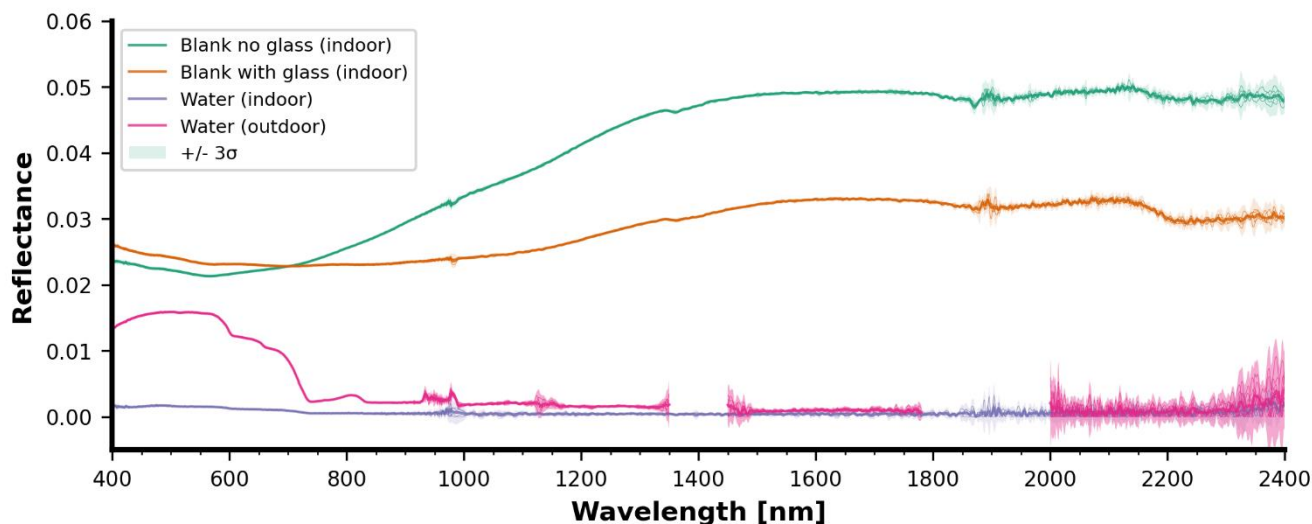
300 Figure 14 Comparison of different blank measurements above water, for both the indoor laboratory and the outdoor mesocosm campaign. All sample measurements during the indoor laboratory campaign were taken with the 'Glass' or 'No glass' option, depending on the required setup. The black background plate has a higher reflectance than water. All measurements reported in this paper are raw reflectance measurements, meaning that the blank signal can still be subtracted to obtain material-specific reflectances with higher accuracy. Each curve is the average with the shading representing 3\sigma confidence interval.
