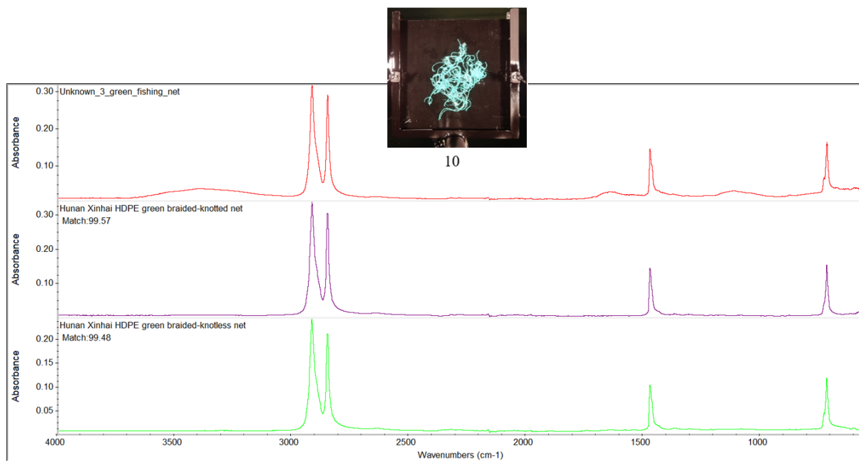
Figure D3 FTIR spectrum of the ocean-harvested green fishing net sample, indicating a match with HDPE.
