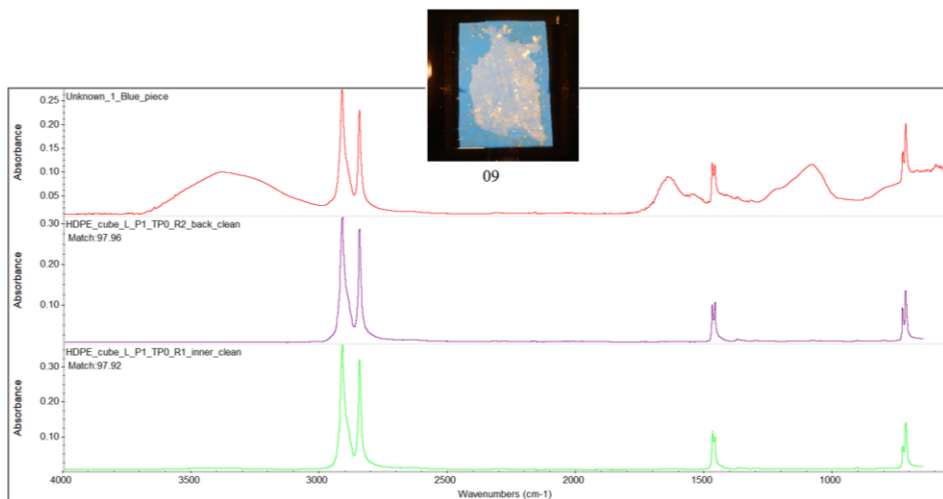
Figure DC1: FTIR spectrum of the blue ocean-harvested plastic, indicating a match with HDPE.
