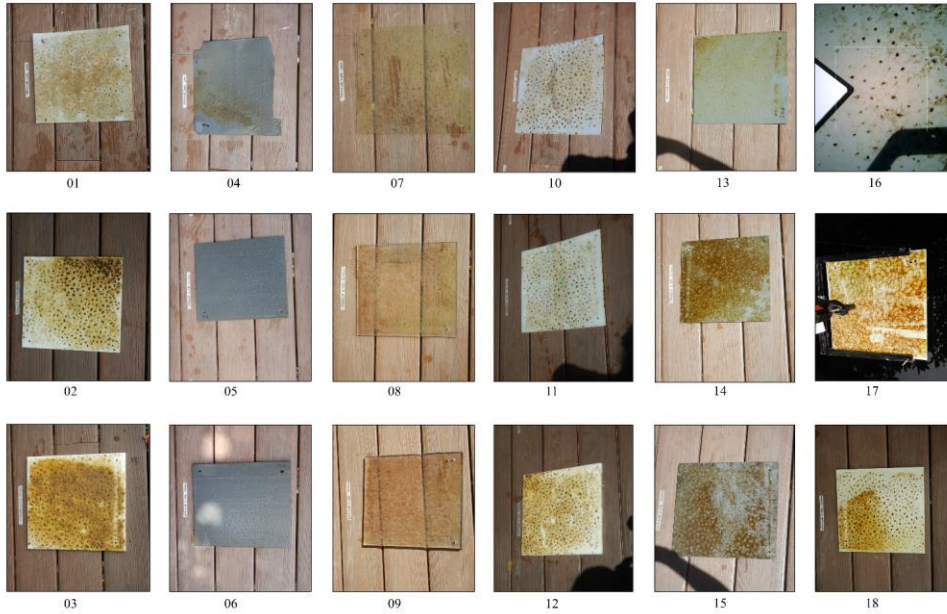
415 Figure A2 Overview of biofouled samples, used in the outdoor measurement campaign: HDPE (01 - 03), XPS (04-06), PET-G (07-09), PA6 (10-12), PVC (13-15), PP (16-18). Rows from top to bottom denote 1, 5, and 10 mm thickness, respectively. For PP 1 mm (16), the viewfinder preview of the SPECIM IQ camera is used as the overview image was found missing.
