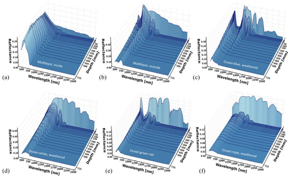
270 Figure 10 Spectral reflectance at varying depths for (a-b) multilayer inside and outside, (c) blue weathered ocean plastic, (d) white weathered biofouled dried ocean plastic, (e) a piece of green ocean net, and (f) weathered piece of ocean rope.
