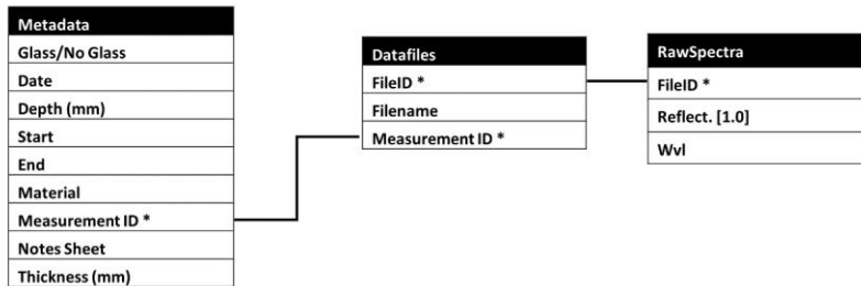
165 Figure 34 Data structure diagram for the hyperspectral measurement dataset. The table 'RawSpectra' contains the full set of raw data tables, concatenated from individual data files. The Metadata table contains the registration for each measurement and is linked to the RawSpectra through the Datafiles table. A Measurement ID from the Metadata table can have multiple FileIDs in the datafiles table. This also allows easy selection and aggregation of duplicate measurements for averaging and statistics.
