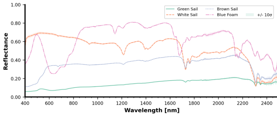
Figure 1240 Spectral reflectance of sailing-related objects, (a): white sail, sample ID 15 in Figure A1Figure-1. (b): brown sail, sample ID 17 in Figure A1Figure-1. (c): green sail, sample ID 16 in Figure A1Figure-1. (d): blue foam, sample ID 14 in Figure A1Figure-1. Each curve is accompanied by a 10σ confidence interval and individual measurement lines (colored hairlines), albeit barely visible due to the low variance of each set of five measurements.
