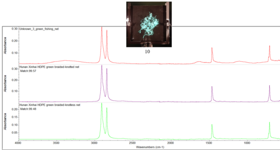
Figure DC3: FTIR spectrum of the ocean-harvested green fishing net sample, indicating a match with HDPE.
