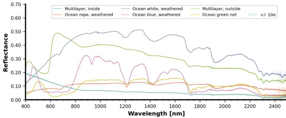
Figure 11 Surface-level spectral reflectance of the six materials displayed in Figure 10. Each curve is accompanied by a 10σ confidence interval and individual measurement lines (black hairlines), albeit barely visible due to the low variance of each set of five measurements.
