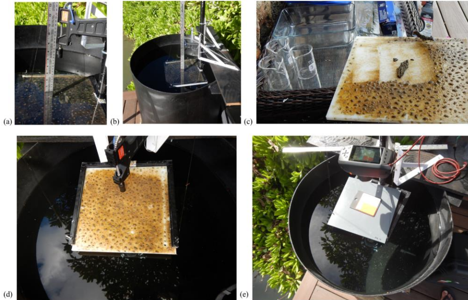
210 Figure 56 (a-b) Depth of submersion and distance of SEV lens to target measurements, (c) collection of biofilm to determine the biofilm mass for all the biofouled samples, (d) biofouled sample placed in position for SEV reflectance measurements and (e) SPECIM IQ camera collecting with a standard reference target.
