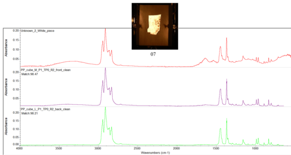
435 Figure DC2: FTIR spectrum of the ocean-harvested white piece of plastic, indicating a match with PP.
