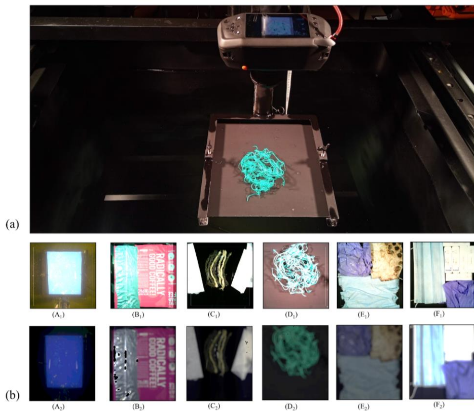
145 Figure 22 (a) The SPECIM IQ camera, positioned over one of the samples, and (b) the samples that were recorded by the SPECIM IQ. Subscript (1) denotes the image taken from the viewfinder, and subscript (2) denotes the RGB composite from the SPECIM hypercube. The samples were: weathered ocean blue plastic front side (A), multilayer packaging, inside and outside combined (B), ocean rope (C), ocean green net (D), composite (old medical gloves, old medical face mask, white oceanhite plastic, (E)), and a composite of new face mask, new medical glove, and rapid antigen tests (F).
