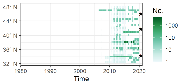
335 Figure 3: The number of measurements within 50 km of the shore and 25 m of the surface for temperature (a), dissolved oxygen (b), and any carbonate system measurements (c) using two-month, 0.5-degree latitude spatiotemporal blocks. Salinity (not shown) hews closely to the dissolved oxygen distribution. From north to south, stars mark the Washington-Oregon border, the Oregon-California border, and Point Conception (34.5° N). Spatial data coverage was best across all parameters between 2010 and 2015, whereas overall observation quantity was highest between 2015 and 2020. Since 2015, dissolved oxygen and carbonate system measurements have become more concentrated into fewer locations along the coast despite increasing awareness of the risks of 340 nearshore acidification and hypoxia events.
