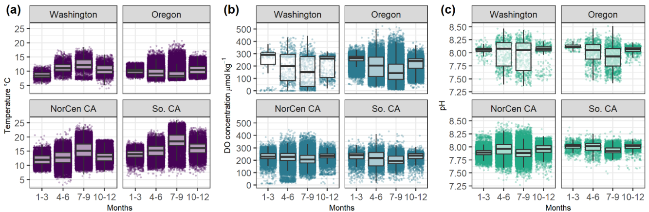
380 Figure 5: Measurements shoreward of the 100 m bathymetric contour of temperature (a), dissolved oxygen (DO) (b), and pH (c) capture intra-annual and regional variation. The lowest median DO and pH conditions are found with the highest temperatures in late summer, rather than during peak upwelling periods (April – June). Here, California is split into two regions: NorCen CA, spanning the northern border to Point Conception (34.5 N), and So. CA, from Point Conception to the southern border. Ninety-nine percent of the data falls within 30 km of shore and 65% falls within 10 km of shore.
