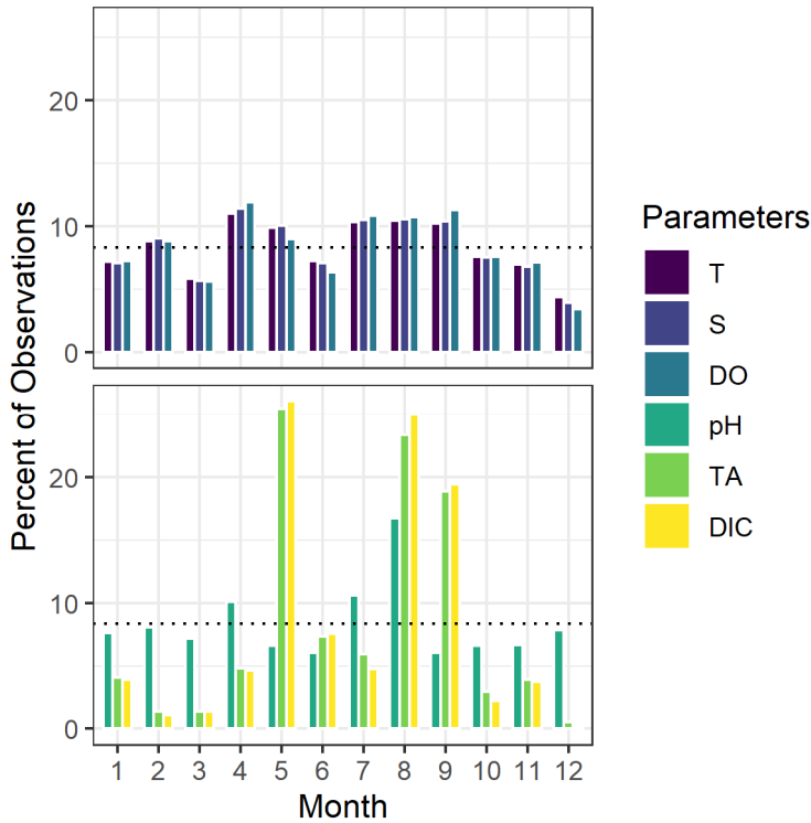
355 Figure 4: The distribution of daily observations by month varies substantially by parameter relative to an equal split (dashed lines). Temperature (T), salinity (S), and dissolved oxygen (DO) observations are fairly evenly distributed across seasons, with notable observational peaks in April, May, July, August, and September. Carbonate system parameters (pH, total alkalinity or TA, and dissolved inorganic carbon or DIC) are more concentrated in the summer months, with nearly all TA and DIC observations occurring in May, August, or September. Of the carbonate system parameters, only pH observations are nearly 360 equitably distributed throughout the year.
