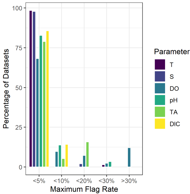
310 Figure 2: The rate of unreliable (“flagged”) observations varied by dataset and parameter measured between temperature (T), salinity (S), dissolved oxygen (DO), pH, total alkalinity (TA), and dissolved inorganic carbon (DIC). Maximum unreliable flag rates were generally low, especially for T and S. All datasets that included measurements with > 30% flag rates used measurement methods described by the original publishers as “not quantitative”. Flag rates between 10% and 30% were uncommon but reflected occasional periods of fouling or equipment malfunction in high resolution autonomous sensor datasets or, in rare cases, more stringent standards applied to datasets that had not been previously published and initially quality controlled. 315
