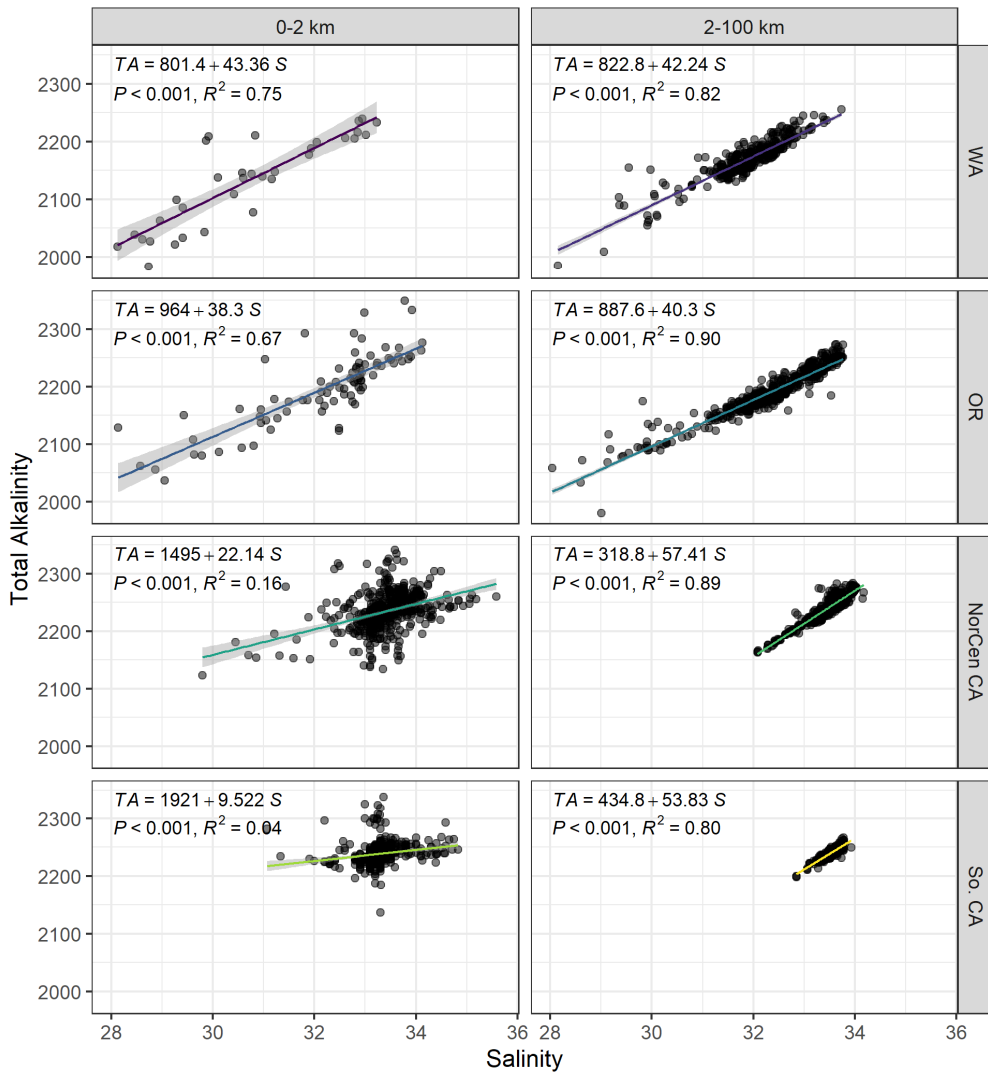
440 Figure 7: Regional near-surface (< 25 m) total alkalinity (TA)-salinity relationships from 0-2 km from shore and 2-100 km offshore in along the U.S. West Coast. As with Figure 5, the break between northern and southern CA is Point Conception, at 34.5° N. These relationships reflect only direct measurements of salinity and TA on discrete samples with salinity > 28.
