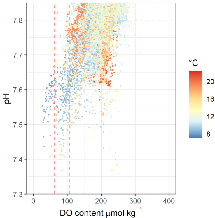
Figure 6: Low dissolved oxygen (DO) and pH conditions are frequently present in state waters (within 5 km of the shore) and 50 m of the surface. pH measurements below 7.8 (grey dashed horizontal line) are common but are more rarely accompanied by mildly hypoxic ( < 107 \mu\text{mol kg}^{-1} or 3.5 \text{ mg L}^{-1} DO, grey dashed vertical line) or hypoxic ( < 61 \mu\text{mol kg}^{-1} or 2 \text{ mg L}^{-1} DO, red dashed vertical line) conditions. Simultaneous low pH, low DO events are typically associated with low temperatures, whereas low pH conditions alone are present across a wide range of temperatures.
