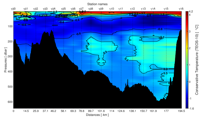
(b) Conservative Temperature [ ^{\circ}C ]
