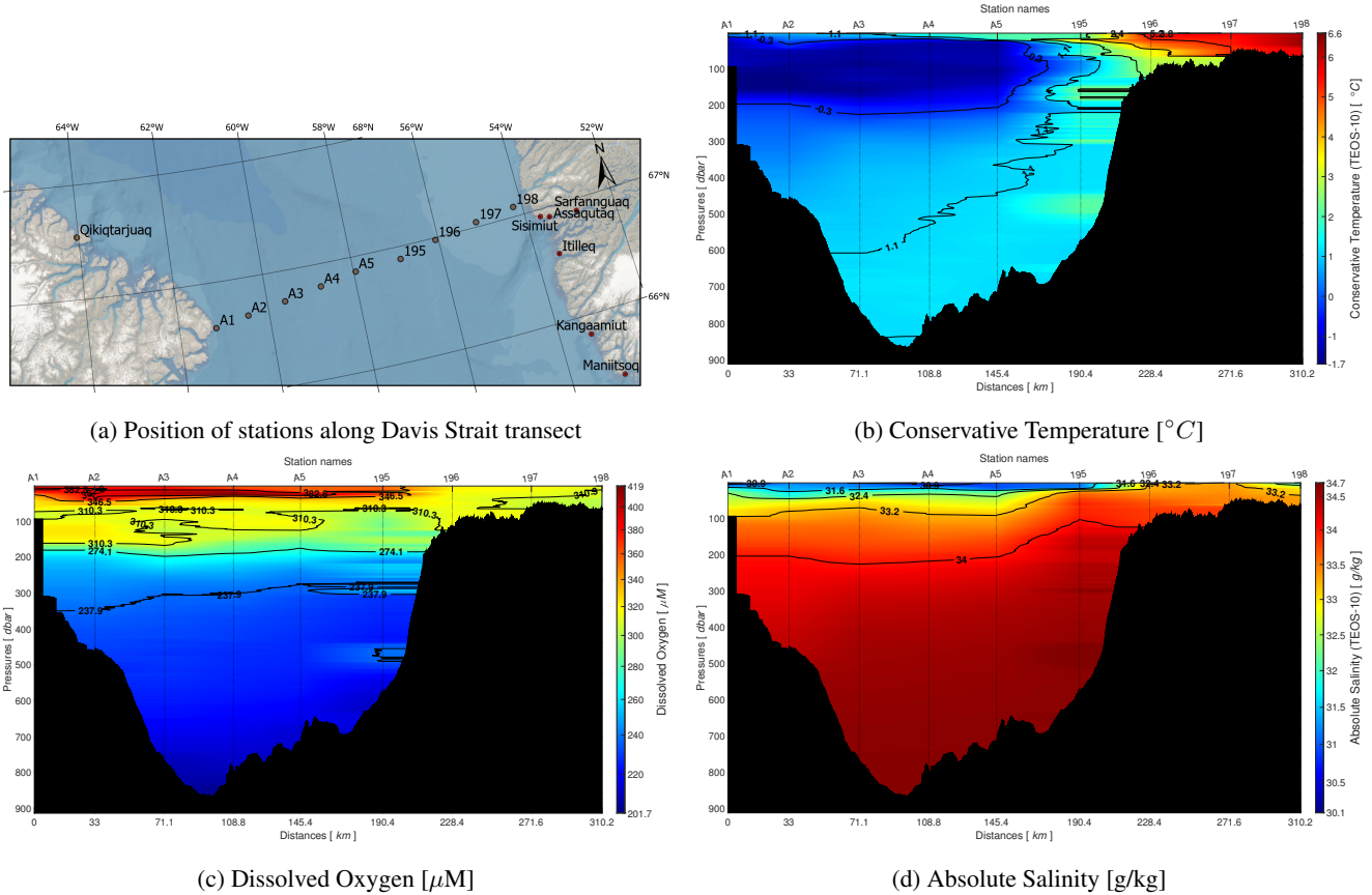
Figure 4. Davis Strait transect profiles during leg 3 of 2021 expedition. Isolines represent the variable presented at each subfigure.
