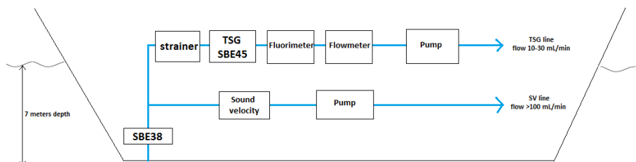
Figure C1. Schematic of the thermosalinograph
