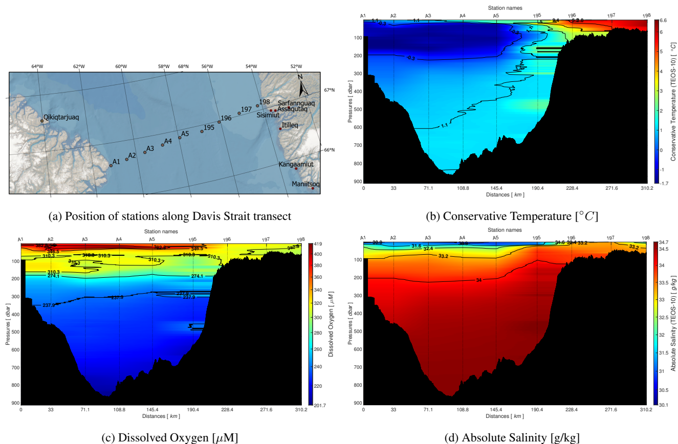
Figure 4. Davis Strait transect profiles during leg 3 of 2021 expedition. Isolines represent the variable presented at each subfigure.
