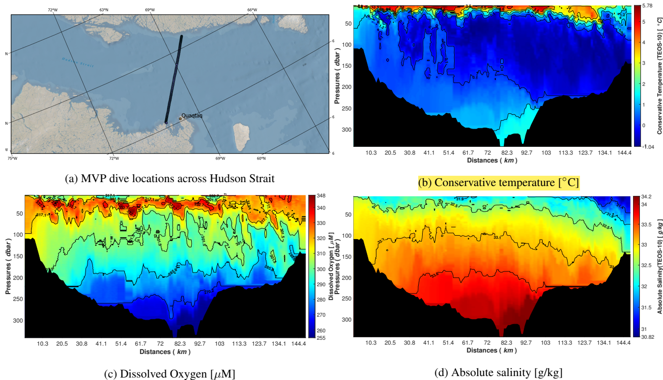
Figure 10. MVP section profile across Hudson Strait from Leg 3 of the 2021 expedition.
