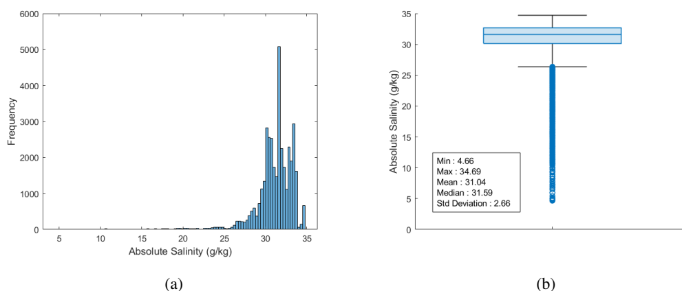
Figure 11. Histogram 11a and boxplot 11b of the absolute salinity values from the TSG system collected during Leg 2 of the 2021 expedition.
