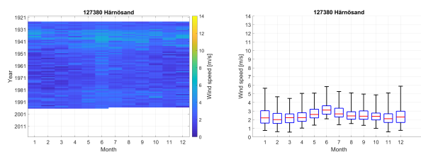
Figure A10. Data screening plot for Hårnösand. Left panel shows the data coverage and the monthly mean wind speed value according to the color bar, while the right panel shows the monthly wind speed, where the red line is the monthly mean wind speed, the upper and lower limits of the box 75- and 25-percentile and the end-bars represents the maximum and minimum monthly mean wind speed.
