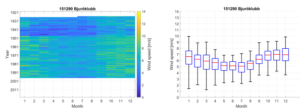
Figure A12. Data screening plot for Bjuröklubb. Left panel shows the data coverage and the monthly mean wind speed value according to the color bar, while the right panel shows the monthly wind speed, where the red line is the monthly mean wind speed, the upper and lower limits of the box 75- and 25-percentile and the end-bars represents the maximum and minimum monthly mean wind speed.
