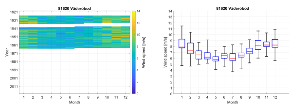
Figure A7. Data screening plot for Väderöbod. Left panel shows the data coverage and the monthly mean wind speed value according to the color bar, while the right panel shows the monthly wind speed, where the red line is the monthly mean wind speed, the upper and lower limits of the box 75- and 25-percentile and the end-bars represents the maximum and minimum monthly mean wind speed.
