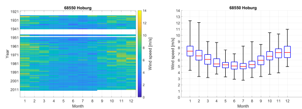
Figure A2. Data screening plot for Hoburg. Left panel shows the data coverage and the monthly mean wind speed value according to the color bar, while the right panel shows the monthly wind speed, where the red line is the monthly mean wind speed, the upper and lower limits of the box 75- and 25-percentile and the end-bars represents the maximum and minimum monthly mean wind speed.
