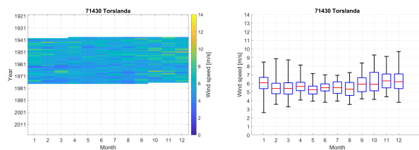
Figure A4. Data screening plot for Torstlanda. Left panel shows the data coverage and the monthly mean wind speed value according to the color bar, while the right panel shows the monthly wind speed, where the red line is the monthly mean wind speed, the upper and lower limits of the box 75- and 25-percentile and the end-bars represents the maximum and minimum monthly mean wind speed.
