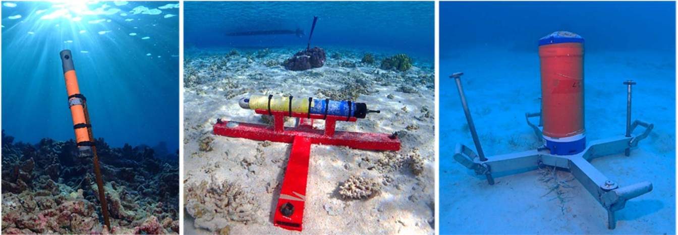
365 Figure 8: Images of moored structures and deployed instruments in Raroia atoll. Left: PVC tube for RBRduet T.D or SBE56 sensors fixed on hard coralline bottom. Middle: Aquadopp Nortek (on the forefront) and Marotte HS (at the back) moored on same station on pavement or coral head. Right: ADCP Sentinel instrument moored at the bottom of a deep lagoon (photos: Serge Andréfouët)
