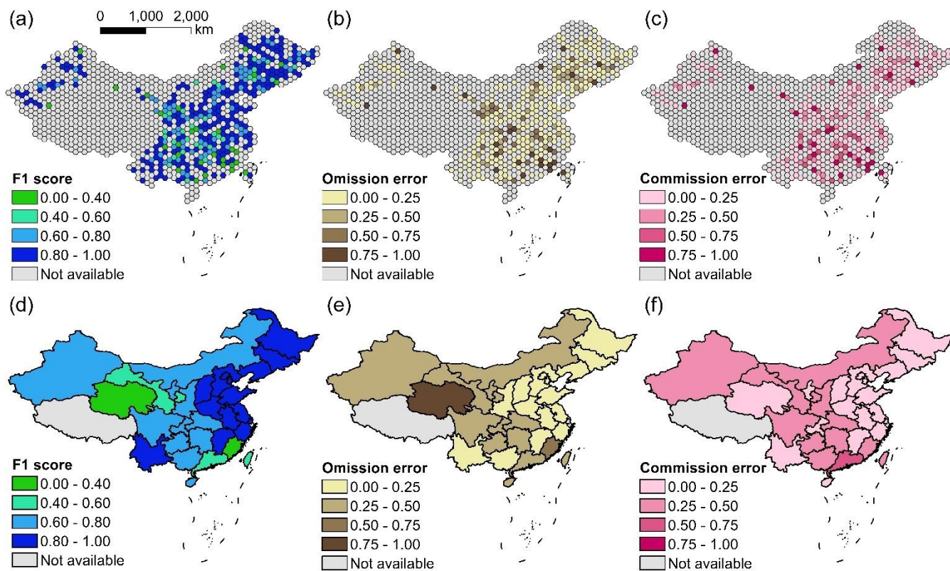
710 Figure 4: Spatial variation of mean accuracy of CACD for 1986-2020. (a-c) Hexagon level. Noted only hexagons containing both cropland and non-cropland samples were calculated. (d-f) Province-level. Noted Xizang, Hong Kong, and Macau were excluded from the analysis due to small numbers of cropland samples.
