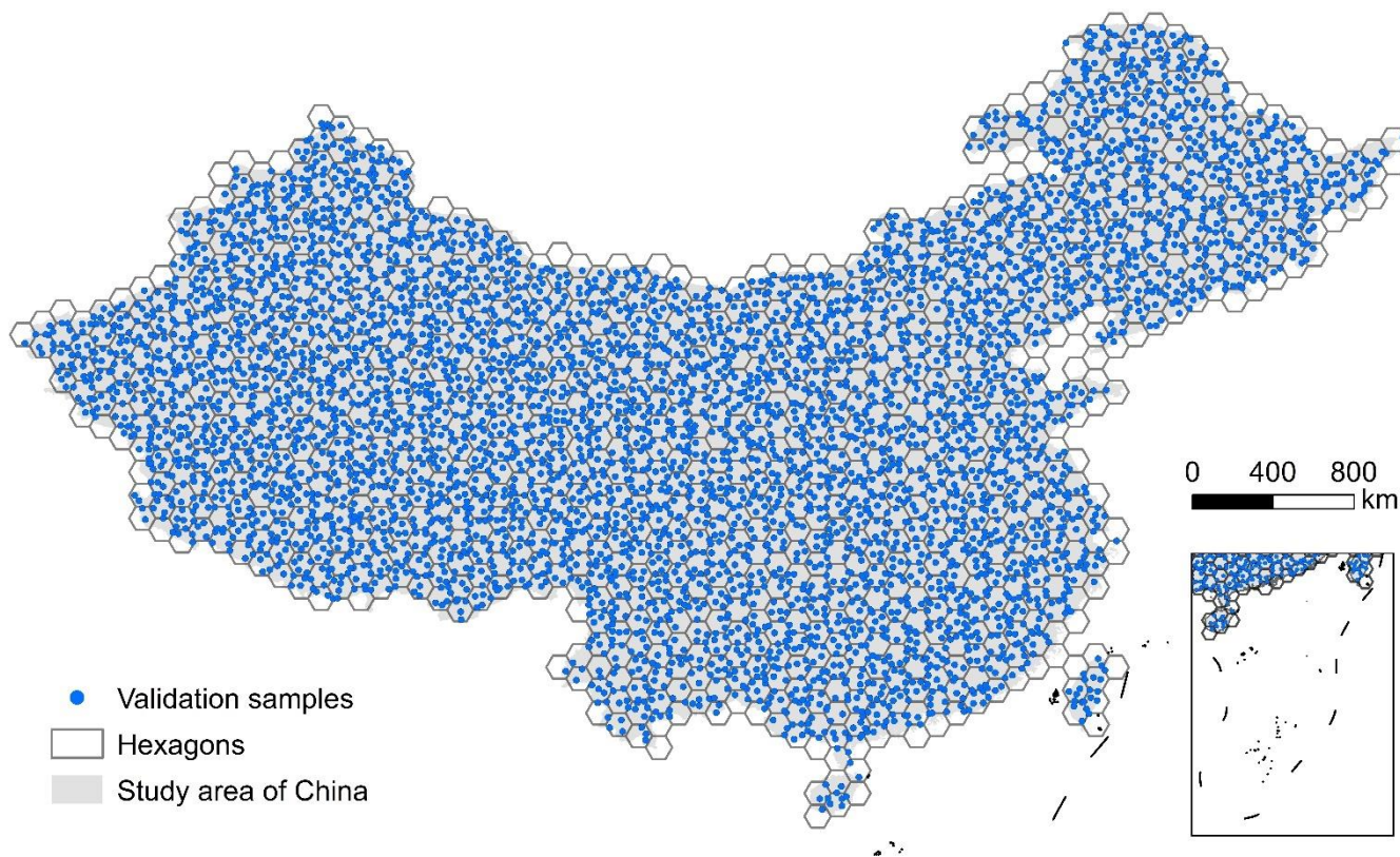
Figure 3: Distribution of validation samples.
