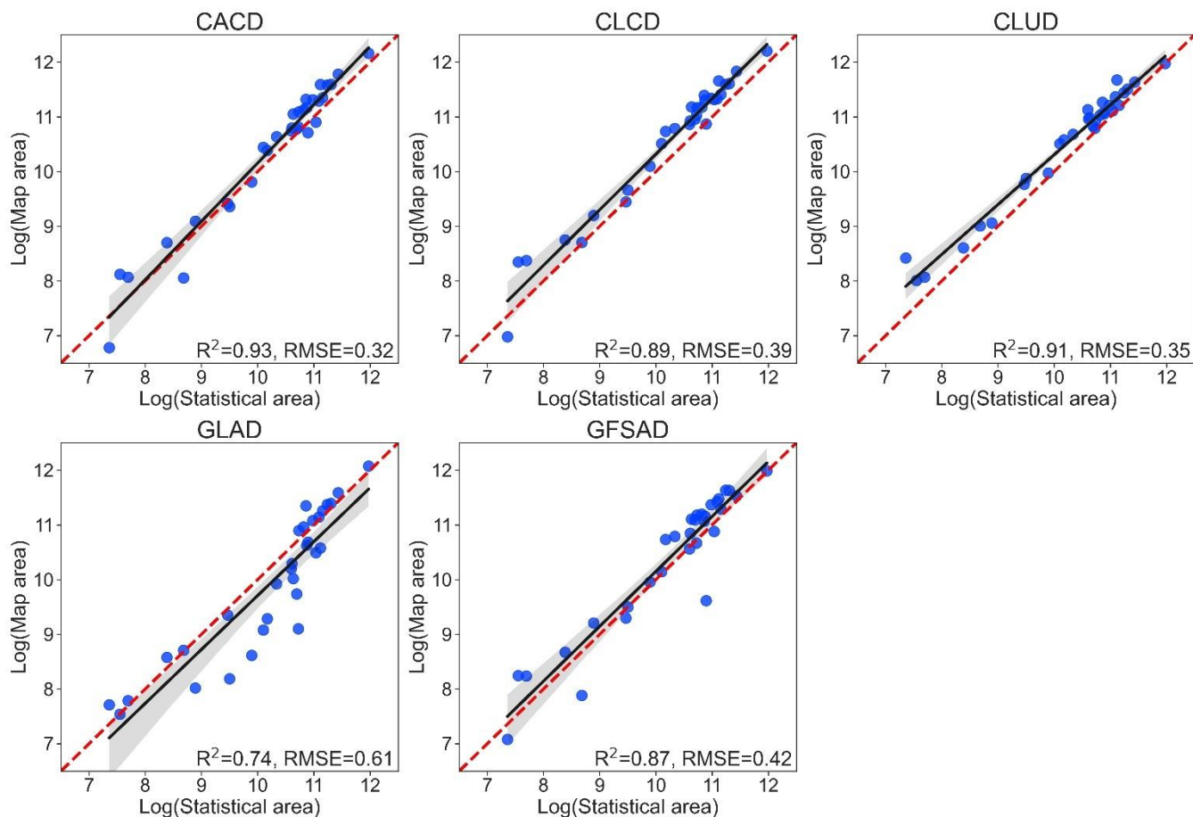
725 Figure 8: Scatterplots of the provincial cropland area in 2015 between the five products and the statistical data. The red dotted line represents the 1:1 diagonal.
