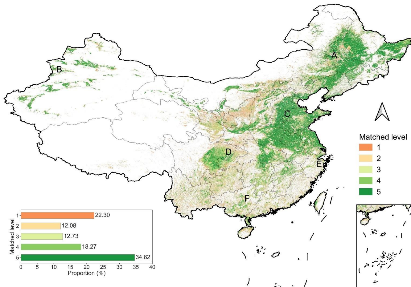
715 Figure 6: Spatial agreement of cropland extent of the five products (CACD, CLCD, CLUD, GLAD, and GFSAD) in 2015. Matched level indicates how often a pixel is identified as cropland. For example, '4' means four out of the five products recognize it as cropland. The bar chart in the lower-left corner denotes the area proportion of different matched levels (1-5). Locations A-F respectively correspond to zoomed areas in Figure 7.
