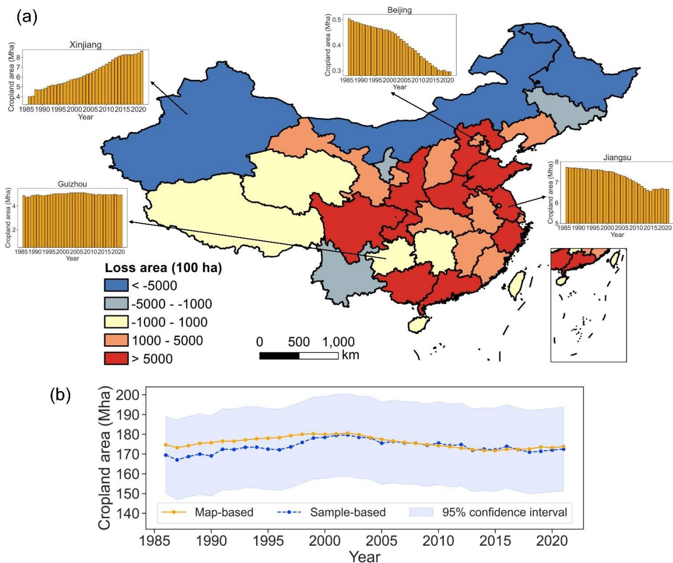
Figure 9: Cropland area changes in China between 1986-2021. (a) Provincial net loss derived from the CACD data. Negative values indicate cropland gain. (b) Annual dynamics of the map-based and the sample-based cropland area at the national scale.
