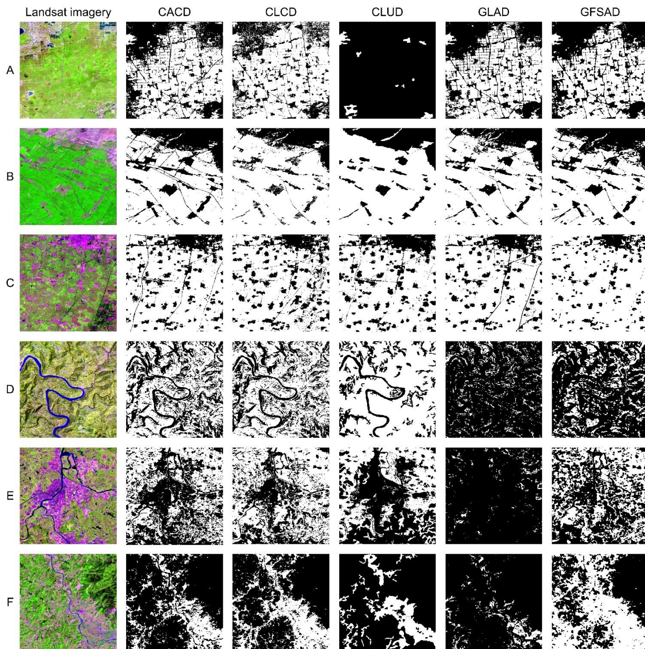
720 Figure 7: Regional comparisons of the five products in 2015. Referencing Landsat imagery in the first column is composed by SWIR1, NIR, and Red bands in RGB channels. Columns 2-6 display the spatial distribution of the five products, with cropland shown in white and non-cropland shown in black. All maps have a scale of 1:100000. Locations of A-F are shown in Figure 6.
