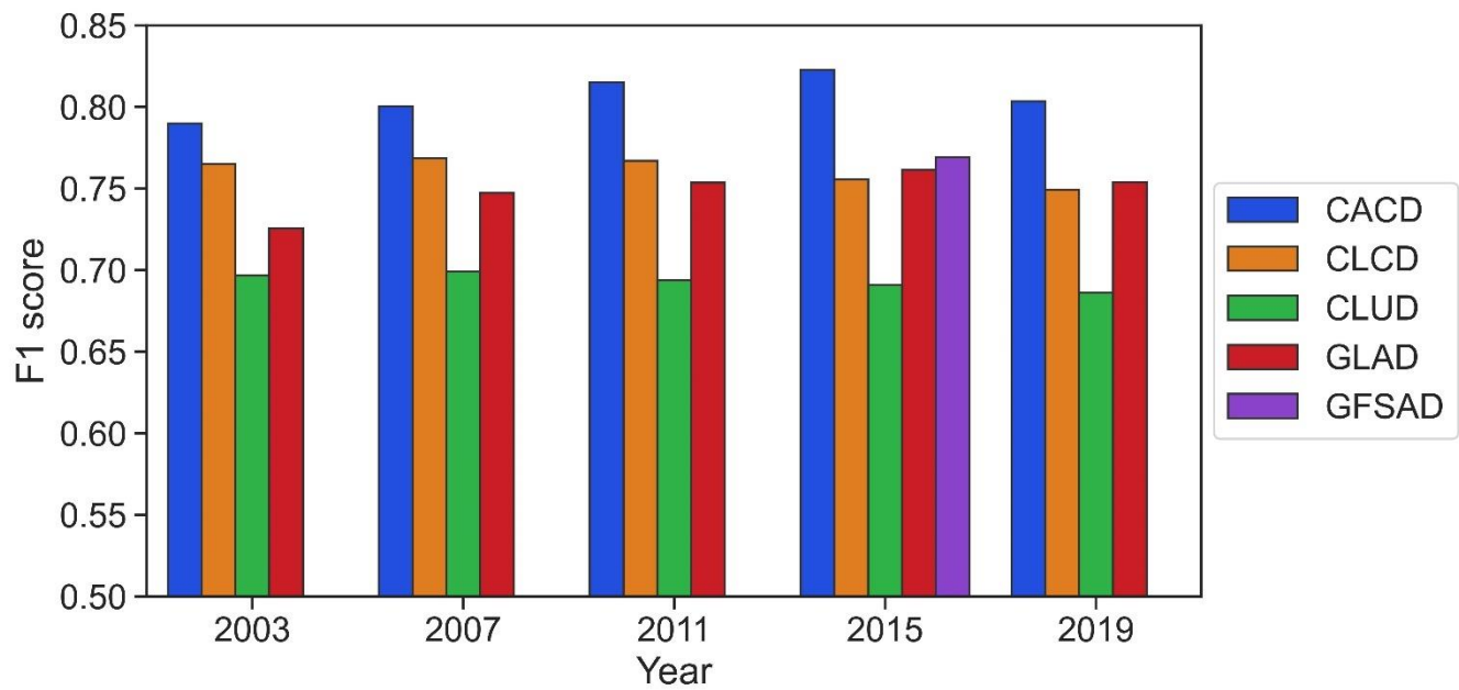
770 Figure 5: Comparisons of the pixel-wise accuracy of F1 score between the five products based on the annual validation samples.
