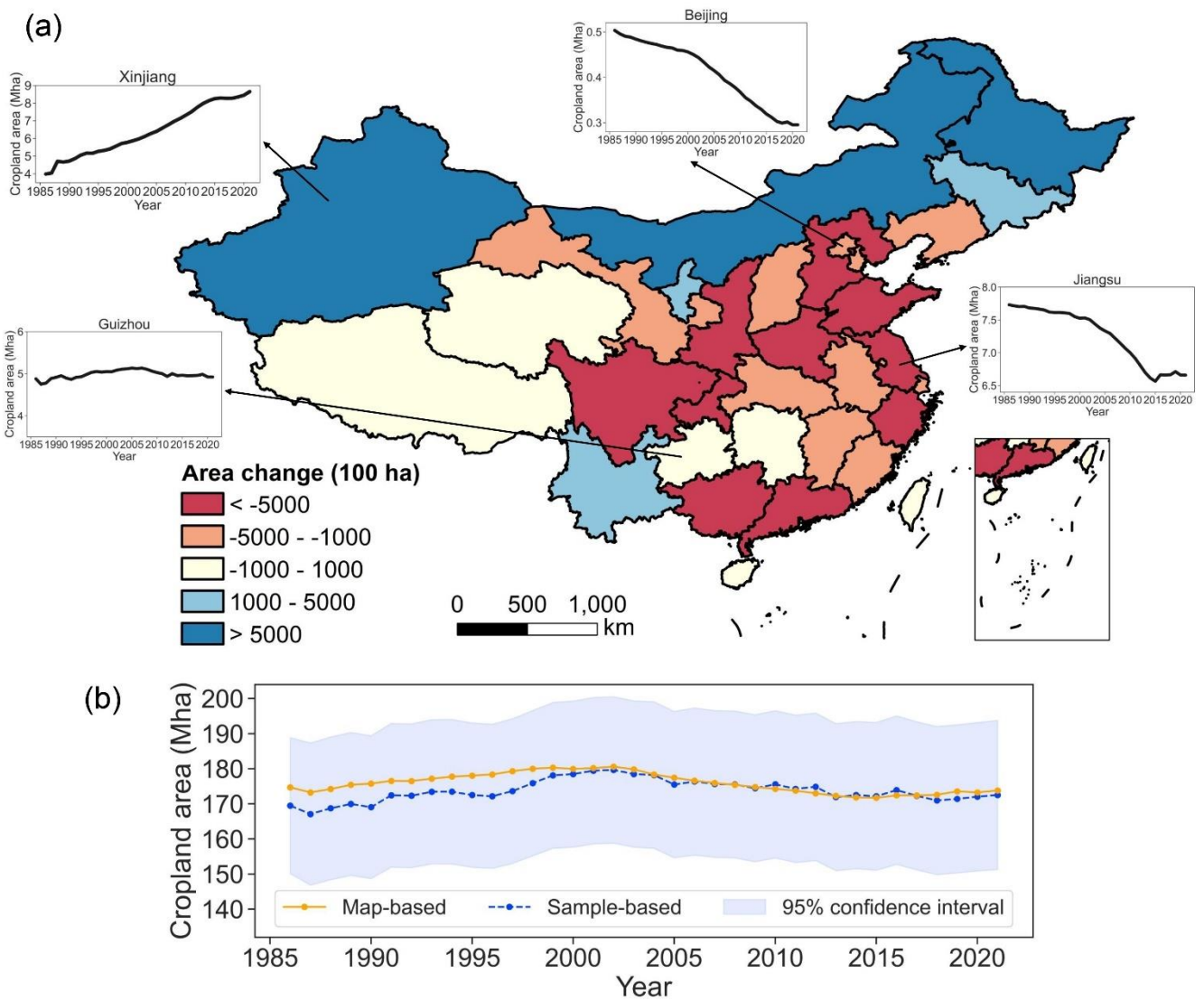
Figure 9: Cropland area changes in China between 1986-2021. (a) Provincial cropland change area derived from the CACD data. (b) Annual dynamics of the map-based and the sample-based cropland area at the national scale.
