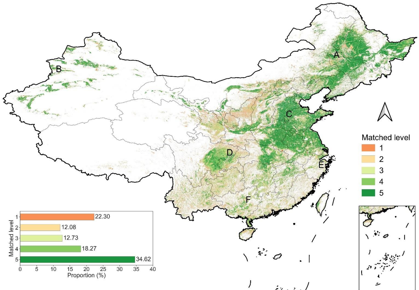
780 Figure 6: Spatial agreement of cropland extent of the five products (CACD, CLCD, CLUD, GLAD, and GFSAD) in 2015. Matched level indicates how often a pixel is identified as cropland. For example, '4' means four out of the five products recognize it as cropland. The bar chart in the lower-left corner denotes the area proportion of different matched levels (1-5). Locations A-F respectively correspond to zoomed areas in Figure 7.
