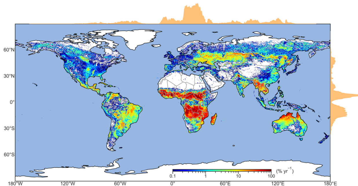
Figure 4. Global distribution of the mean annual GFED5 burned area, expressed as a percentage of the burnable land area in each 0.25^\circ \times 0.25^\circ grid cell, from 2001 to 2020. The two area charts displayed above and to the right of the map provide a visual representation of the relative fractions of burned area along the longitude and latitude axes, respectively.
