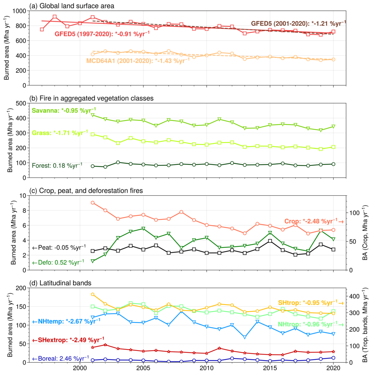
1135 Figure 5. Long-term trends in global burned area from GFED5 (in % yr -1 ), normalized by the annual mean, for a) different time intervals and data products, b) normal type fires in aggregated vegetation classes, c) crop, peat and deforestation fires, and d) five latitudinal bands: Boreal (60°N-90°N), NHtemp (23.5°N-60°N), NHtrop (EQ-23.5°N), SHtrop (23.5°S-EQ), and SHextrop (90°S-23.5°S). Sign ‘*’ before the number indicates a significant (p < 0.05) trend value. Labels and arrows on panels c & d denote the y-axis scale for each GFED5 burned area category.
