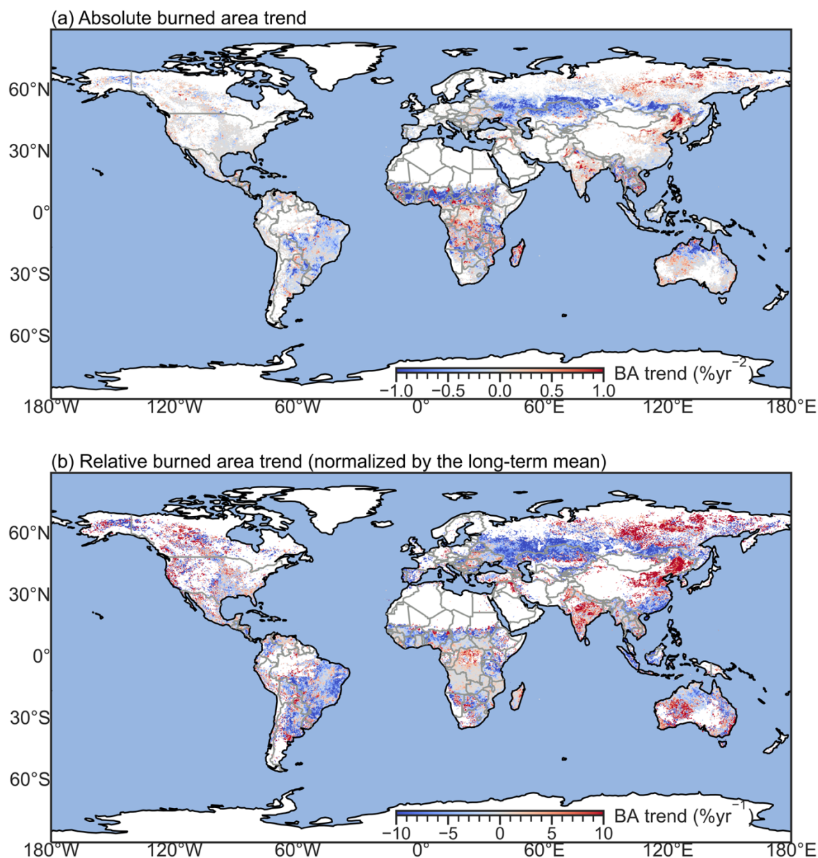
1145 Figure 6. Global maps of GFED5 burned area trends during 2003-2020. (a) Map of the linear trend in units of absolute change in percent burned area for each 0.25^\circ grid cell ( \% \text{ burned area yr}^{-2} ); (b) map of relative burned area trend in each grid cell ( \% \text{ yr}^{-1} ). The values in panel (b) were estimated by dividing the values in panel (a) by the all-year mean burned area shown in Figure 4.
