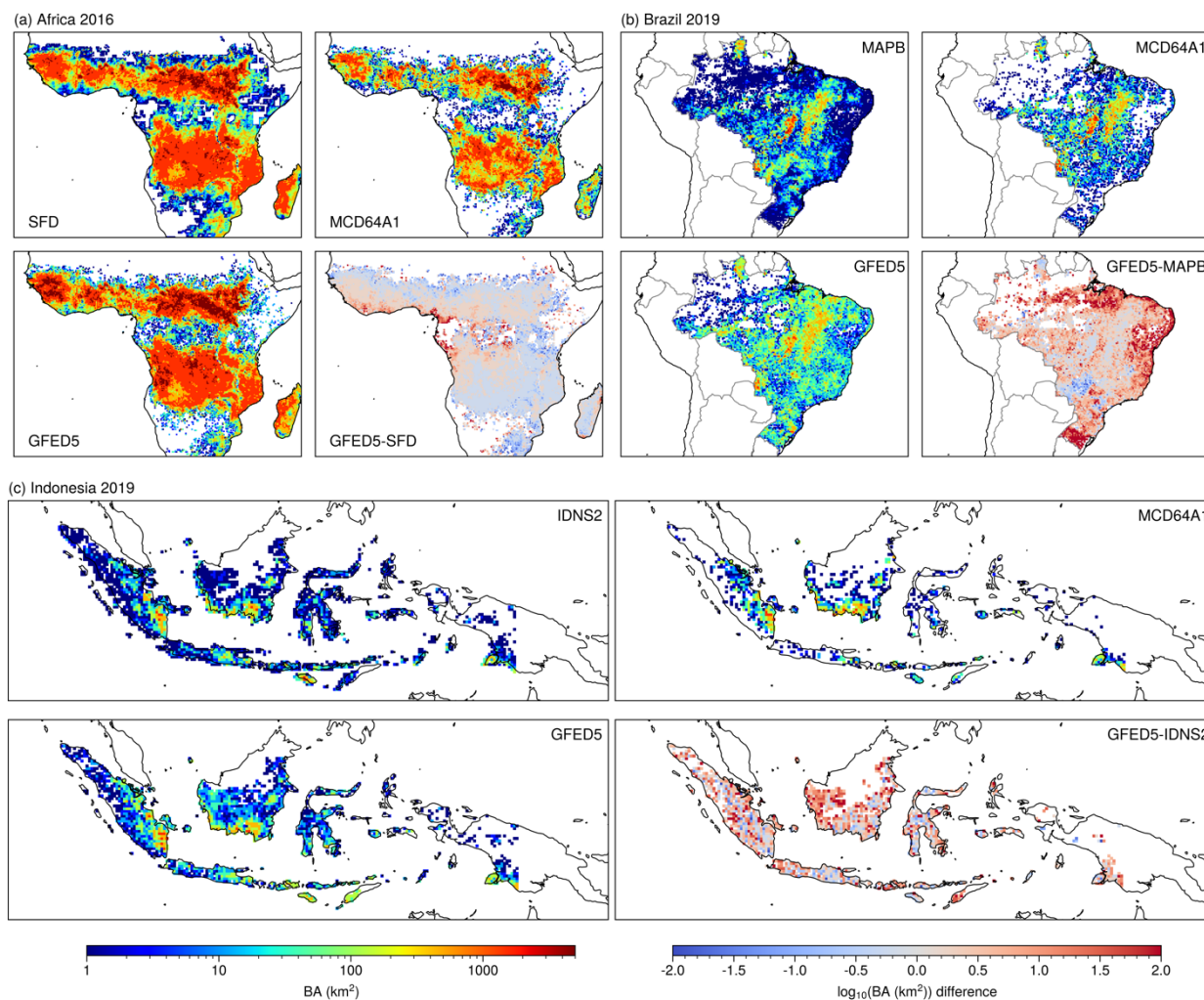
1190 Figure 11. A spatial ( 0.25^\circ \times 0.25^\circ ) comparison of burned area from GFED5 with burned area from MCD64A1 and higher 1190 resolution satellites (SFD for Africa, MAPB for Brazil, IDNS2 for Indonesia; see Table 1 for details) is shown for (a) Africa, (b) Brazil, (c) Indonesia.
