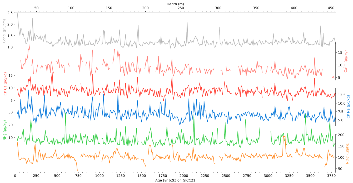
Figure 3. Overview of the complete data set at 10 yr resolution on the GICC21 (Sinnl et al., 2022) agescale. From top to bottom the data series are electrolytic meltwater conductivity (Cond.), \text{Ca}^{2+} measured by fluorescence spectrometry, Ca and Na measured by ICP-TOFMS, \text{NH}_4^+ measured by fluorescence spectrometry and \text{NO}_3^- , measured by absorption spectrometry. Note, that the \text{Ca}^{2+} record partly suffers from analytical issues leading to a large number of gaps in the final data set. However, the Ca data from the ICP-TOFMS covers not most of these gaps and provides an almost complete data set.
