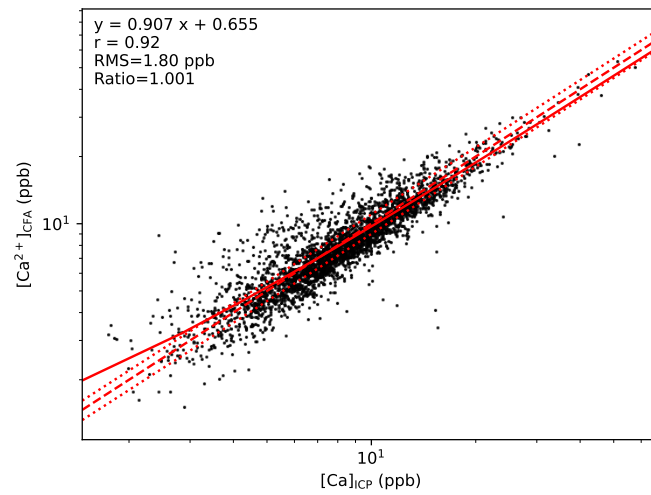
Figure 6. Cross plot of ICP-TOFMS Ca and fluorimetric \text{Ca}^{2+} concentrations at 10 cm resolution, considering only sections with less than 50 % missing data. Regression, Pearson correlation ( r ), root mean square error (rms) and average ratio were calculated on the concentrations (i.e. not log-transformed). The solid line is the result of the regression, the dashed line marks the 1:1 line, the dotted lines indicate a \pm 10\% deviation from that line.
