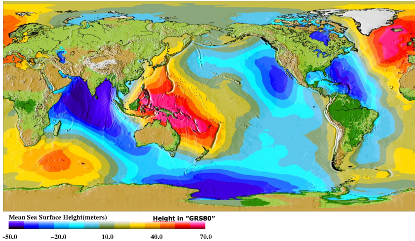
365 Figure 4: The DTU21 mean sea surface from the Technical University of Denmark (DTU) in meters
