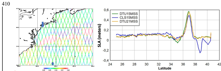
415 Figure 5: Sentinel-3A 5y mean sea level anomaly along track 791 in the Gulf Stream area relative to DTU15MSS (left). The Sentinel-3A track 791 is located between the with blue arrows in the left figure. The S3A mean anomalies relative to DTU15MSS, CLS15MSS and DTU21MSS (right).
