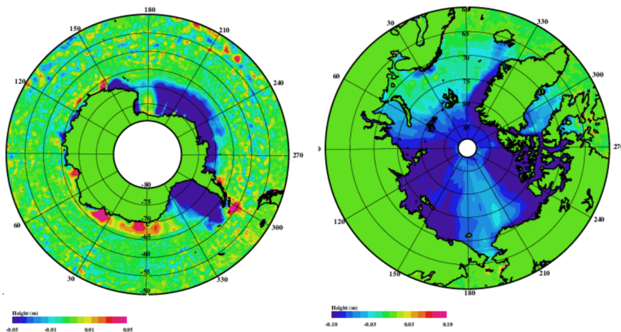
310 Figure 3. DTU21MSS-DTU15MSS for the Southern Ocean (left) and the Arctic Ocean (right). The color scale ranges up to +/- 5 cm for the Southern Ocean and +/-10cm for the Arctic Ocean.
