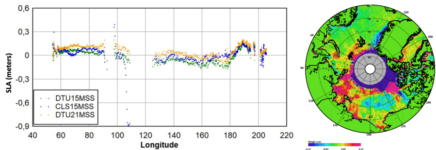
565 Figure 7. Sea level anomalies (in meters) between the 5-year S3A mean profile along track 497/498 and various MSS models in the Arctic Ocean (left). Right: Mean Sea Surface difference between DTU21MSS and CLS15MSS Dark Blue Regions north of Canada are voids in the CLS15MSS. The color scale ranges from -15cm to +15 cm.
