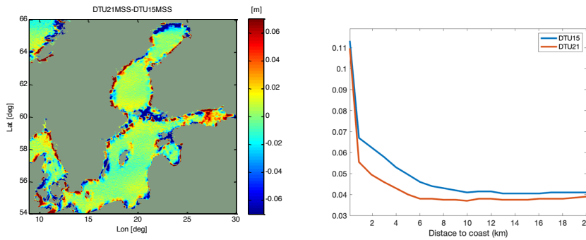
Figure 8: Difference between the DTU21MSS and the DTU15MSS in the Baltic Sea (left). Standard deviation (meters) relative to the the Danish vertical reference model DVR90 as a function of distance to coast (right).
