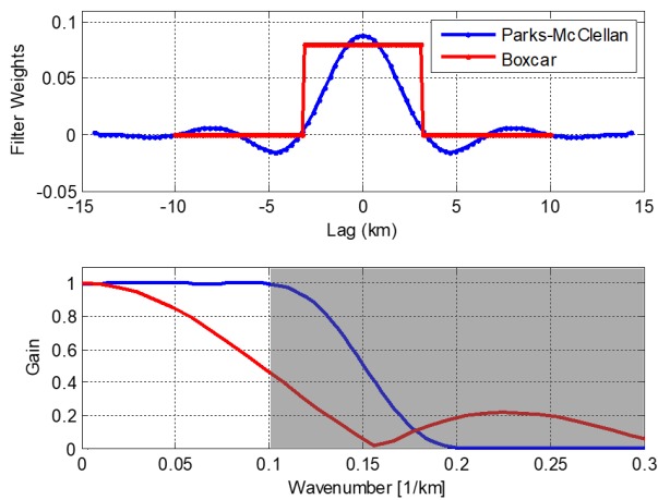
Figure 2: Illustration of Parks-McClellan filter weights (blue) and the boxcar filter (red) to derive 1 or 2-Hz SSH data spatial filter (upper panel). The lower panel illustrates the frequency response of the two filters. Sidelobes and spectral leakage in the 10-40 km wavelength can be seen for the boxcar filter, which will remain as high-frequency noise in the filtered dataset.
