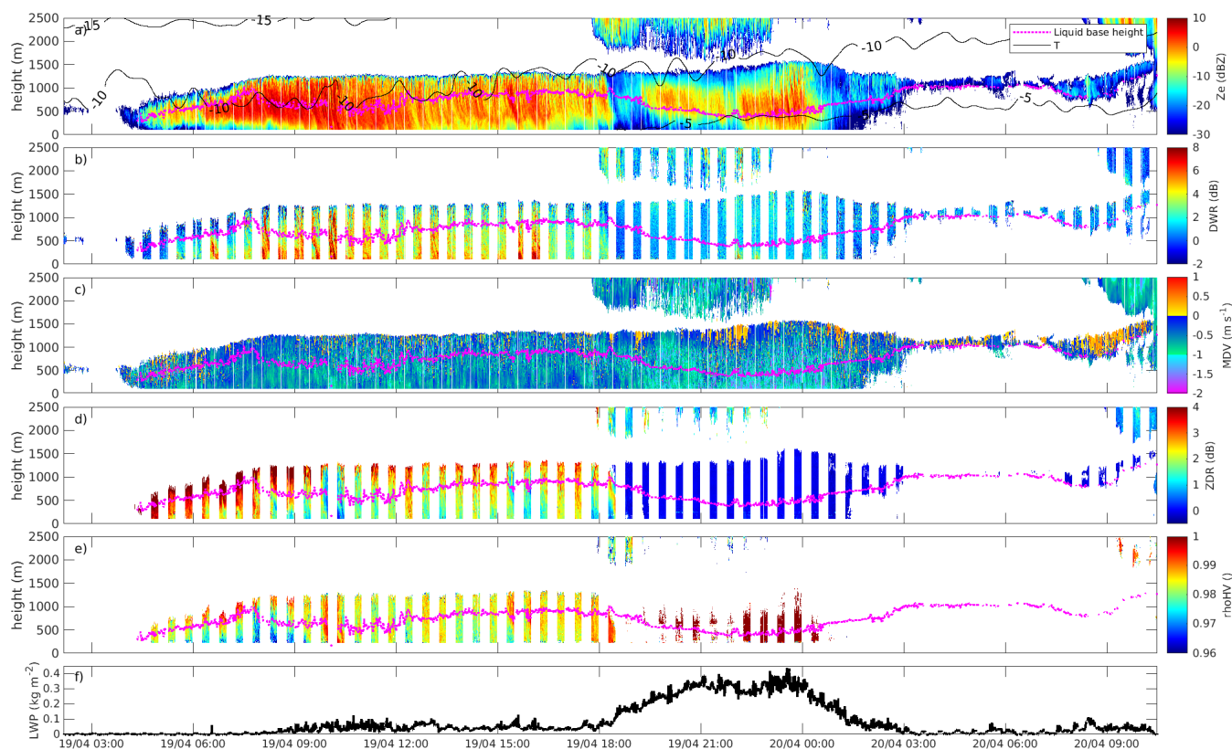
Figure 3. LLMPC event detected on 19-20 April 2022. Panels respectively display: reflectivity from W-band radar with temperature contours overlaid (a), dual-wavelength ratio (b), mean Doppler velocity from W-band radar (c), differential reflectivity (d), correlation coefficient (e), liquid water path (f). All radar variables were recorded at zenith elevation, except for differential reflectivity and correlation coefficient that were recorded at 30° elevation. The dotted magenta line on panels a through e indicates the base height of the lowest liquid layer.
