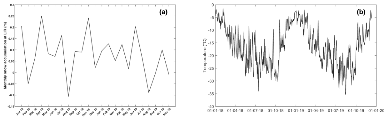
595 Figure A1. Meteorologic records from the AWS on the eastern side of LIR. Two years (from the 1 st of January 2018 to the 12 th of December 2019) of monthly snow accumulation (a) and daily temperature (b).
