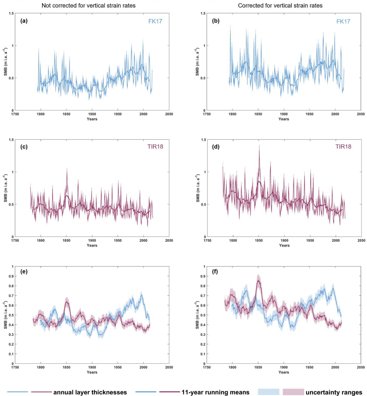
325 Figure 4. Surface mass balance in meter ice equivalent per year ( \text{m i.e. a}^{-1} ) (a-b) for FK17 core, (c-d) for TIR18 core. The thin lines connect the annual layer thicknesses and the thick lines are the 11-year running means. The shaded colored ranges show the uncertainties associated to the SMB. The left panels represent the annual layer thicknesses not corrected for strain rates and the right panels represent the annual layer thicknesses corrected for strain rates. (e-f) The smoothed SMB records result from the use of an 11-year running mean on SMB.
