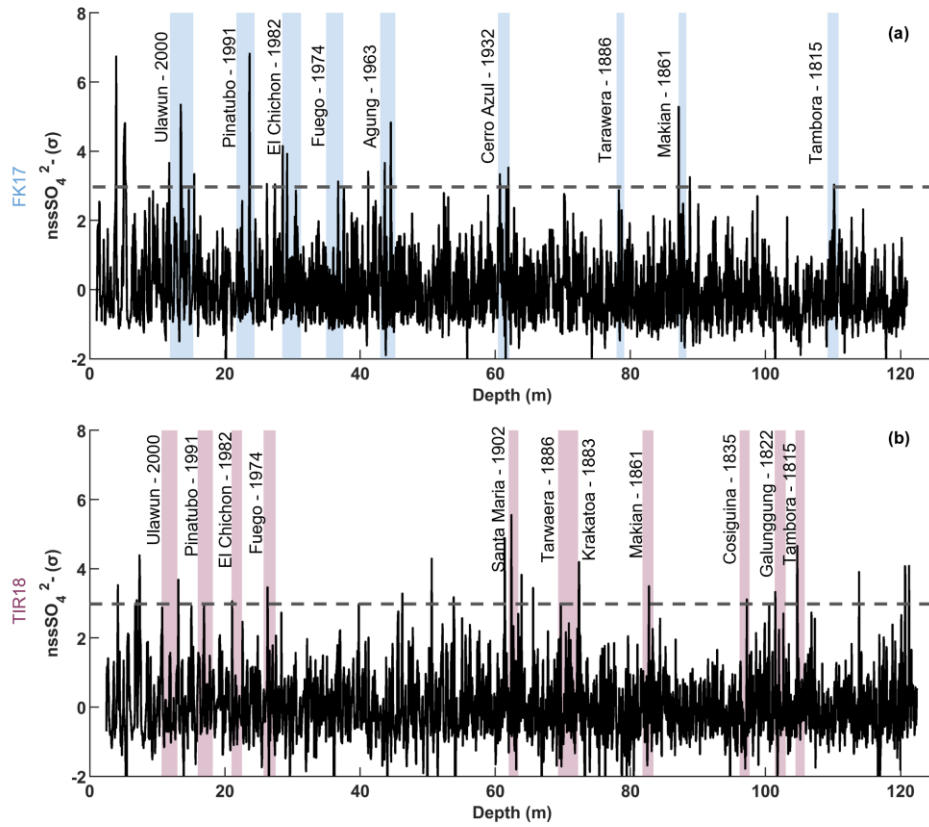
300 Figure 2. Normalized \text{nssSO}_4^{2-} records for FK17 (a) and TIR18 (b). The signal (black line) is expressed as a multiple of standard deviation ( \sigma ), the 3\sigma threshold is the dotted horizontal line, and identified volcanic peaks are shown as blue- or burgundy-colored bars, for FK17 and TIR18 respectively. The thicknesses of the color bars are related to the extended period during which the volcanic signal is potentially recorded in the ice core (year of the eruption + 2 years).
