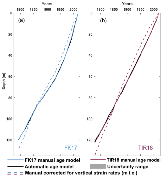
Figure 3. Age–depth profile reconstructed from the manual layer counting process for (a) FK17 (blue line) and (b) TIR18 (burgundy line). Black lines and grey shading are hardly distinguishable, they respectively show the automatic dating and the uncertainty range derived from StratiCounter. The dotted lines represent the manual age models expressed in m i.e. and corrected for vertical strain rates.
