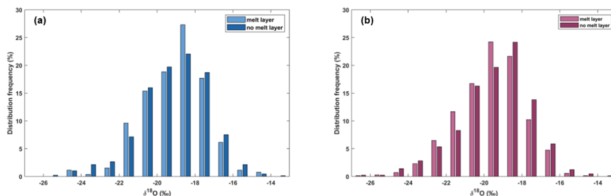
600 Figure C1. Distribution frequency of the \delta^{18}\text{O} samples “with” (lighter color) and “without” (darker color) bubble-free layers in FK17 (a) and TIR18 (b).
