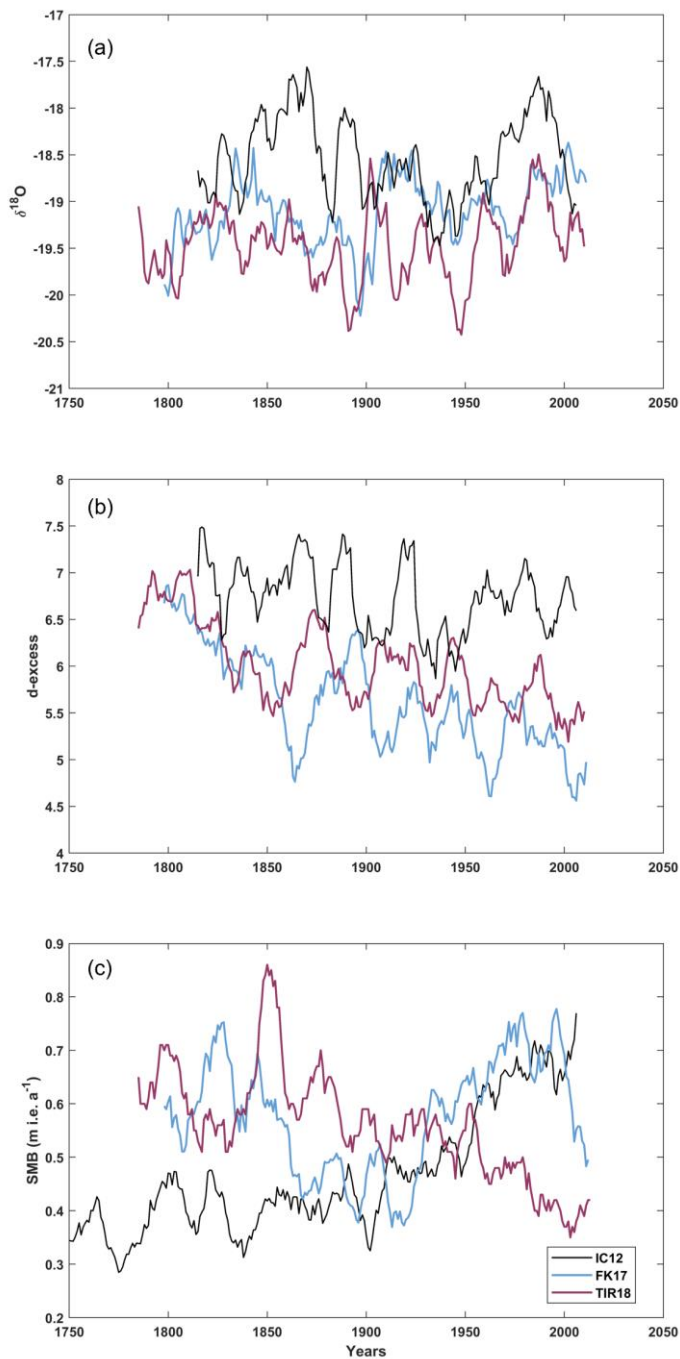
Figure G1. Comparison with IC12 (Philippe et al., 2016; Philippe and Tison, 2023). Note that these datasets have been smoothed using an 11-yr running mean. IC12 is in black, FK17 in blue and TIR18 in burgundy. (a) Annual mean \delta^{18}\text{O} signal. (b) Annual mean d-excess signal. (c) Surface mass balance corrected for vertical strain rates and expressed in m i.e. a -1 .
