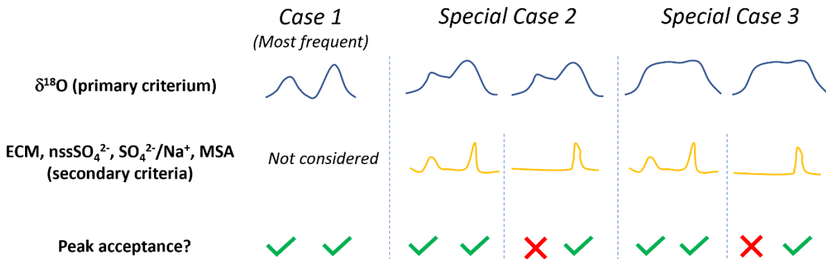
Figure D1. Canvas adopted by the operators for the relative manual dating process. \delta^{18}O has been chosen as the primary criterion of seasonal cycles. In most cases, \delta^{18}O peaks (taken as January of the year) are separated by clear troughs (case 1). The successive peaks are then considered as successive years. Two main special cases were encountered sporadically, with either a shoulder in the rising or decreasing \delta^{18}O signal (case 2) or a sustained plateau of unusual length (case 3). In those cases, the peaks were accepted when present in the majority of the secondary criterion for seasonal cycles (ECM, nssSO_4^{2-} , SO_4^{2-}/Na^+ , MSA).
