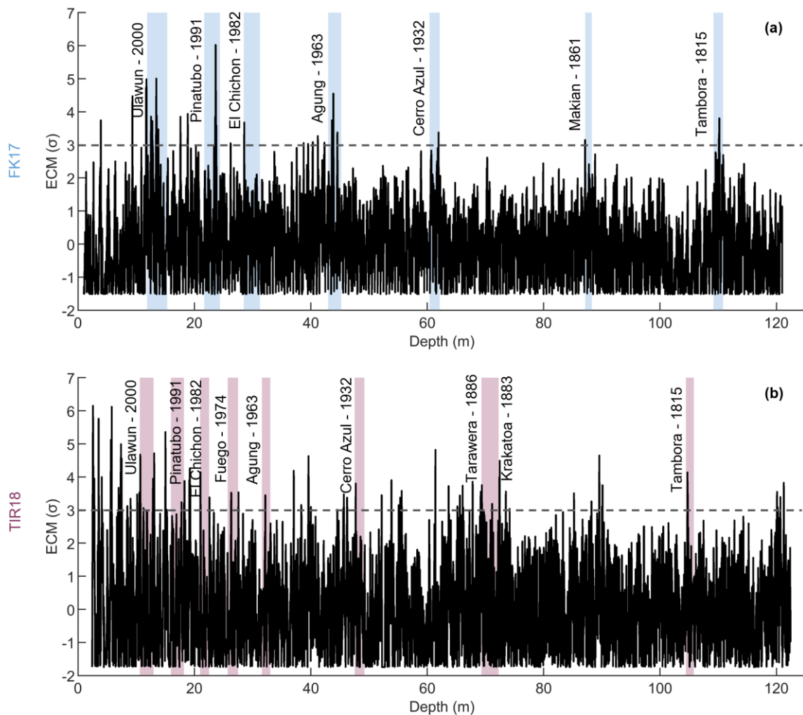
670 Figure F1. Normalized ECM records for FK17 (a) and TIR18 (b). The signal (black line) is expressed as a multiple of standard deviation ( \sigma ), the 3\sigma threshold is the dotted horizontal line, and identified volcanic peaks are shown as blue- or burgundy-colored bars, for FK17 and TIR18 respectively. The thicknesses of the color bars are related to the extended period during which the volcanic signal is potentially recorded in the ice core (year of the eruption + 2 years).
