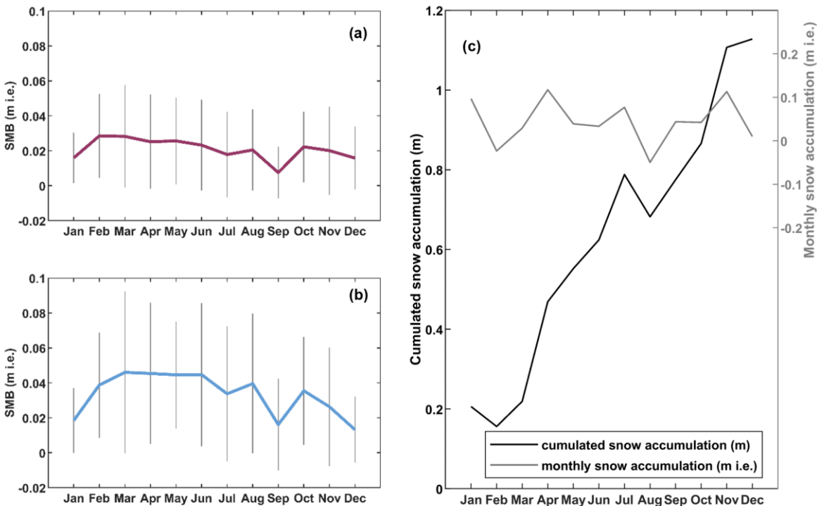
Figure E1. Conditions of snow accumulation at HIR and LIR. Monthly climatology of RACMO2.3 between 1979 and 2016 at (a) HIR and (b) LIR (based on Lenaerts et al., 2017). The color lines connect the climatology means and the vertical grey bars represent the climatology standard (a measure of the interannual variability). (c) A complete year (2018) of snow accumulation from an AWS located on LIR. The black line corresponds to the monthly cumulated snow height changes and the grey line corresponds to the monthly snow accumulation, calculated from the black line data. The m i.e. scale in (c) is calculated with a reference surface snow density of 430 \text{ kg m}^{-3} .
