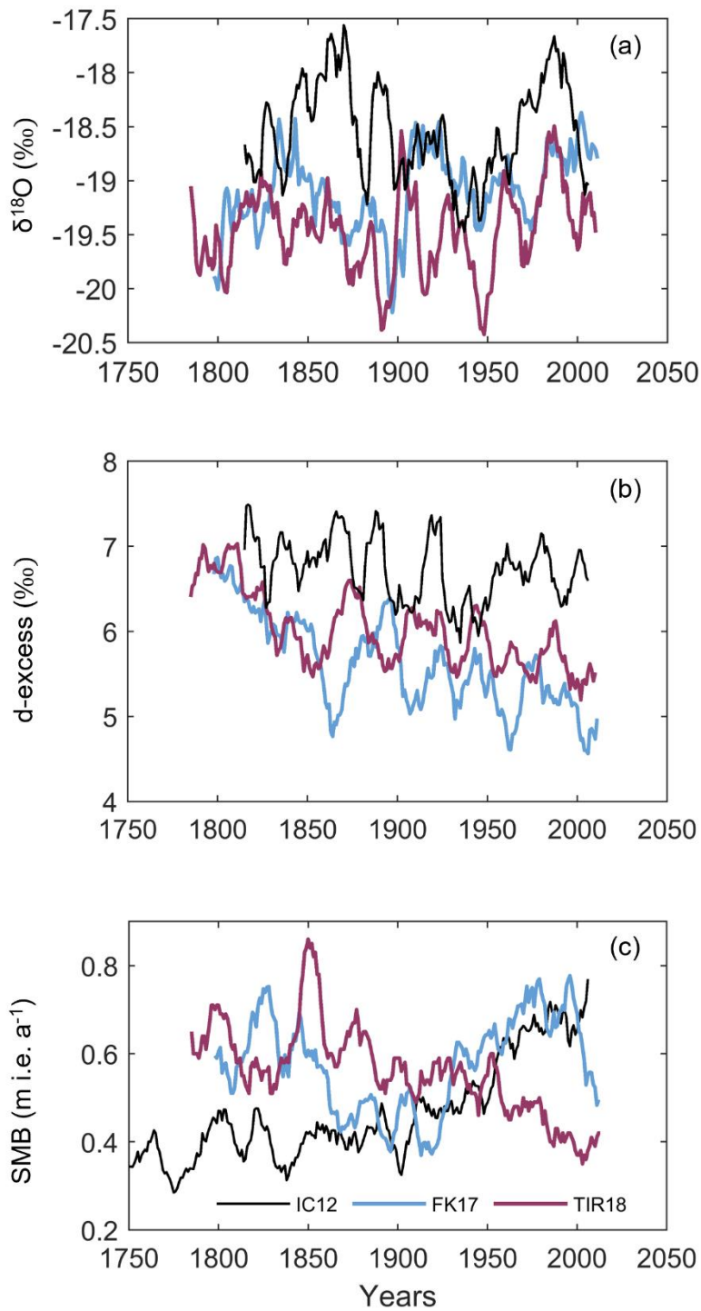
Figure C1G1. Comparison with IC12 (Philippe et al., 2016; Philippe and Tison, 2023). Note that these datasets have been smoothed using an 11-yr running mean. IC12 is in black, FK17 in blue and TIR18 in burgundy. (a) Annual mean \delta^{18}\text{O} signal. (b) Annual mean d-excess signal. (c) Surface mass balance corrected for vertical strain rates and expressed in m i.e. a -1 .
