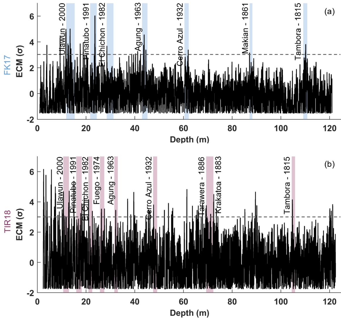
Figure FB1. Normalized ECM records for FK17 (a) and TIR18 (b). The signal (black line) is expressed as a multiple of standard deviation ( \sigma ), the 3\sigma threshold is the dotted horizontal line, and identified volcanic peaks are shown as blue- or burgundy-colored bars, for FK17 and TIR18 respectively. The thicknesses of the color bars are related to the extended period during which the volcanic signal is potentially recorded in the ice core (year of the eruption + 2 years).
