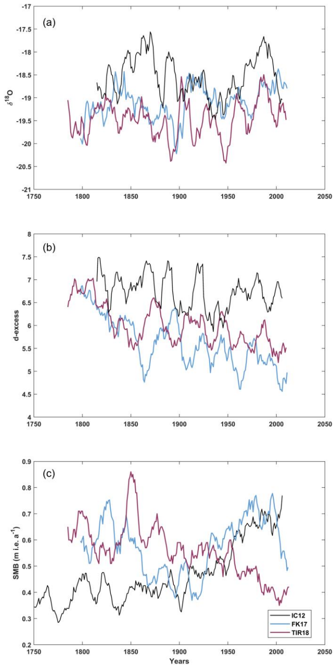
Figure C1G1. Comparison with IC12 (Philippe et al., 2016; Philippe and Tison, 2023). Note that these datasets have been smoothed using an 11-yr running mean. IC12 is in black, FK17 in blue and TIR18 in burgundy. (a) Annual mean \delta^{18}\text{O} signal. (b) Annual mean d-excess signal. (c) Surface mass balance corrected for vertical strain rates and expressed in \text{m i.e. a}^{-1} .
