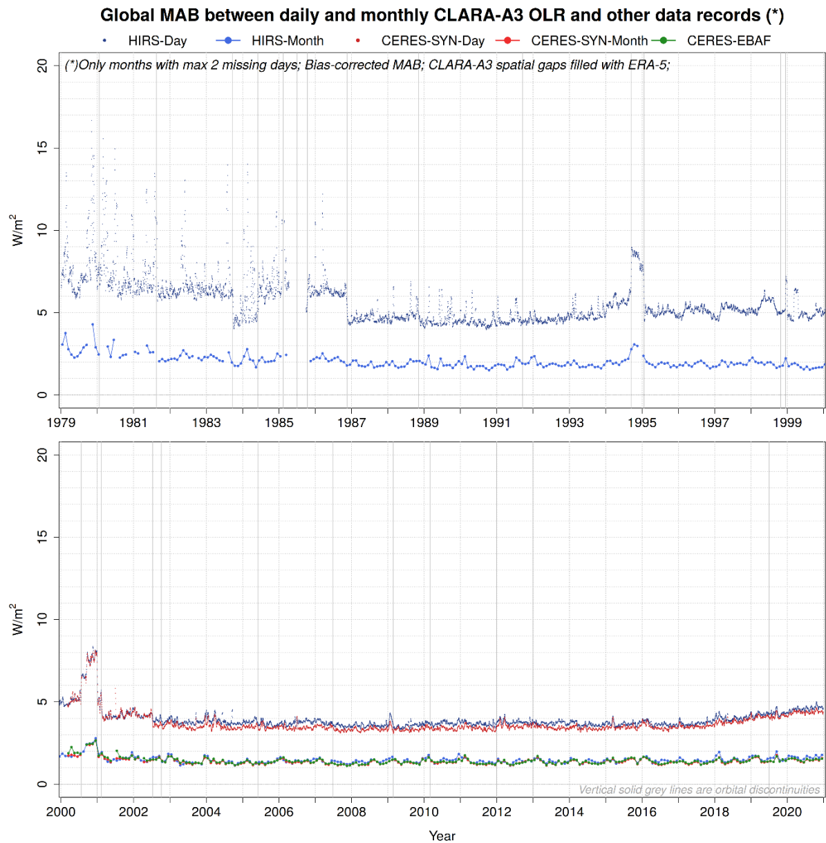
Figure 11: Global MAB between daily and monthly CLARA-A3 OLR and other data records. Daily MAB is systematically 2-3 Wm^{-2} higher compared to monthly MAB.
