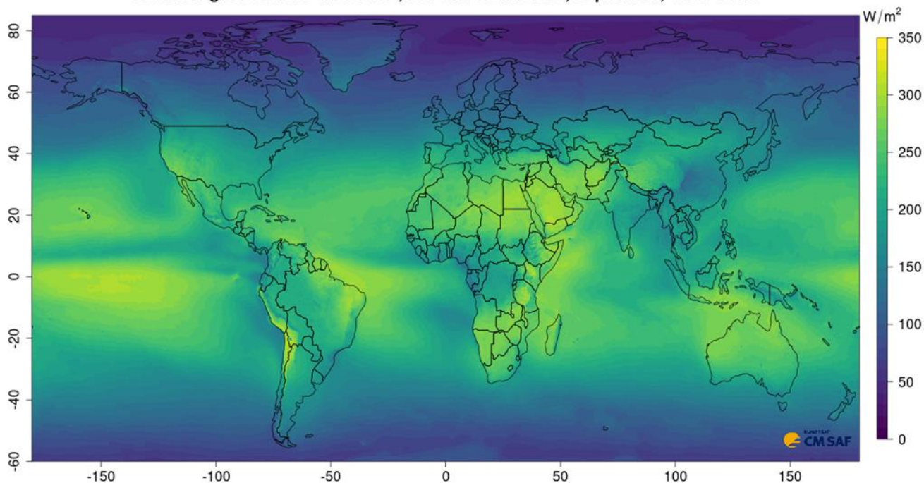
Climatological Surface Irradiance, CM SAF CLARA-A3, September, 1991 - 2020
