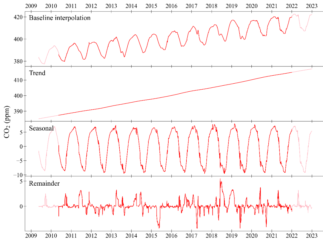
Figure S2: Time series decomposition of hourly averaged CO 2 mole fractions from WAO. The time series (2010-2021) was extended by a year both forwards and backwards in time (2009-2022) to minimize end effects. The top panel shows the data prior to decomposition, with the remainder, seasonal (detrended) and trend (deseasonalised) components plotted beneath respectively. ‘Remainder’ is calculated by subtracting both the seasonal and trend components from the baseline interpolated data. Vertical axis units are in ppm; the seasonal and remainder panels have been normalised to corresponding values of the long-term trend, which are denoted as 0 ppm. The decomposition was carried out using a curve fitting program called STL (see Sect. 2.3).
