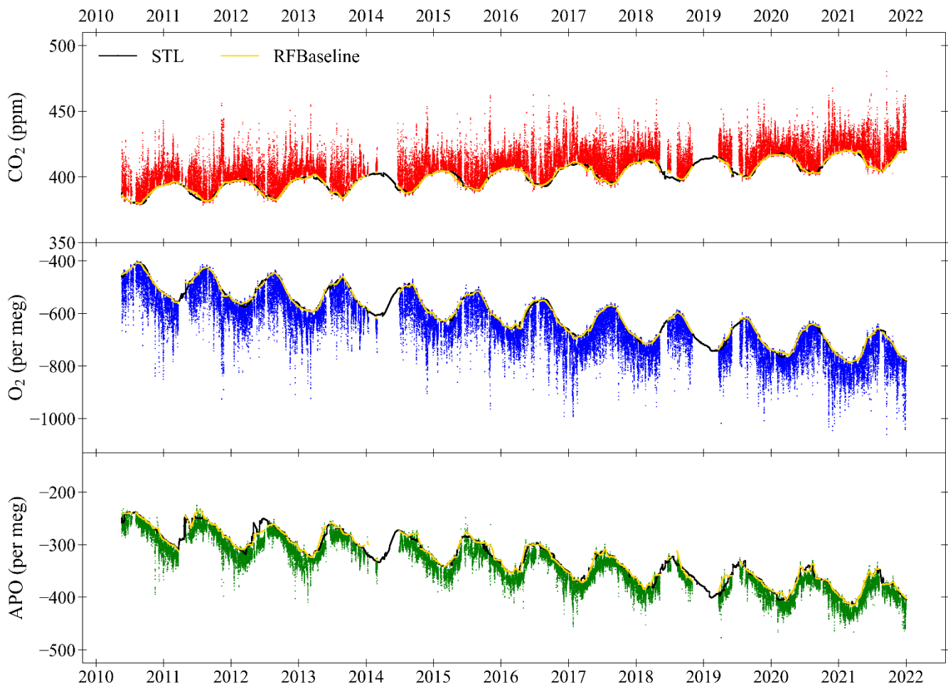
630 Figure 13: Hourly averaged \text{CO}_2 (top panel), \text{O}_2 (middle panel) and APO (bottom panel) at WAO between May 2010 and December 2021. The baselines (yellow lines) are fitted using the RFBaseline function of Ruckstuhl et al. (2012) and the curve fits (black lines) are calculated using the STL function in R (see Sect. 2.3). The \text{O}_2 and \text{CO}_2 y-axes are
