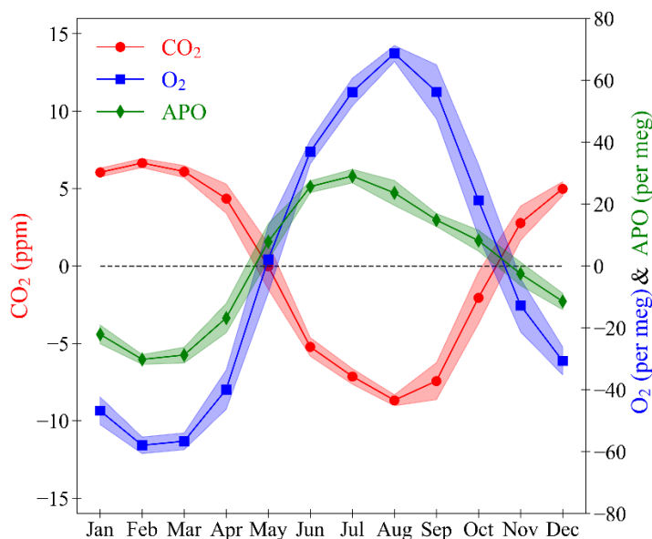
Figure 14: The seasonal cycles of CO 2 (red, left axis), O 2 (blue, right axis), and APO (green, right axis) at WAO. Individual points are the monthly means of the seasonal component of the STL decomposition (see Sect. 2.3). The shaded bands are the average of the \pm 1\sigma standard deviation of the monthly averages of the baseline data. The y-axes are scaled to be visually comparable on a mole per mole basis.
