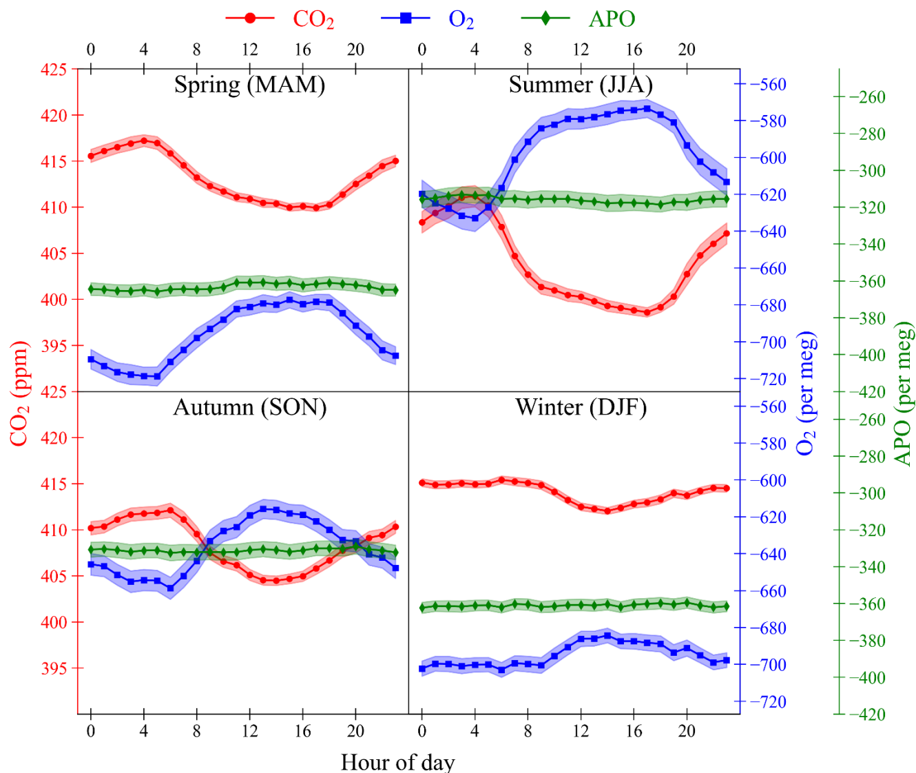
725 Figure 15: The diurnal cycles of CO 2 (red, left axis), O 2 (blue, right axis), and APO (green, right axis) at WAO for each season: spring (MAM), summer (JJA), autumn (SON), and winter (DJF). Individual points are calculated using the 2-minute data from May 2010 to December 2021, with the timeVariation function in the OpenAir package in R (Carslaw and Ropkins, 2012). The shaded bands are the average of the ±1σ standard deviation of the hourly averages of the data. The y-axes are scaled to be visually comparable on a mole per mole basis.
