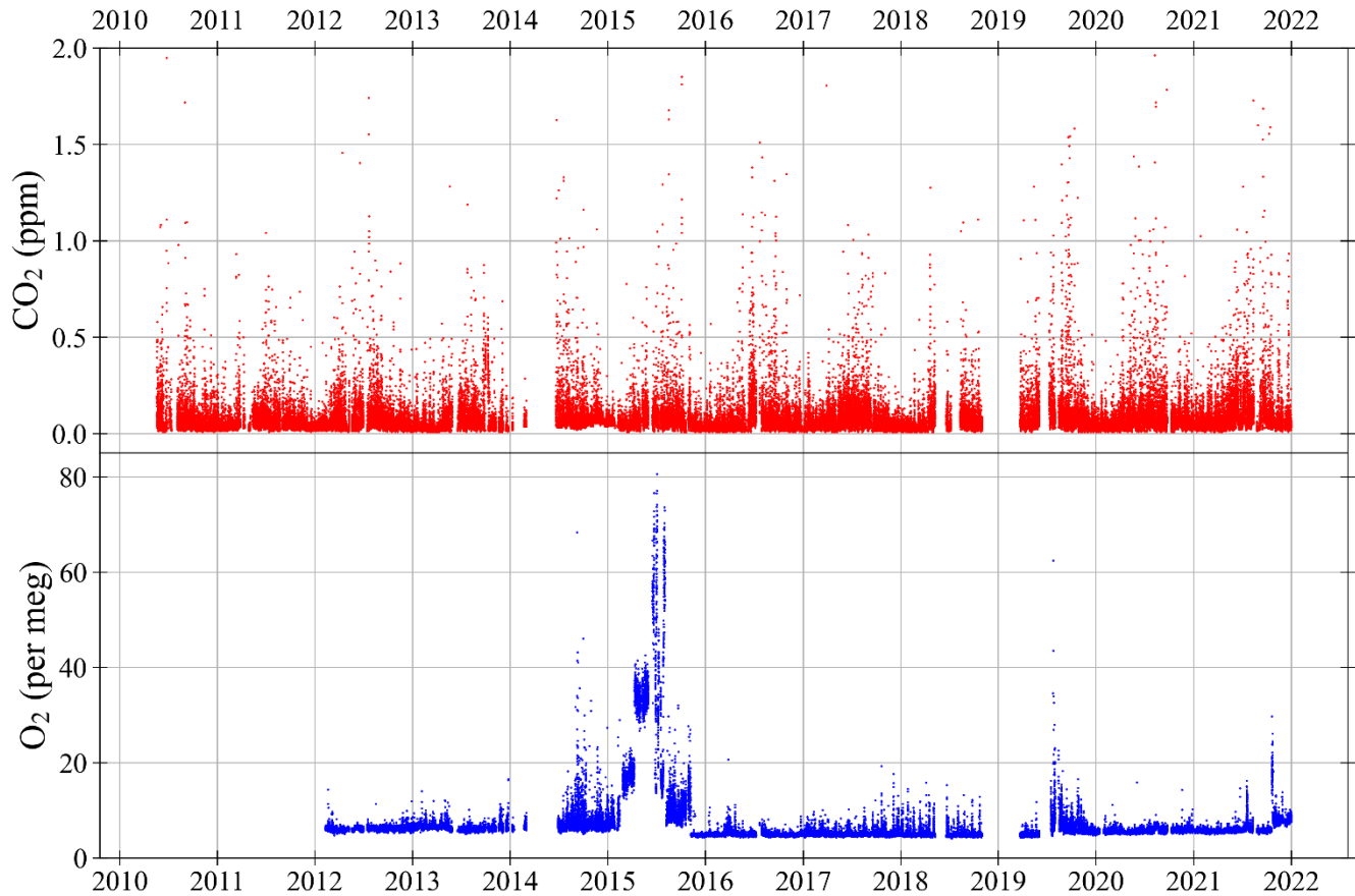
Figure 12: CO 2 (top panel) and O 2 (bottom panel) \pm 1\sigma standard deviation of air measurements at WAO between May 2010 and December 2021. The \pm 1\sigma standard deviations of the 2-minute data were not routinely calculated for O 2 until February 2012. Hourly averages of the \pm 1\sigma standard deviations of the 2-minute measurements. The O 2 y-axis is not visually comparable on a mole per mole basis to the CO 2 y-axis. Note that 4 measurements are off scale in the CO 2 panel, out of more than 70,000 measurements shown.
