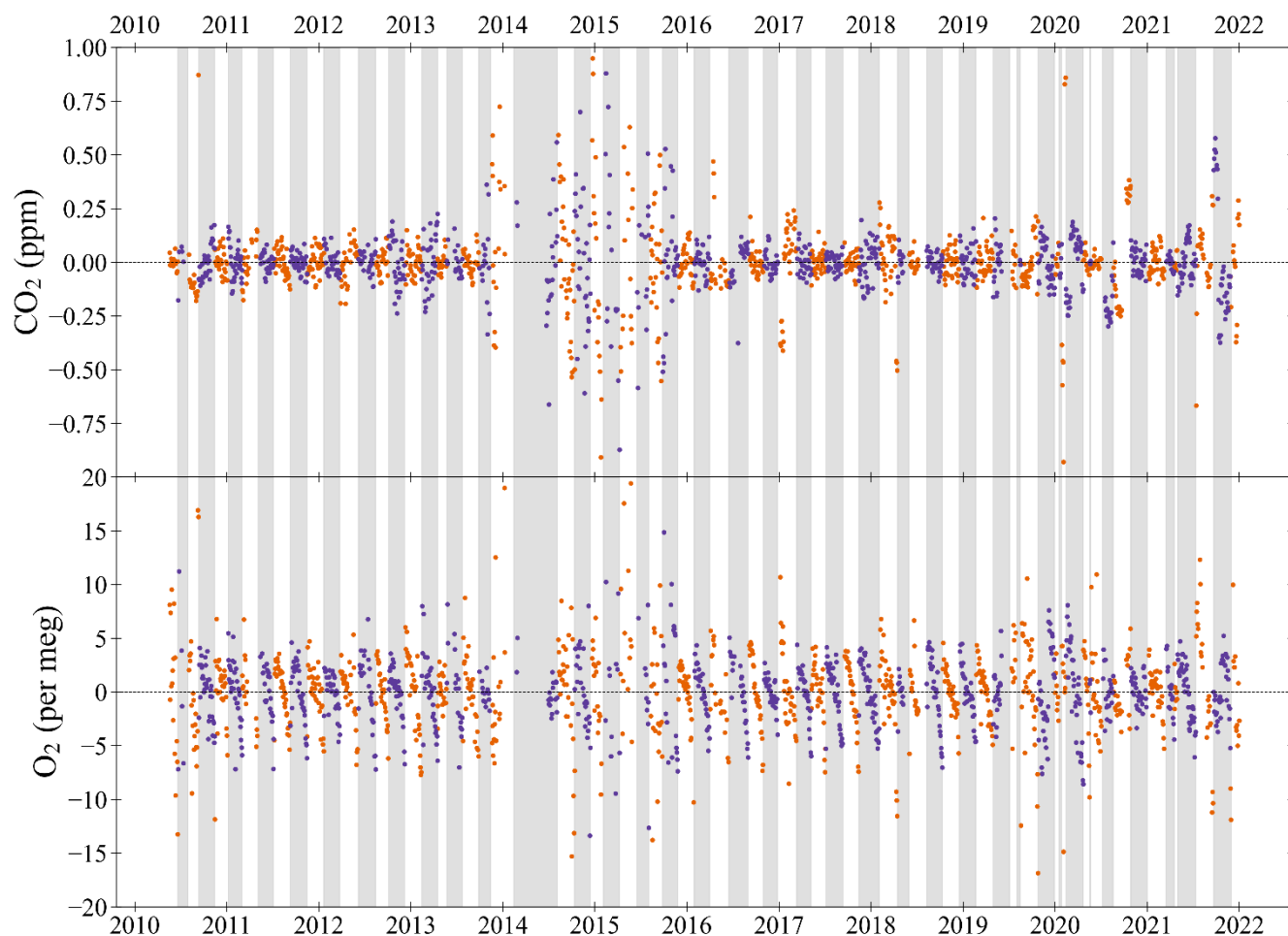
560 Figure 10: The CO 2 (top panel) and O 2 (bottom panel) Working Tank (WT) mole fractions calculated from the calibrations as the difference from the average mole fraction for each WT (measurement minus average) at WAO between May 2010 and December 2021. The WTs alternate between orange and purple, and alternate shaded grey bands, to show when the WT changes. On the y-axes 'zero' is the average mole fraction for each WT (dashed line). The O 2 y-axis is not visually comparable on a mole per mole basis to the CO 2 y-axis. Note that 5 and 7 measurements are off scale in the O 2 and CO 2 panels, respectively, out of more than 1700 measurements shown for each species.
