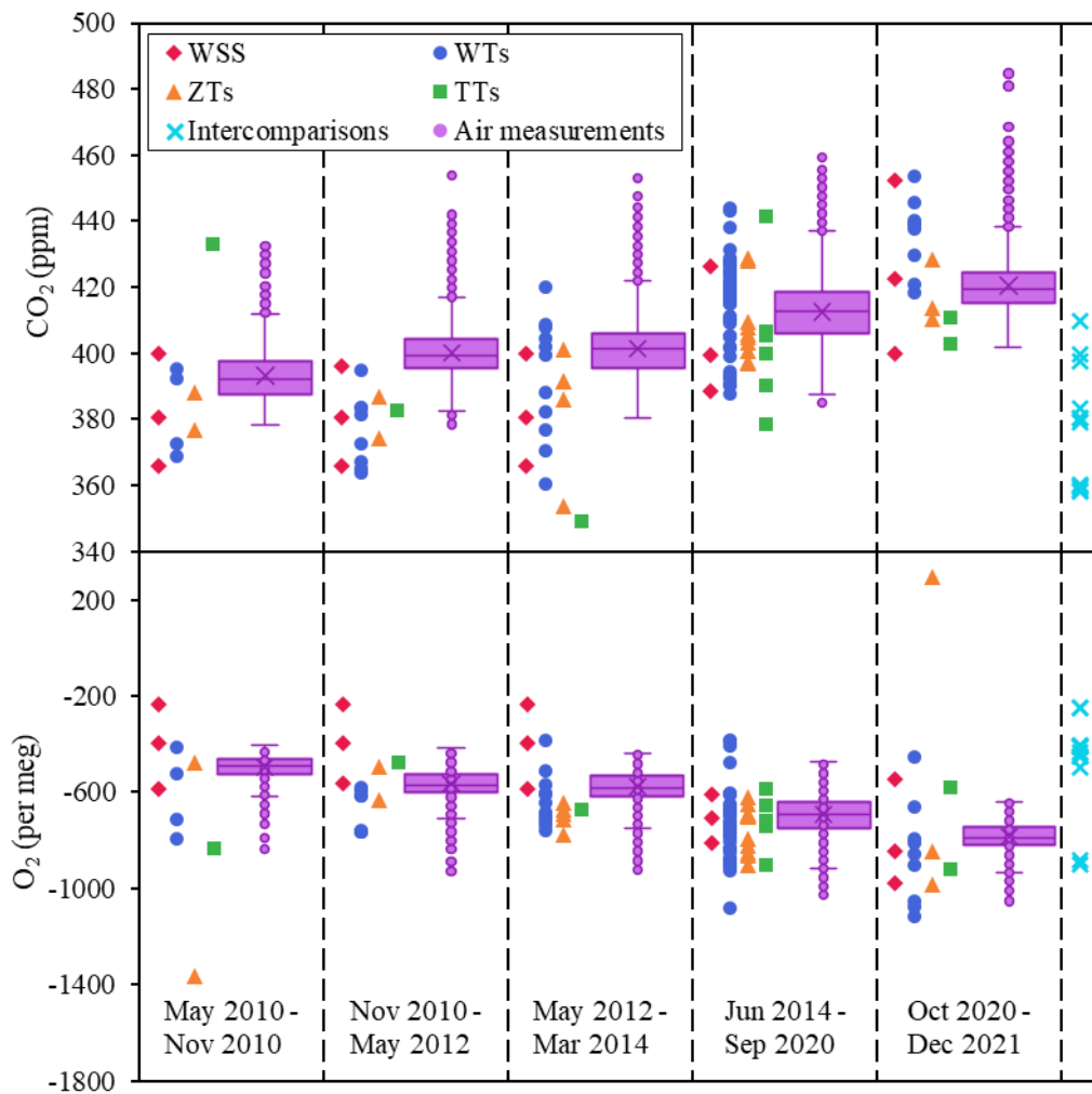
Figure 9: The CO_2 (top panel) and O_2 (bottom panel) mole fractions of the WSSes, WTs, ZTs, TTs and intercomparison cylinders measured at WAO between May 2010 and December 2021. The air measurements made at WAO during this time are shown as box and whisker plots. The O_2 y-axis is not visually comparable on a mole per mole basis to the CO_2 y-axis.
