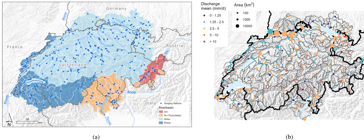
Figure 1. (a) Map of hydrologic Switzerland, covering political Switzerland and extending to neighbouring countries , with all gauging stations of CAMELS-CH and delineations of the four major river basins of Inn, Po, Rhine and Rhone; (b) Mean daily specific discharge and upstream catchment area at gauging stations (lake and river gauging stations with only water level recordings not shown-).
