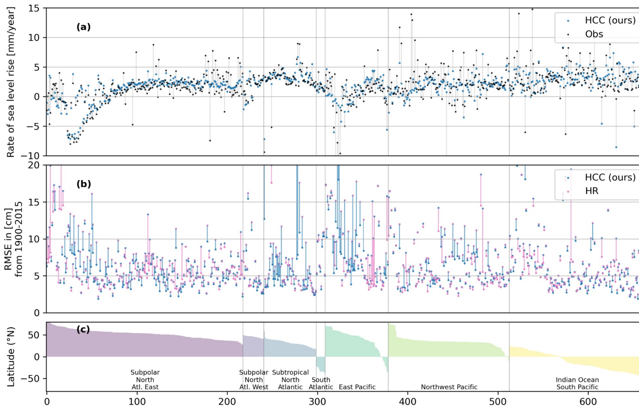
285 Figure 2: Performance of our HCC dataset and the HR dataset compared to tide gauges from the PSMSL record. Panel a: Linear sea level trend for years with valid observations for tide gauge records (black) and HCC (blue) connected by a gray bar. Panel b: RMSE between observed and modeled RSL as blue and pink dots for HCC and HR respectively. RMSE values for the same tide gauge station are connected with a blue bar if HCC has a lower RMSE than HR and with a pink bar if it is higher. Panel c: Latitude of tide gauge locations sorted by ocean basin. A progressive integer of the considered tide gauge is plotted on the x-axis. Outliers are not plotted.
