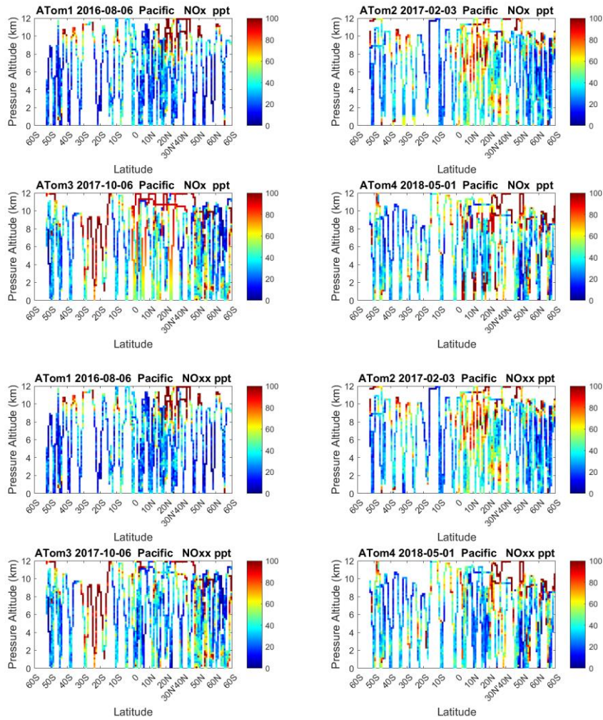
795 Figure 58. 2D Pacific curtain profiles for ATom-1234 of NOx (v2b) and NOxx (=NOx v3).
