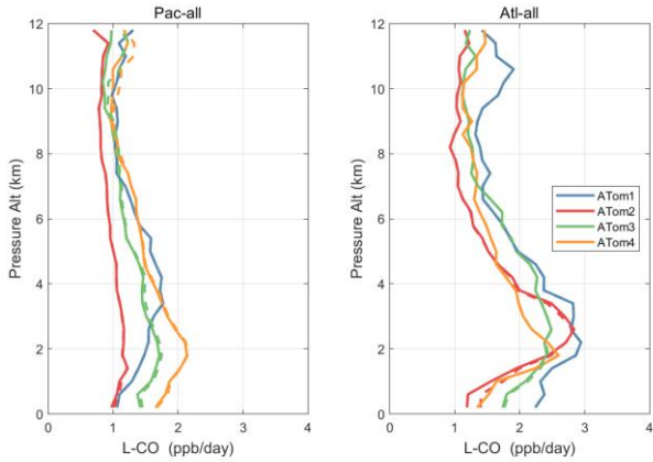
710 Figure 54. Altitude profiles of mean L-CO (ppb/d) over Pacific and Atlantic basin for ATom-1234. See Fig. 51. Compare with Fig. 32. Solid lines are MDS-3, and dashed lines are MDS-2b.
