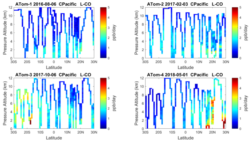
Figure 17. Curtain plots of L-CO (ppb/day) in the tropical Central Pacific (30°S-30°N) for ATom-1234. See Fig. 6.
