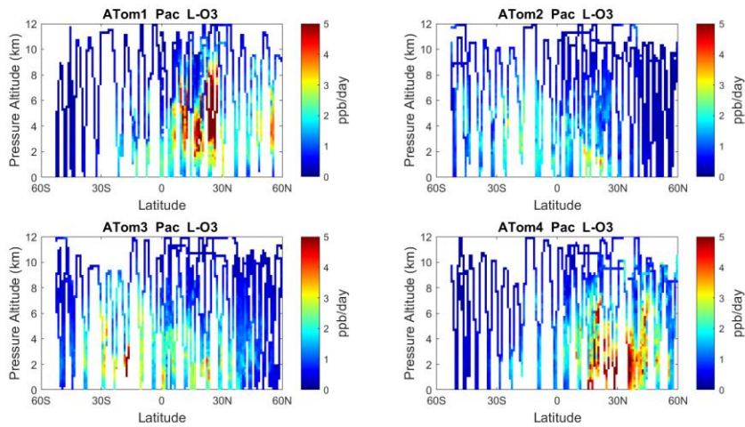
Figure 7. Curtain plots of L-O3 (ppb/day) in Pacific basin (53°S-60°N) for Atom ATom-1234. See Fig. 6
