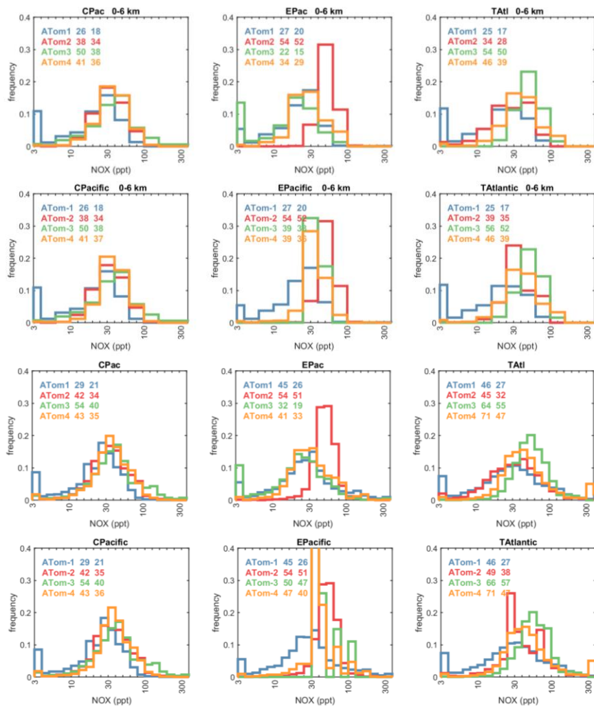
Figure 64. Probability Density of \log_{10}(\text{NO}_x, \text{ppt}) in the 3 tropical basins ( 30^{\circ}\text{S} - 30^{\circ}\text{N} ) for Atom ATom-1234, comparing MDS versions 3 and 2b. See Fig. 61. The numbers in the legend are, successively, the mean value of \text{NO}_x and the mean value of the \log_{10}(\text{NO}_x) , both in ppt. The 4 successive rows are: 0-6 km, MDS V3 and V2b; and 0-12 km, MDS V3 and V2b.
