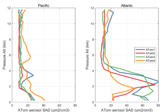
Figure 65. Vertical mean profiles of aerosol surface area density SAD ( \mu\text{m}^2 \text{cm}^{-3} ), over the Pacific and Atlantic basins. Standard weighting, see text. SAD is the sum of the four reported modes (nucleation, Aitken, accumulation, coarse) with most of the area from accumulation and coarse modes.
