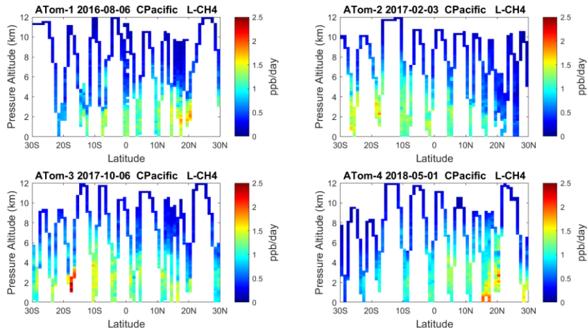
340 Figure 16. Curtain plots of L-CH 4 (ppb/day) in the tropical Central Pacific (30°S-30°N) for ATom-1234. See Fig. 6.
