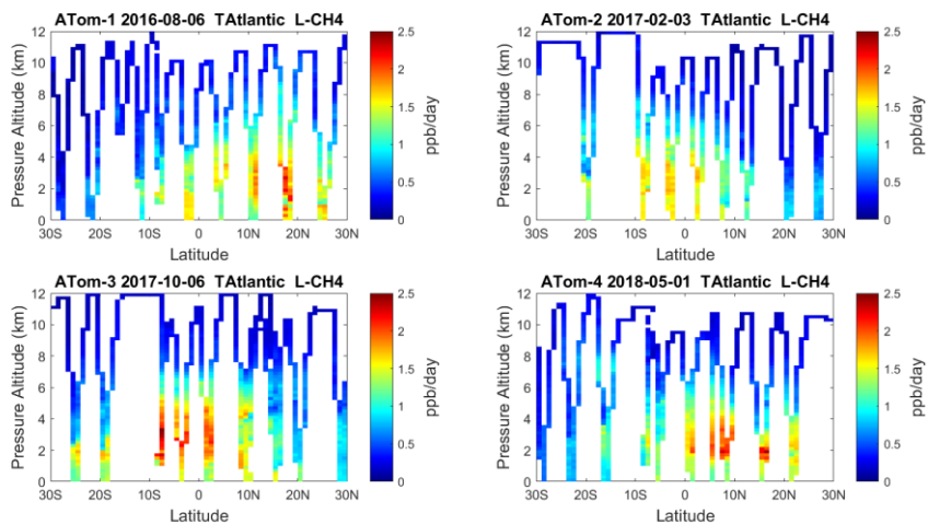
Figure 24. Curtain plots of L-CH 4 (ppb/day) in the tropical Atlantic (30°S-30°N) for ATom-1234. See Fig. 6.
