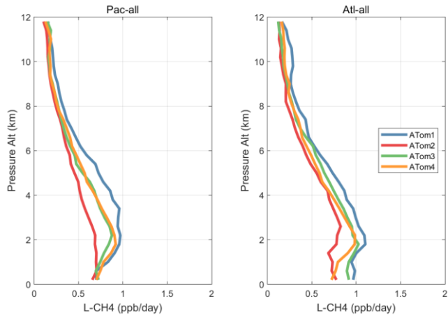
440 Figure 31. Mean altitude profile of L-CH4 (ppb/day) over the Pacific and Atlantic basins (53°S-60°N) for ATom-1234.
