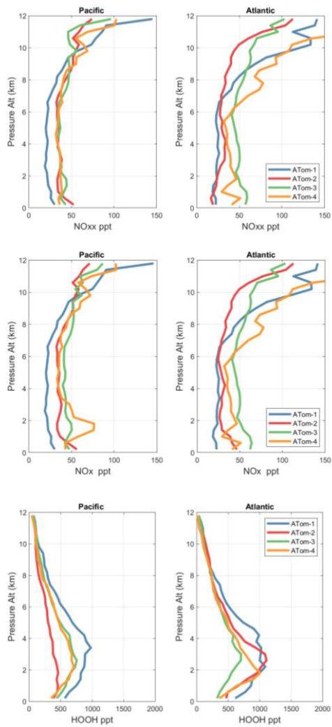
785 Figure 56. Vertical mean profiles (ppt vs pressure altitude) of NO x (v2b), NO xx (=NO x v3) and HOOH over the Pacific and Atlantic basins. Standard weighting, see text.
