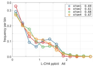
Figure 42. Probability Density of L-CH 4 (ppb/day) in Pacific and Atlantic basins for Atom ATom-1234. See Fig. 40.
