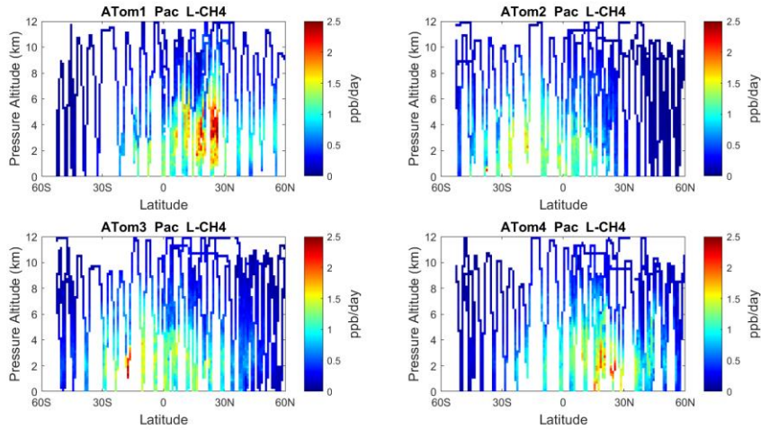
Figure 8. Curtain plots of L-CH 4 (ppb/day) in Pacific basin (53°S-60°N) for ATom1-1234. See Fig. 6
