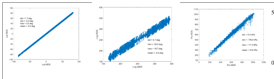
195 Figure 3. Comparison of the model grid cell value for pressure, latitude, and longitude used in the RDS calculation with those from the 32,383 10 s ATom-1 parcels (MDS). In each figure the standard deviation, minimum error, maximum error and mean error are shown. Values are specific to the UCI CTM with a T159L57 grid. These displacement errors occur because several 10 s parcels often occur within one CTM cell and must be shifted to nearby vacant cells.
