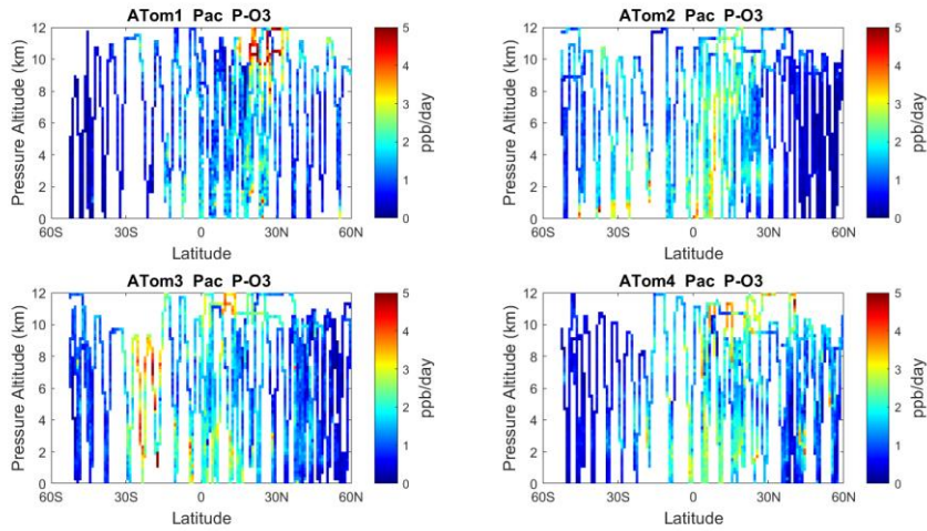
305 Figure 6. 2D curtain plots (altitude-latitude profiling) of P-O3 (ppb/day) in Pacific basin (53°S-60°N) for Atom ATom-1234. In all these curtain plots, ATom 10s parcel data are weighted by cosine (latitude) and sampling frequency, and then they are averaged into 1° latitude and 200 m altitude bins.
