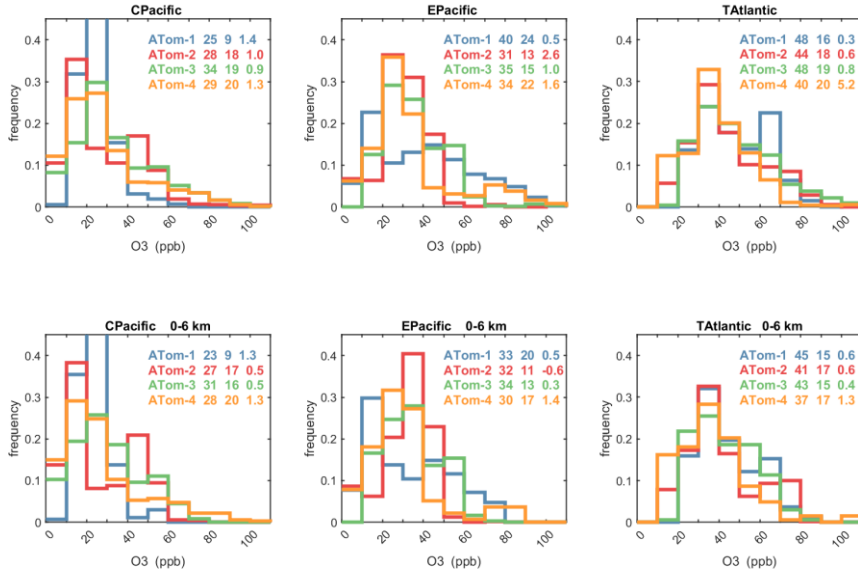
Figure 62. Probability Density of O 3 (ppb) in the 3 tropical basins (30°S-30°N) for ATom ATom-1234. See Fig. 61. The numbers in the legend are, successively, the mean value, standard deviation, and skewness in ppb.
