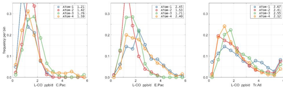
Figure 47. Probability Density of L-CO (ppb/day) in the 3 tropical basins for ATom-1234. See Fig. 40.
