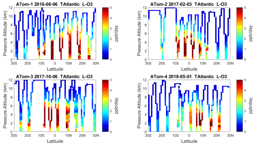
365 Figure 23. Curtain plots of L-O3 (ppb/day) in the tropical Atlantic (30°S-30°N) for ATom-1234. See Fig. 6.
