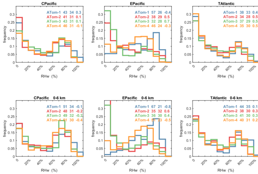
Figure 63. Probability Density of the relative humidity over liquid water (RHw, %) in the 3 tropical basins (30S-30N) for ATom-1, ATom-2, ATom-3, and ATom-4. See Fig. 61. The numbers in the legend are, successively, the mean value, standard deviation, and skewness in %.
