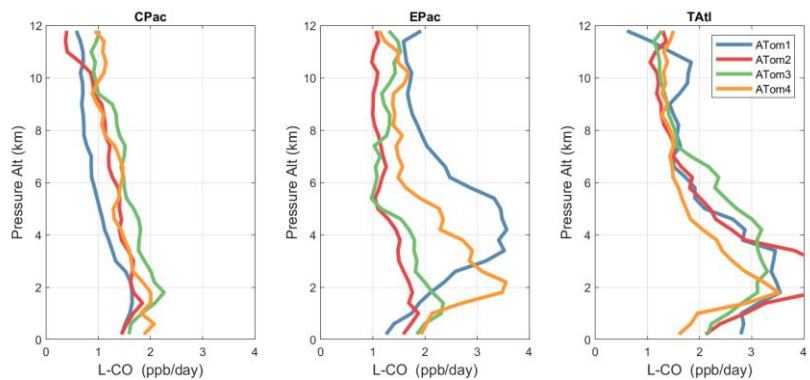
Figure 36. Mean altitude profile of L-CO (ppb/day) over the 3 tropical basins for ATom-1234.
