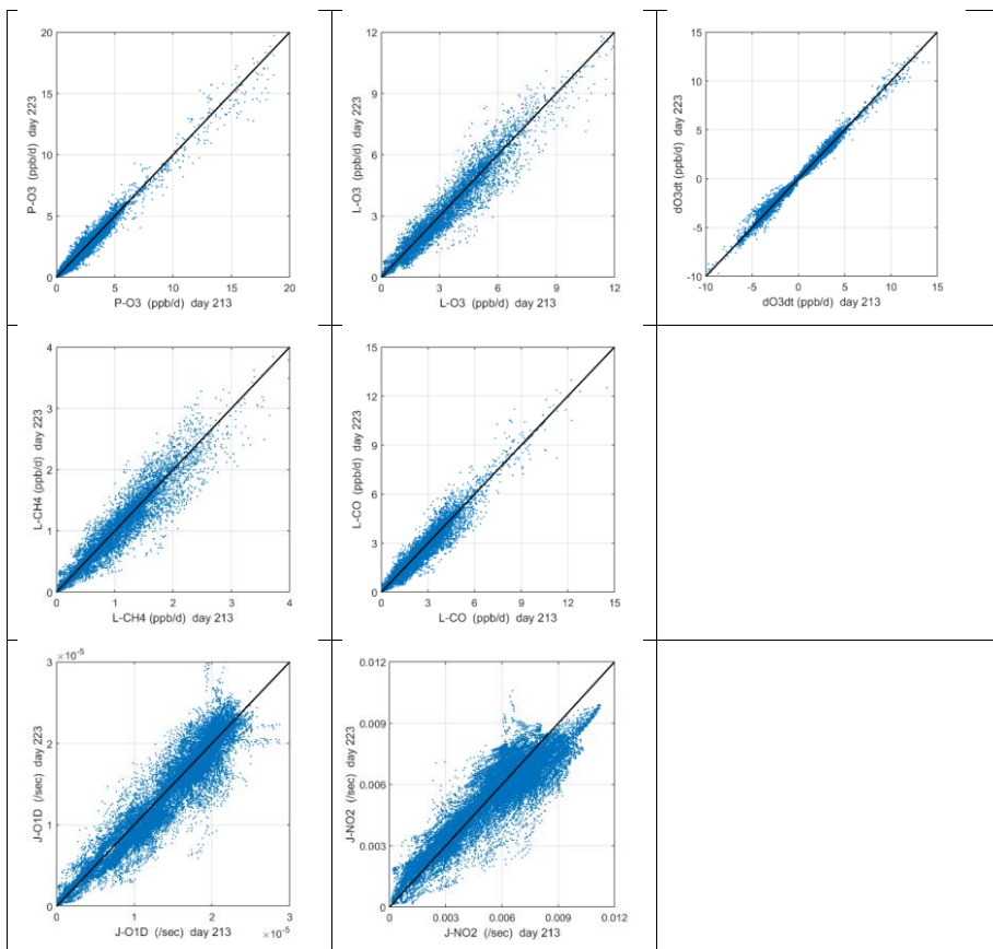
Figure 4. Reactivities (ppb/b) and J-values (/sec) calculated for all 32,383 ATom-1 10 s parcels using two different days with different cloud fields and ozone columns. The net integrated ozone change over the day, dO_3/dt (ppb/d), is also shown. Day 213 = August 1 and day 223 = August 11. Mean reactivity statistics here are calculated as the mean of five days (August 1, 6, 11, 16, 21), while sensitivity analyses used only day 223.
