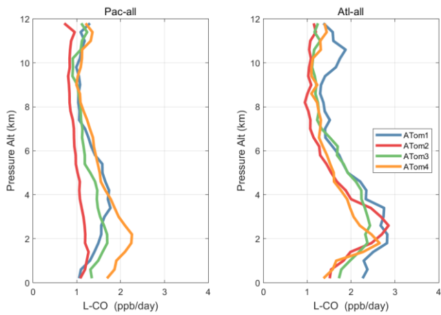
445 Figure 32. Mean altitude profile of L-CO (ppb/day) over the Pacific and Atlantic basins (53°S-60°N) for ATom-1234.
