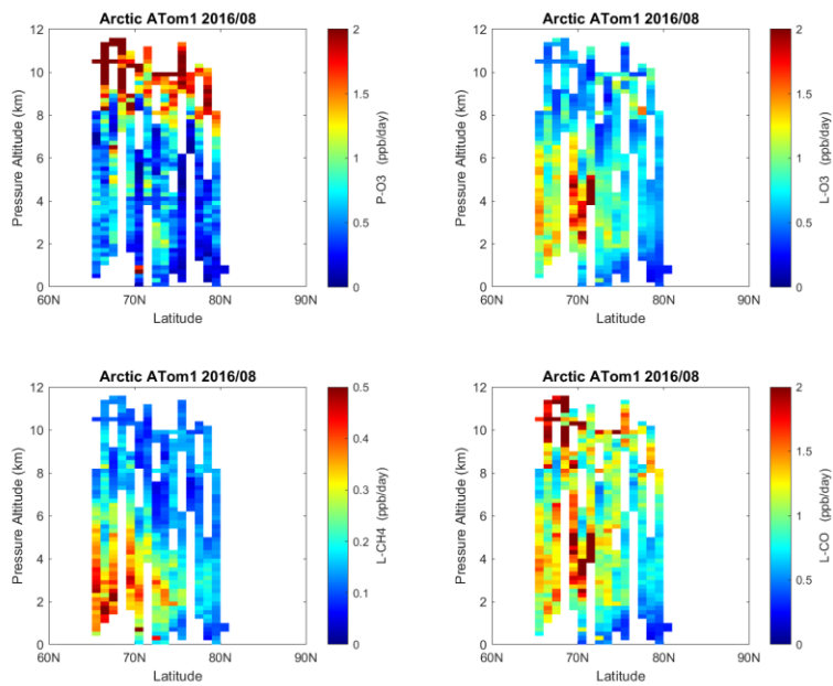
Figure 26. Curtain plots of the 4 reactivities (P-O 3 , L-O 3 , L-CH 4 , L-CO ppb/day) over the Arctic for ATom-1. Note the color bars have a much smaller range than in the Pacific and Atlantic basin plots. Troposphere-only parcels are shown, with stratosphere defined as (H 2 O < 30 ppm) and (O 3 > 80 ppb) and (CO < 120 ppb). See Fig. 6.
