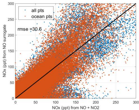
Figure 50. Scatter plot of NOx using NO as a surrogate ( \text{NOx} = 2.055 \times \text{NO} , y-axis) and directly measured NOx (x-axis) for all ATom parcels where \text{NO}_2 is measured. The red points are all ocean basin parcels; and the blue points are all others. The 1:1 black line is for reference.
