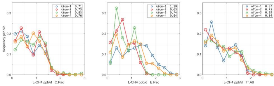
Figure 46. Probability Density of L-CH4 (ppb/day) in the 3 tropical basins for ATom-1234. See Fig. 40.
