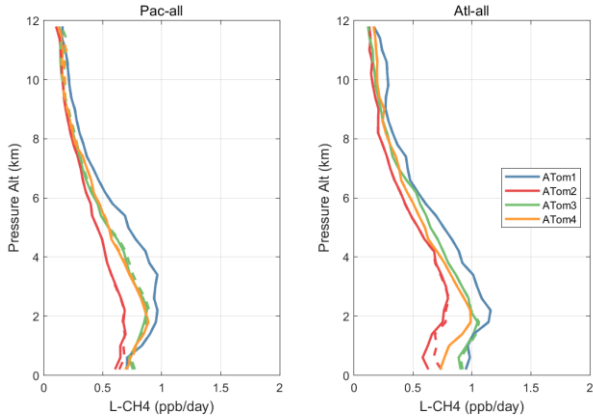
705 Figure 53. Altitude profiles of mean L-CH 4 (ppb/d) over Pacific and Atlantic basin for ATom-1234. See Fig. 51. Compare with Fig. 31. Solid lines are MDS-3, and dashed lines are MDS-2b.
