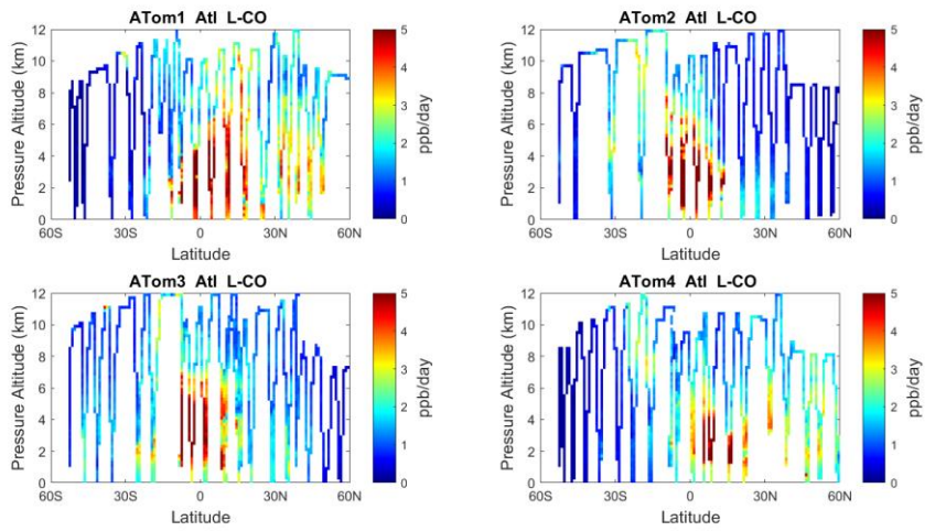
330 | Figure 13. Curtain plots of L-CO (ppb/day) in Atlantic basin (53°S-60°N) for ATom ATom-1234. See Fig. 6.
