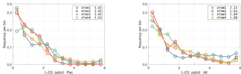
Figure 41. Probability Density of L-O3 (ppb/day) in Pacific and Atlantic basins for ATom-1234. See Fig. 40
