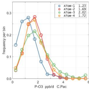
Figure 44. Probability Density of P-O 3 (ppb/day) in the 3 tropical basins (30°S-30°N) for Atom ATom-1234. See Fig. 40.
