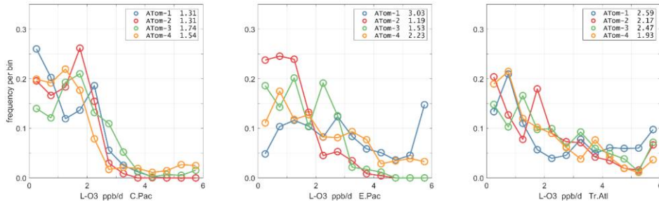
Figure 45. Probability Density of L-O3 (ppb/day) in the 3 tropical basins for ATom-1234. See Fig. 40.
