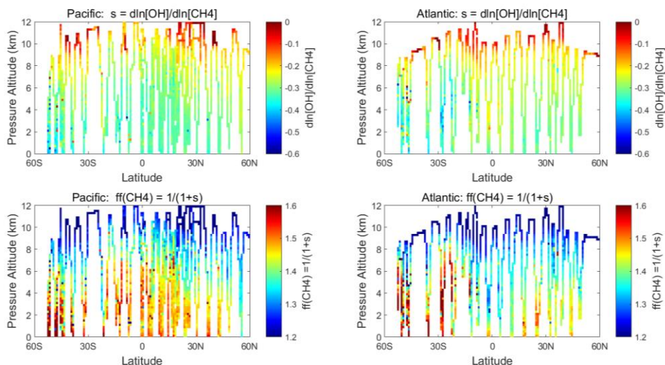
1015 Figure 70. 2D curtain plots from ATom-1 of (top) the OH sensitivity to CH 4 , s_{\text{OH}} = \text{dln}[\text{OH}]/\text{dln}[\text{CH}_4] = \text{dln}[\text{L-CH}_4]/\text{dln}[\text{CH}_4] - 1 , for 1020 Pacific and Atlantic basins, and (bottom) the CH 4 lifetime feedback factor, \text{ff}_{\text{CH}_4} = 1/(1+s_{\text{OH}}) for the same.
