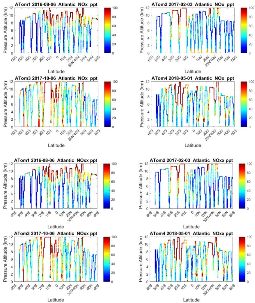
800 Figure 59. 2D Atlantic curtain profiles for ATom-1234 of NOx (v2b) and NOxx (=NOx v3).
