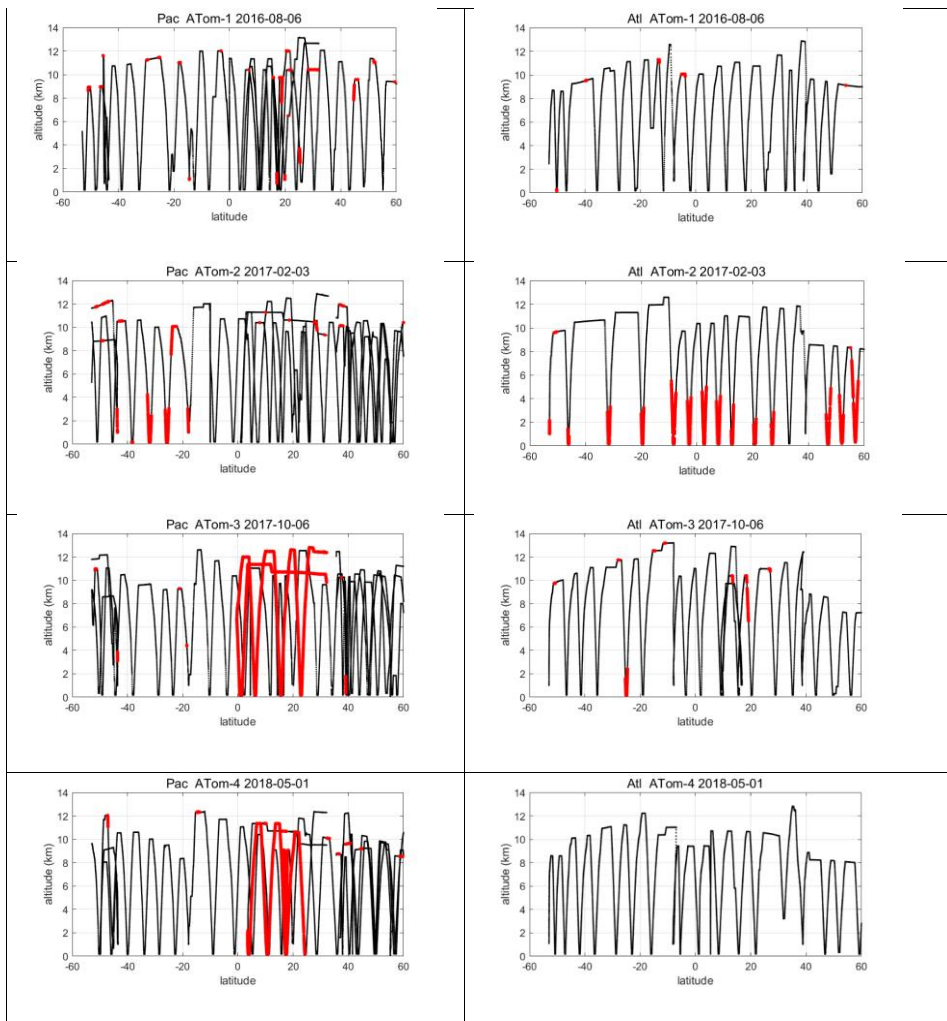
Figure 49. ATom-1234 profiling in Pacific and Atlantic basins showing parcels (large red dots) where \text{NO}_2 observations are missing, where long-gap interpolation was used in MDS version 2b, and where shifting to \text{NO}_x^{\text{fit}} based on \text{NO} observations in MDS version 3 results in a change in \text{NO}_x of >1 ppt.
