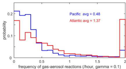
920 Figure 66. Frequency distribution of gas-aerosol reactions (per hour) for ATom-1 Pacific (blue) and Atlantic (red) assuming a high reactivity coefficient \gamma = 0.10 .
