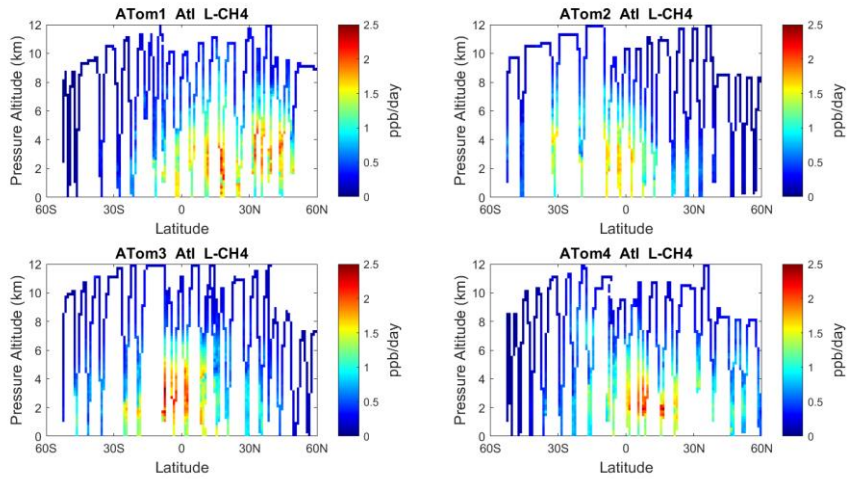
325 | Figure 12. Curtain plots of L-CH 4 (ppb/day) in Atlantic basin (53°S-60°N) for ATom ATom-1234. See Fig. 6.
