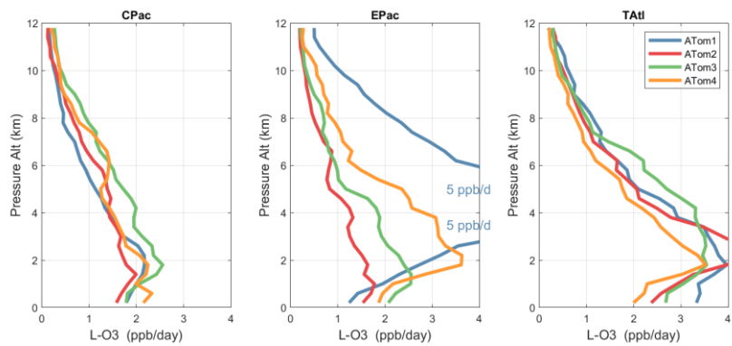
450 Figure 34. Mean altitude profile of L-O3 (ppb/day) over the 3 tropical basins for ATom-1234.
