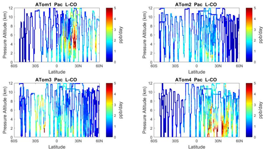
Figure 9. Curtain plots of L-CO (ppb/day) in Pacific basin (53°S-60°N) for ATom1-1234. See Fig. 6
