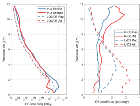
970 Figure 68. (left) O 3 loss frequency (/day) versus pressure altitude (km), averaged over Pacific (blue) and Atlantic (red) basins for ATom-1. True linearized loss frequency ( 1/T^1 , solid lines) is compared with the often-used approximation ( 1/T^A = L-O_3/O_3 , dashed lines). (right) Altitude profiles for both ocean basins of P-O 3 (solid) and L-O 3 (dashed), both in ppb/d.
