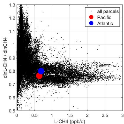
1010 Figure 69. Sensitivity of CH 4 loss with respect to its abundance (dln[L-CH 4 ]/dln[CH 4 ], in % per %) versus loss rate (L-CH 4 , in ppb/d) for parcels in ATom-1. All ATom-1 10 s parcels, including continental data, are plotted (small black dots) as well as the basin-mean values for Pacific (red dot) and Atlantic (blue dot).
