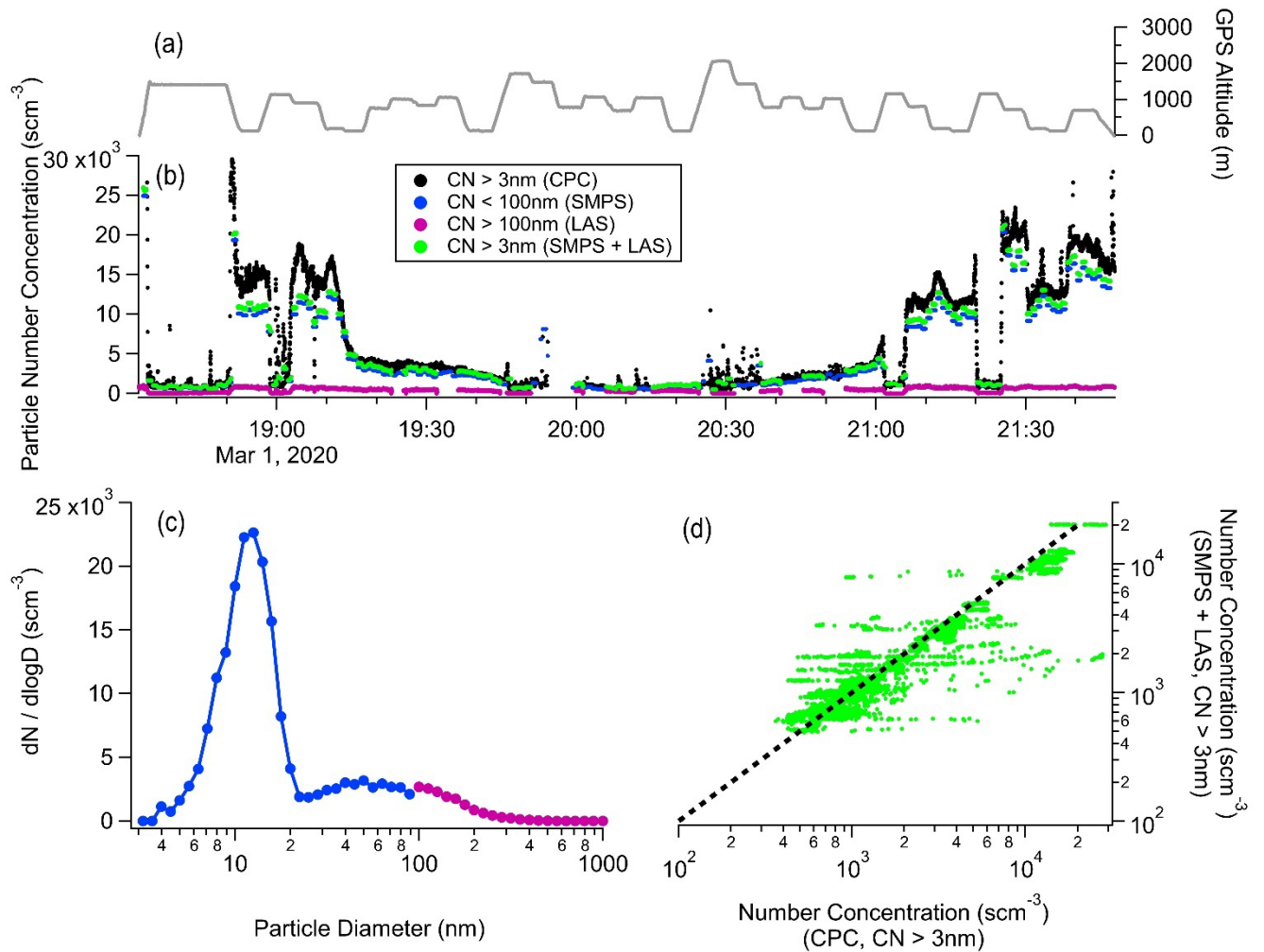
Figure S1: Closure analysis for particle number concentration measurements derived from an ultrafine CPC, SMPS, and LAS. (a-b) Timeseries data are shown for Research Flight 14 (1 March 2020), (c) an average size distribution during a MinAlt leg at approximately UTC 21:17, and (d) a scatterplot of the integrated number concentration derived from LAS+SMPS instruments against number concentration directly measured by a CPC.
