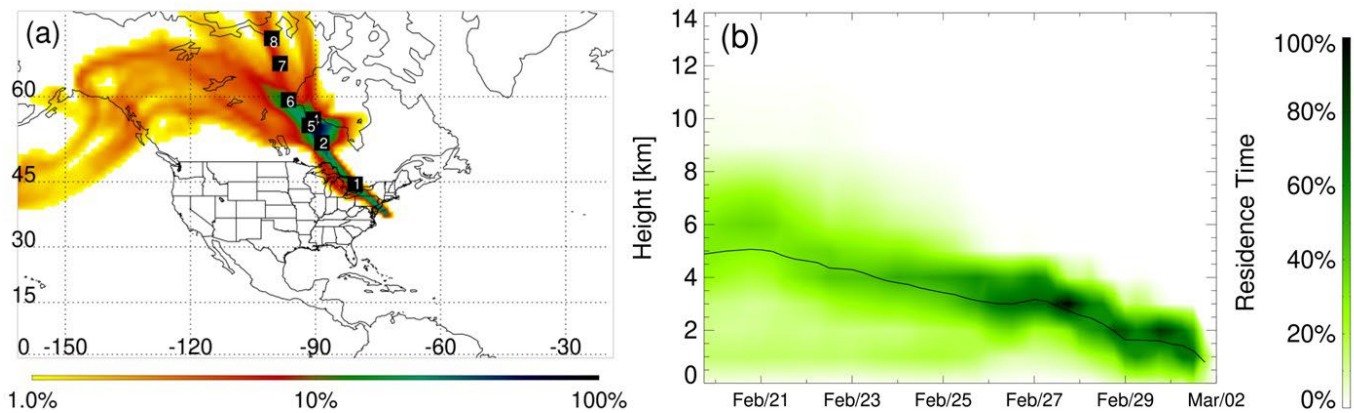
1575 Figure 8: (a) Horizontal and (b) vertical views of simulated air mass residence time (RT) for flight measurements at 19:22 1580 UTC on 1 March 2020 (RF14). The labels with white numbers on the map in (a) indicate the locations of maximal RT for the corresponding upwind day. Transport pathways differ significantly, and absolute RT values may vary a lot between cases. For a better comparison of transport pathways between cases, RT is expressed as a percentage of the maximal integrated value during the 10-day trajectory period. RT is color-coded with (a) logarithmic and (b) linear scales, respectively.
