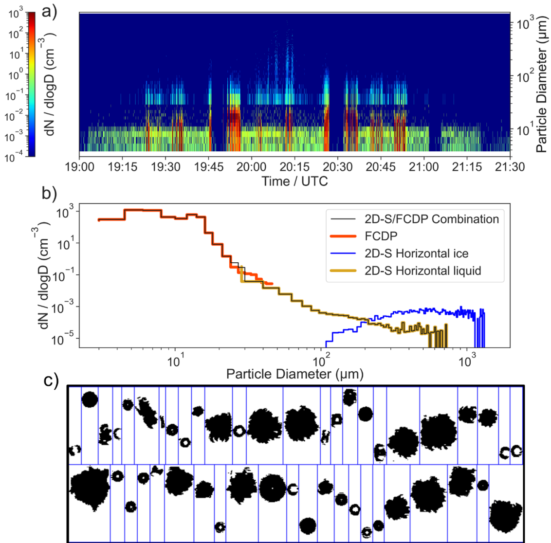
1615 Figure 12: Representative data products derived from FCDP and 2D-S on the Falcon for RF14 on 1 March 2020. (a) Time series of cloud droplet size distribution for RF14 on 1 March 2020 based on combining FCDP and 2D-S data, (b) average size distribution of liquid (FCDP and 2D-S Horizontal) and ice (2D-S Horizontal) for cloud measurements with LWC > 0.02 \text{ g m}^{-3} and N_d > 10 \text{ cm}^{-3} , and (c) example images captured by the 2D-S Horizontal probe for UTC 20:05:35 – 20:05:50.
