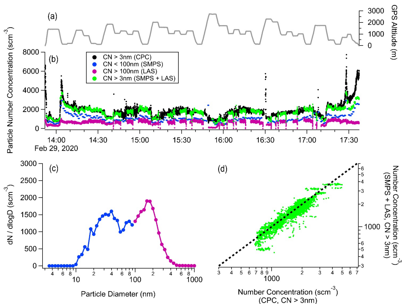
Figure 7: Closure analysis for particle number concentration measurements derived from an ultrafine CPC, SMPS, and LAS. 1565 (a-b) Time series data are shown for Research Flight 12 on 29 February 2020, (c) an average size distribution (SMPS in blue and LAS in magenta) during a BCB leg at approximately UTC 16:15 (bottom left), and (d) a scatterplot of the integrated number concentration derived from LAS+SMPS instruments against number concentration directly measured by a CPC. Units of \text{scm}^{-3} represent standard \text{cm}^{-3} . For panel d, orthogonal distance regression (ODR) linear fitting resulted in a slope of 0.961, intercept of -1.07 \text{ cm}^{-3} , and coefficient of determination ( r^2 ) of 0.868. Mean absolute error (MAE) and mean absolute percentage error (MAPE) values of 148 \text{ cm}^{-3} and 8.45%, respectively, are well within stated uncertainties in Table 5 and 1570 demonstrate excellent measurement closure.
