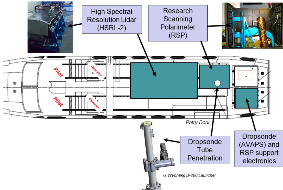
1535 Figure 4: King Air interior layout.
