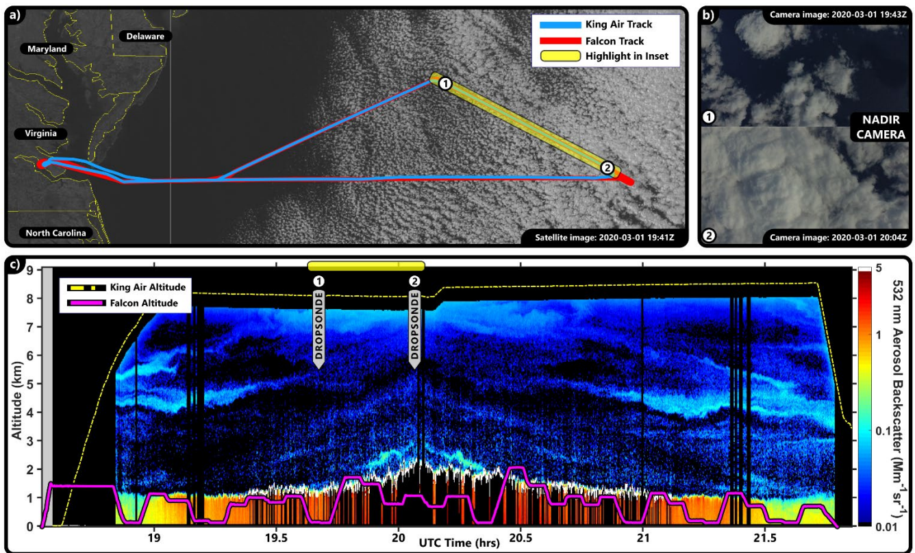
1585 Figure 9: (a) Flight tracks of the King Air and HU-25 Falcon on RF14 on 1 March 2020 overlaid on GOES-16 visible imagery captured at UTC 19:41. The number 1 and 2 labels correspond to where the two dropsondes were launched along the downwind leg (highlighted in yellow) during this flight. These indicators are consistent in all three panels. (b) Nadir camera imagery from the King Air at the time the two dropsondes were launched. (c) Time series of the King Air aerosol backscatter shown as curtain profiles, along with the altitude trace of the King Air and Falcon aircraft. Shown also are the locations of where the 1590 two dropsondes were launched and the downwind leg is highlighted in yellow.
