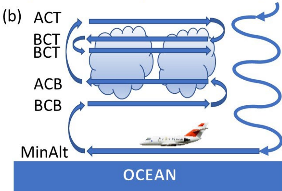
1530 Figure 3: (a) Visual summary of Research Flight 13 (1 March 2020, L1) tracks for both the (yellow) Falcon and (red) King Air overlaid on GOES-16 imagery (UTC 15:21). Highlighted in the flight is a “delay loop” (described in sect. 2.4) executed by the Falcon to improve coordination with the King Air. (b) The generic Falcon pattern used in process study flights including stacked level legs (“wall”) with spiral soundings before and after the wall; meanwhile the King Air (not shown in panel b) flies aloft characterizing the same area. In this flight, in place of a spiral sounding at the end of a wall, the Falcon conducted a slant descent from the last BCT leg to a subsequent MinAlt leg.
