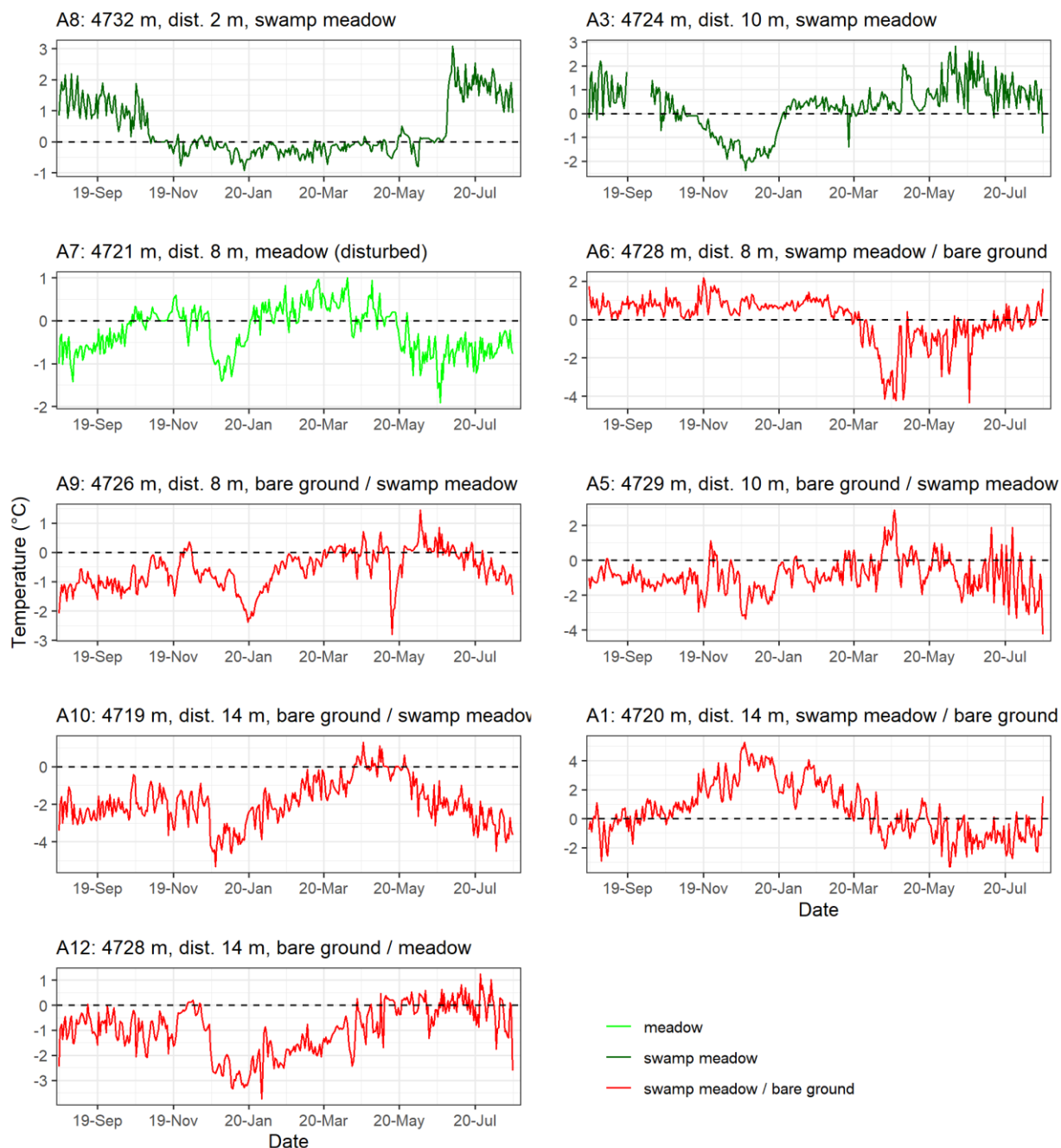
225 Figure 3. Intra-plot differences in daily ground surface temperatures (GST) for period August 2019 – July 2020 at sites at the local scale (2 km 2 ) on the Chalaping peat plateau in the south-central HAYR.
