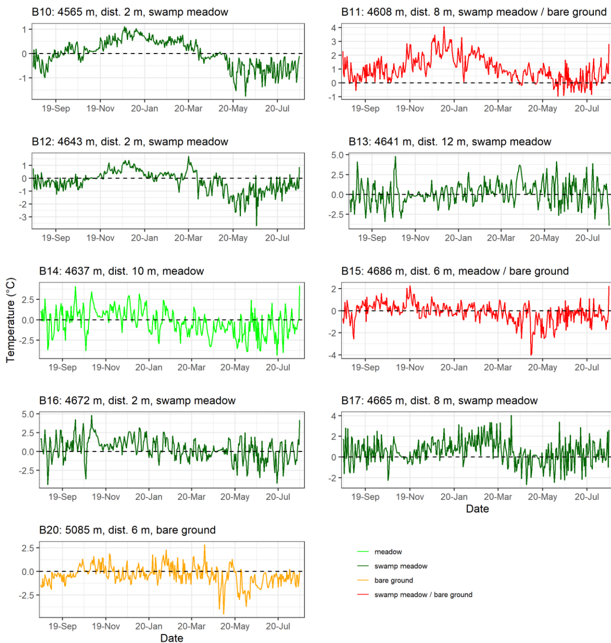
250 Figure 6. Intra-plot differences in daily ground surface temperatures (GST) for period August 2019 – July 2020 in sites B10 to B20 along the elevational transect in the south-central HAYR.
