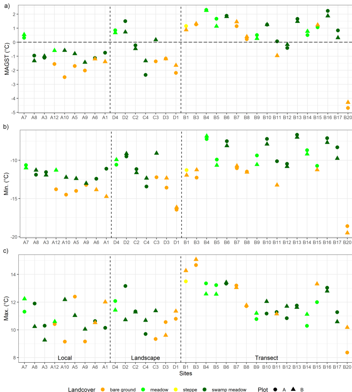
285 Figure 8. Mean annual ground surface temperature (MAGST) (a), the minimum GST (b), and the maximum GST (c) for the period August 2019 to July 2020 in both plots A and B of each site in south-central HAYR. Local scale ( 2\text{ km}^2 ), Landscape scale ( 50\text{ km}^2 ), and Elevational transect ( 800\text{ m} difference).
