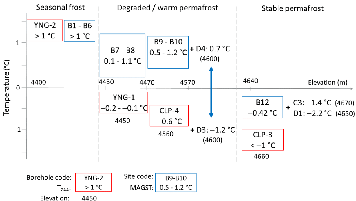
380 Figure 10. Comparison of the mean annual ground surface temperature (MAGST) for the period August 2019 to July 2020 in south-central HAYR with the multi-year (2010-2017) average temperatures at the depth of zero annual amplitude ( T_{ZAA} ) at depths of 10 and 15 m. Boreholes data are from Luo et al. (2018b). T_{ZAA} = Temperatures at the depth of zero annual amplitude (10 to 15 m).
