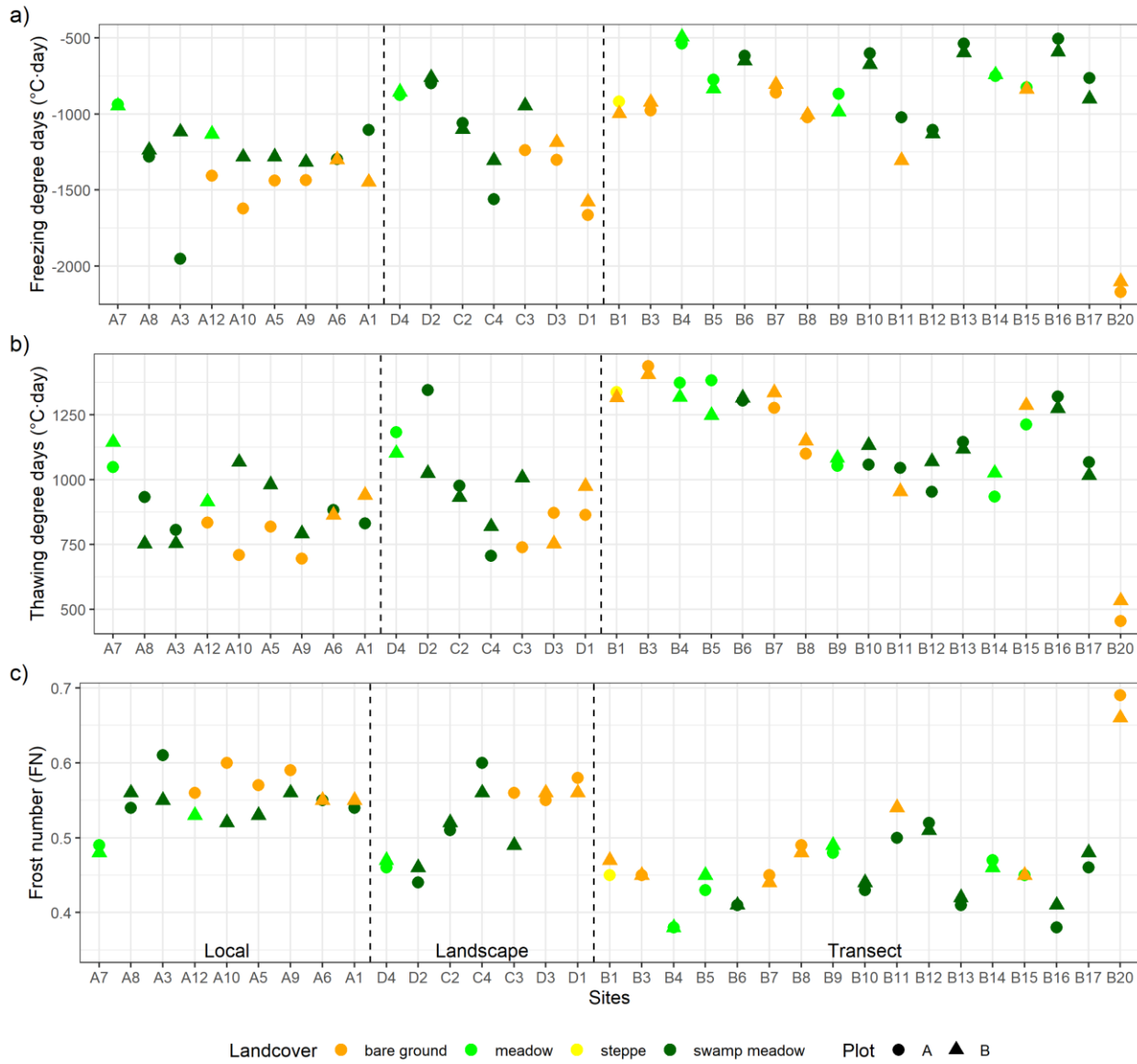
Figure 9. Freezing degree days (a), thawing degree days (b), and the frost number (c) at the depth of the ground surface temperature, approximately 5 cm into the ground, for the period August 2019 to July 2020 in both plots (A and B) of each site in south-central HAYR. Local scale (2 km 2 ), Landscape scale (50 km 2 ), and Elevational transect (800 m difference).
