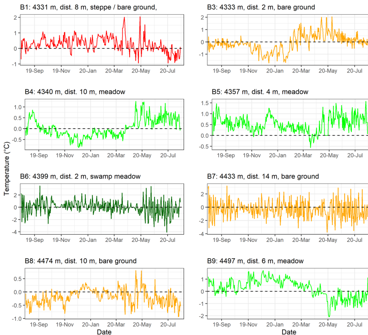
Figure 5. Intra-plot differences in daily ground surface temperatures (GST) for period August 2019 – July 2020 in sites B1 to B9 along the elevational transect in the south-central HAYR.
