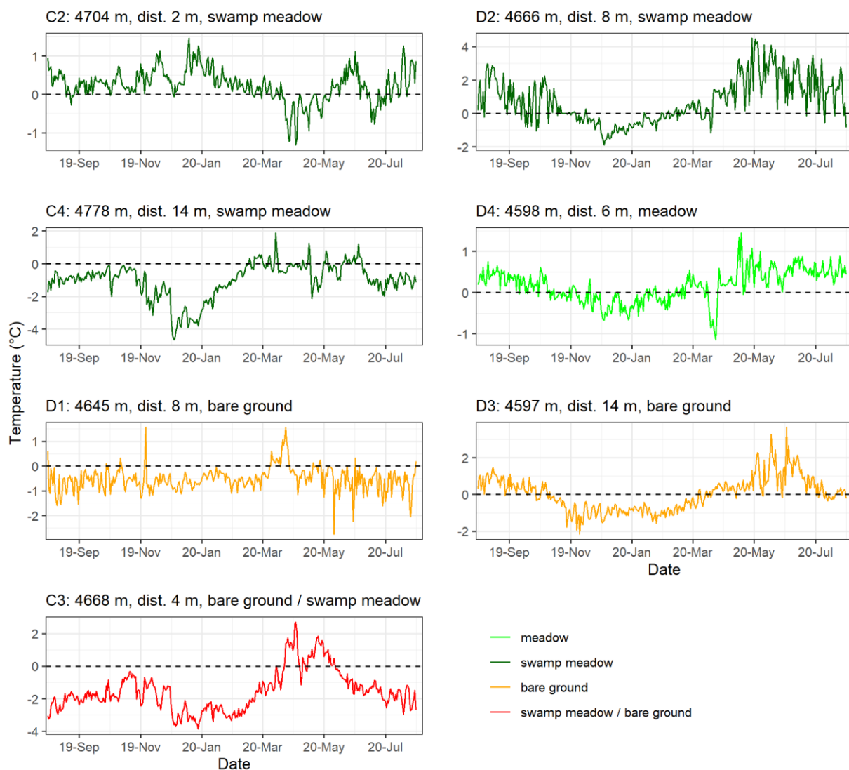
Figure 4. Intra-plot differences in daily ground surface temperatures (GST) for period August 2019 – July 2020 in sites at the landscape scale (50 km 2 ) on the Chalaping peat plateau in the south-central HAYR.
