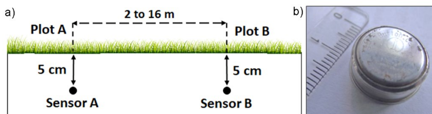
140 Figure 2. The schematic draw with the monitoring of GST at the fine-scale: the position of the two plots at distances from 2 to 16 m (a). Photo of the iButton temperature logger DS1922L (b).
