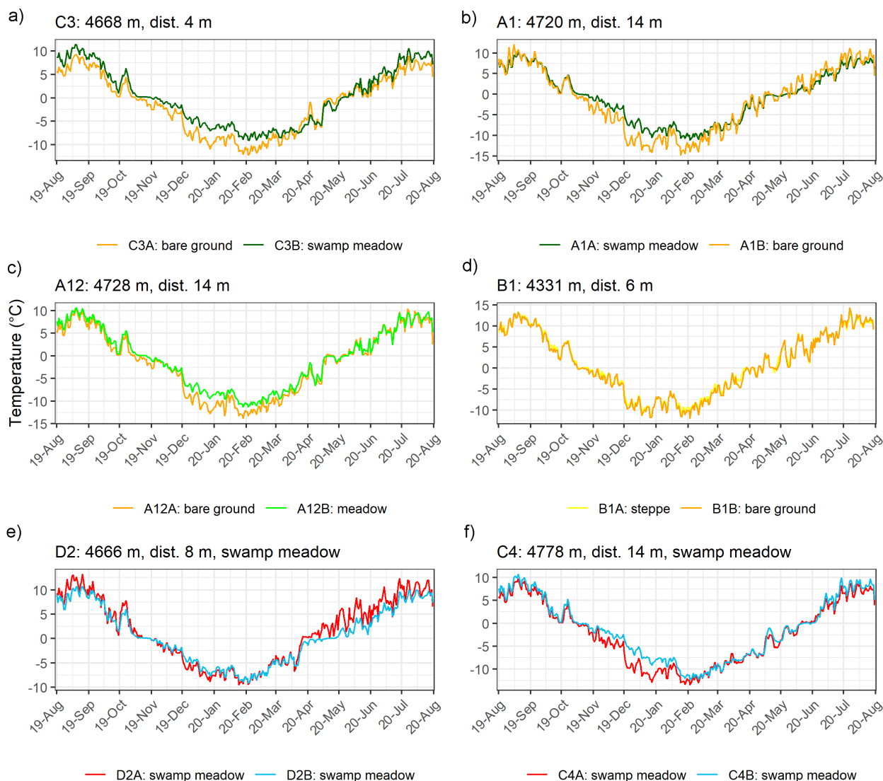
Figure 7. Evolution of the daily ground surface temperatures (GST) for period August 2019 – July 2020 at sites with different landcover between the paired plots: bare ground and alpine swamp meadow (a and b), bare ground and alpine meadow (c), bare ground and alpine steppe (d), and sites with alpine swamp meadow in both plots (e and f) in the south-central HAYR.
