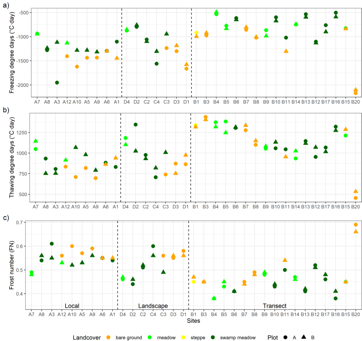
380 Figure 11. Freezing degree days (a), thawing degree days (b), and the frost number (c) at the depth of the ground surface temperature, approximately 5 cm into the ground, for the period August 2019 to July 2020 in both plots (A and B) of each site in south-central HAYR. Notes: Local scale (2 km 2 ), landscape scale (50 km 2 ), and elevational transect (800 m difference).
