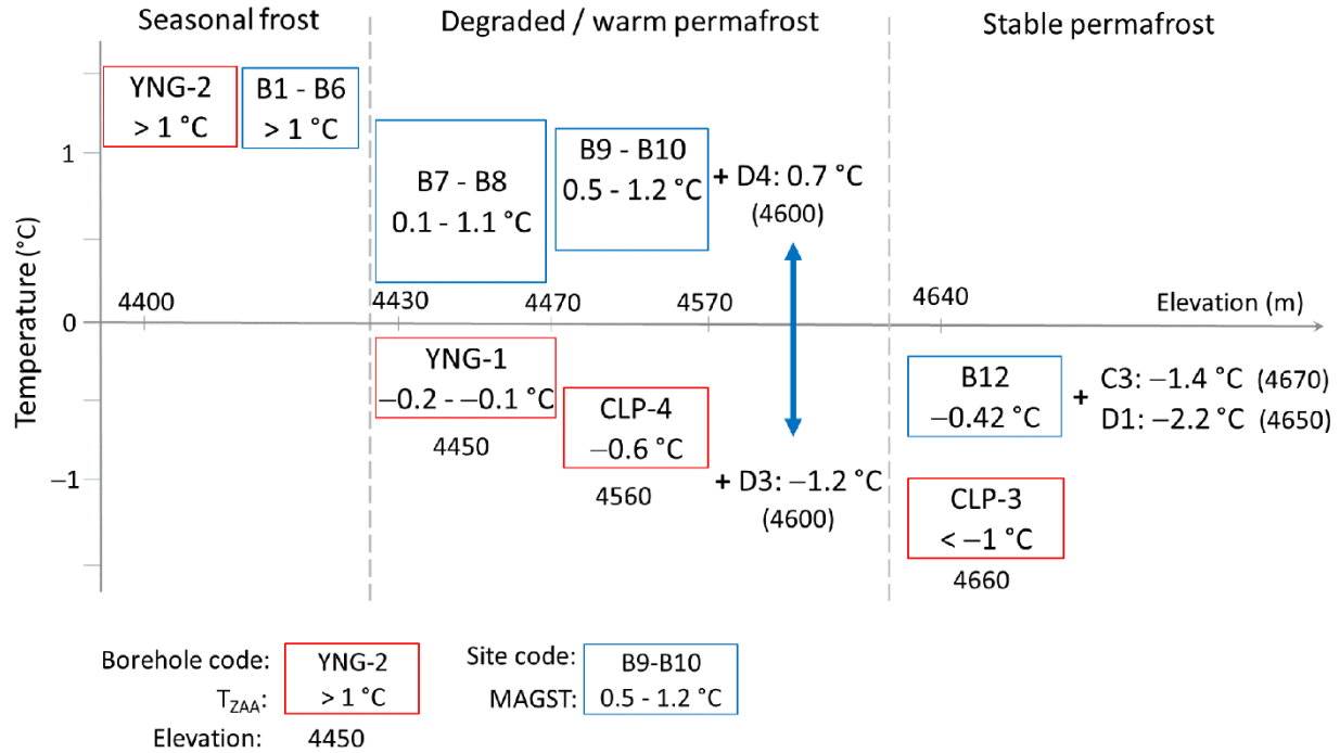
425 Figure 12. Comparison of the mean annual ground surface temperature (MAGST) for the period August 2019 to July 2020 in south-central HAYR with the multi-year (2010-2017) average temperatures at the depth of zero annual amplitude ( T_{ZAA} ) at depths of 10 and 15 m. Notes: Boreholes data are from Luo et al. (2018b), T_{ZAA} = Temperatures at the depth of zero annual amplitude (10 to 15 m).
