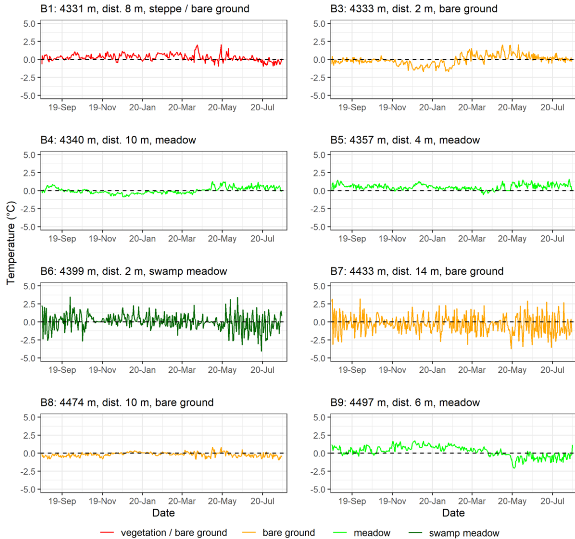
Figure 6. Intra-plot differences in daily GST for period August 2019 – July 2020 in sites B1 to B9 along the elevational transect in the south-central HAYR.
