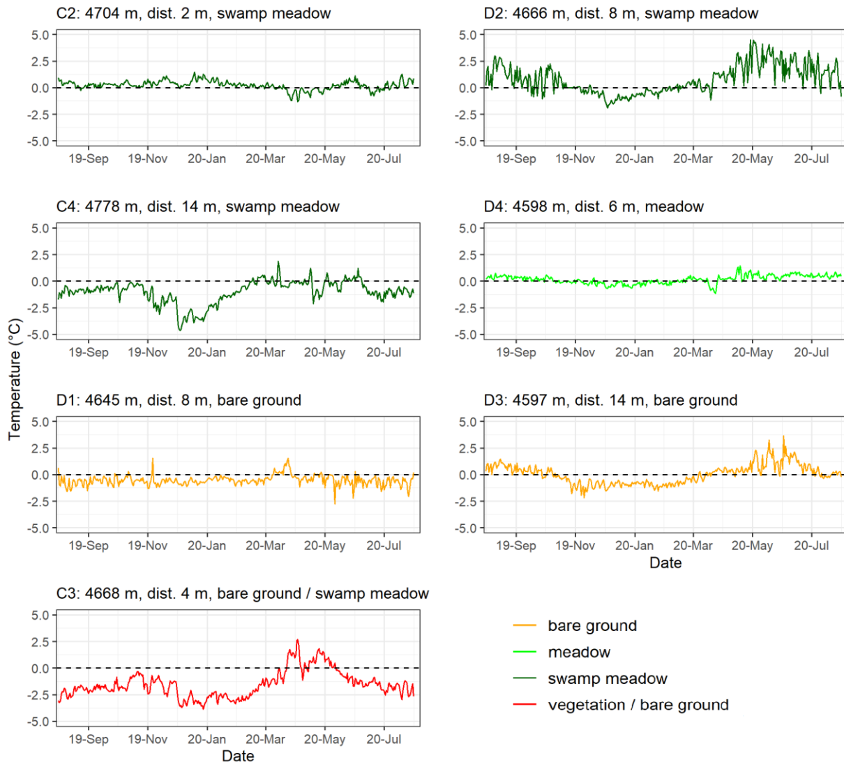
Figure 5. Intra-plot differences in daily GST for period August 2019 – July 2020 in sites at the landscape scale (50 km 2 ) on the Chalaping peat plateau in the south-central HAYR.
