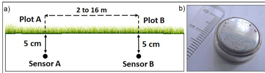
140 Figure 2. The schematic draw with the monitoring of GST at the fine-scale: the position of the two plots at distances from 2 to 16 m (a). Photo of the iButton temperature logger DS1922L (b). 145
