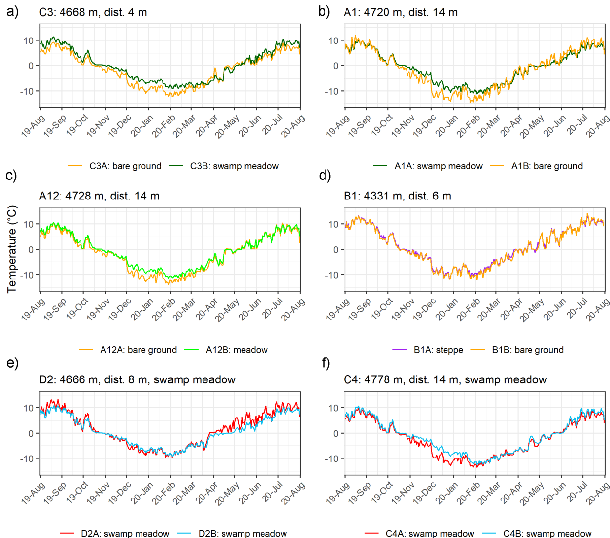
290 Figure 8. Evolution of the daily GST for period August 2019 – July 2020 at sites with different landcover between the paired plots: bare ground and alpine swamp meadow (a and b), bare ground and alpine meadow (c), bare ground and alpine steppe (d), and sites with alpine swamp meadow in both plots (e and f) in the south-central HAYR.
