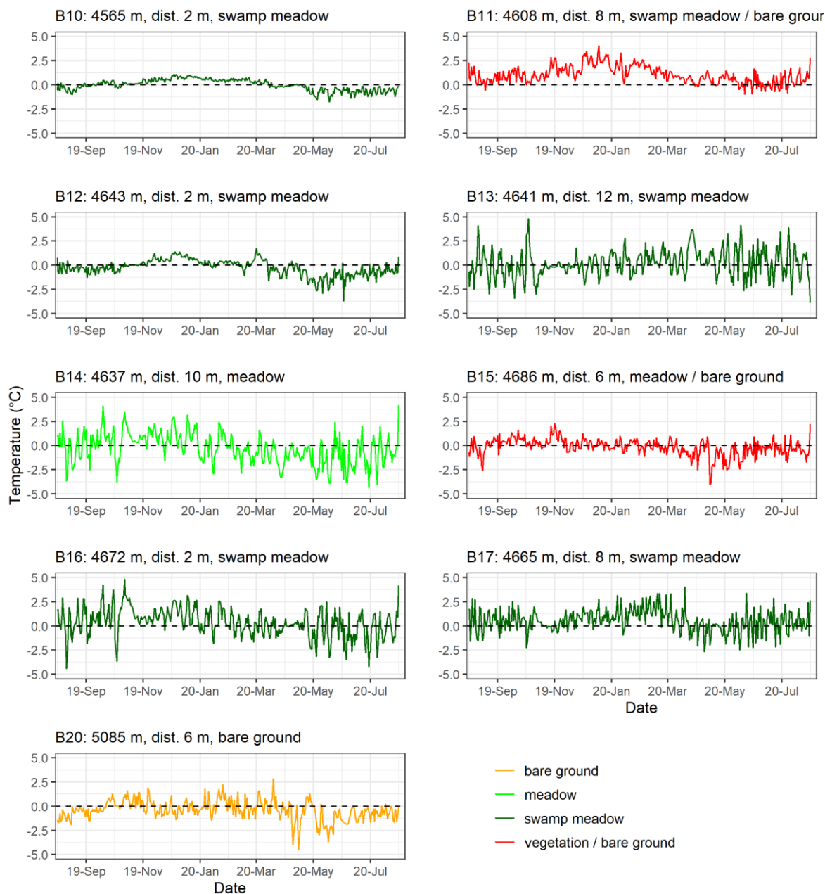
Figure 7. Intra-plot differences in daily GST for period August 2019 – July 2020 in sites B10 to B20 along the elevational transect in the south-central HAYR.
