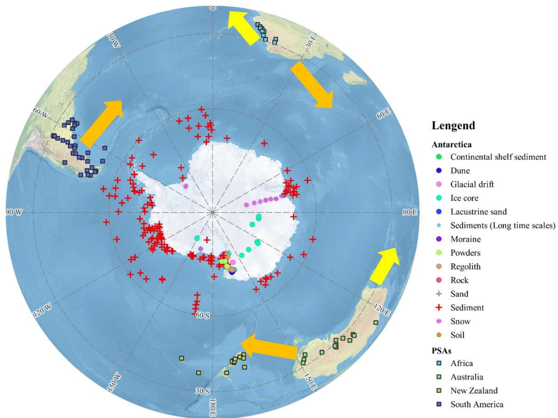
Fig. 7. The locations of the samples with marked in this database for Sr-Nd isotope ratios from Antarctica and PSAs in this database. The dust transport paths are marked with yellow arrows based on previous studies (Gaiero, 2007; Shao et al., 2010; Gili et al., 2021) (this figure was created with ArcGIS).
