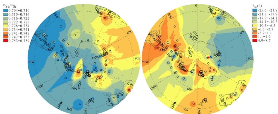
Fig. 8. Sr and Nd isotopic compositions of Holocene samples (black circles) from the AIS and ice-free areas on its periphery and aeolian dust samples (surface samples with no accurate ages) from PSAs in Australia, southern Africa and South America. The colours were determined by inverse distance weighted interpolation using ArcGIS.
