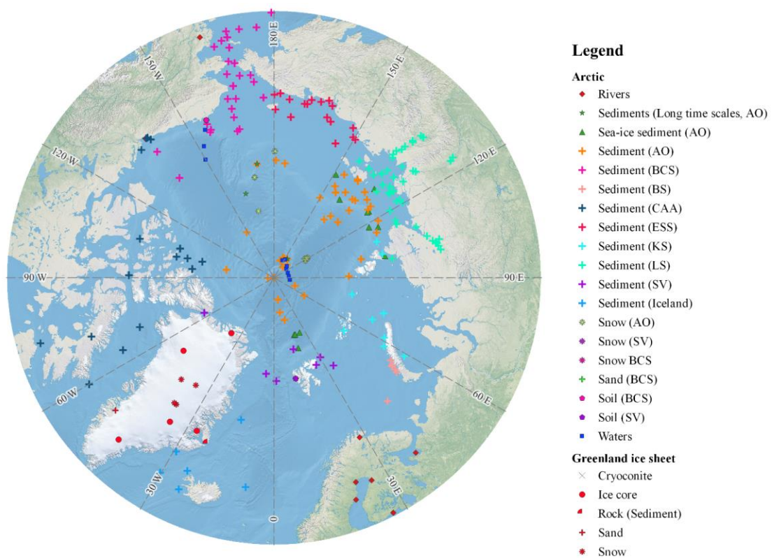
Fig. 4. Distribution of sampling sites in the Arctic. The types of samples are denoted with different shapes and colours (Table 3). (AO: Arctic Ocean; BCS: Bering-Chukchi Sea; BS: Barents Sea; CAA: Canadian Arctic Archipelago; ESS: East Siberian Sea; KS: Kara Sea; LS: Laptev Sea; SV: Svalbard) (this figure was created with ArcGIS).
