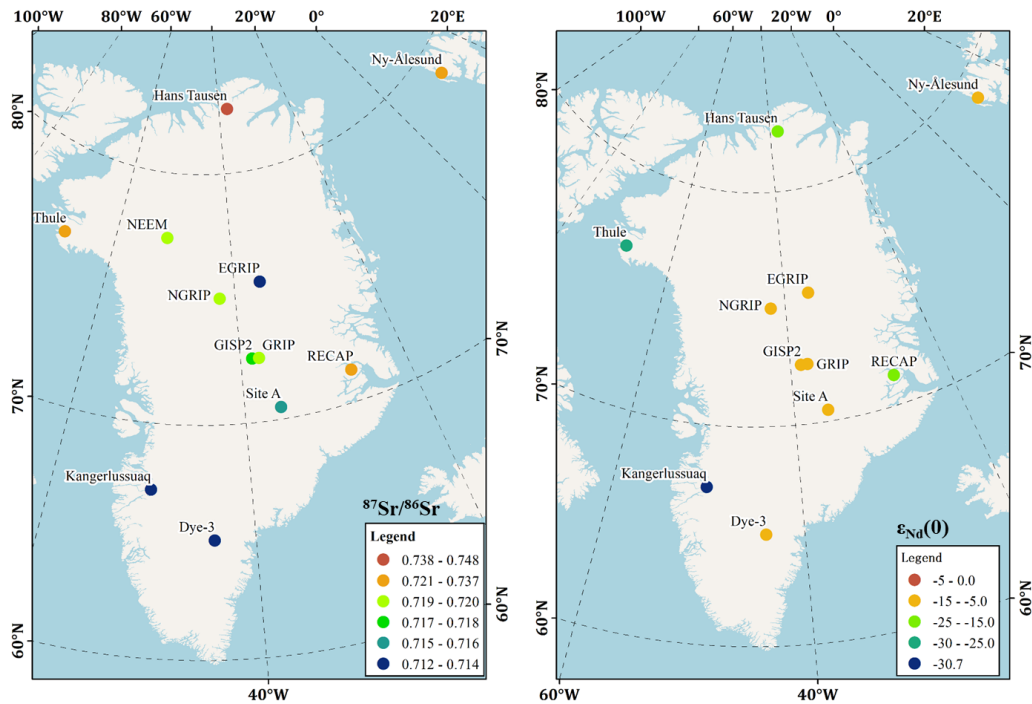
Fig. 5. ^{87}\text{Sr}/^{86}\text{Sr} and \epsilon_{\text{Nd}}(0) data in snow or ice cores and sand/soil samples from Ny-Ålesund, Svalbard and GrIS (this figure was created with ArcGIS).
