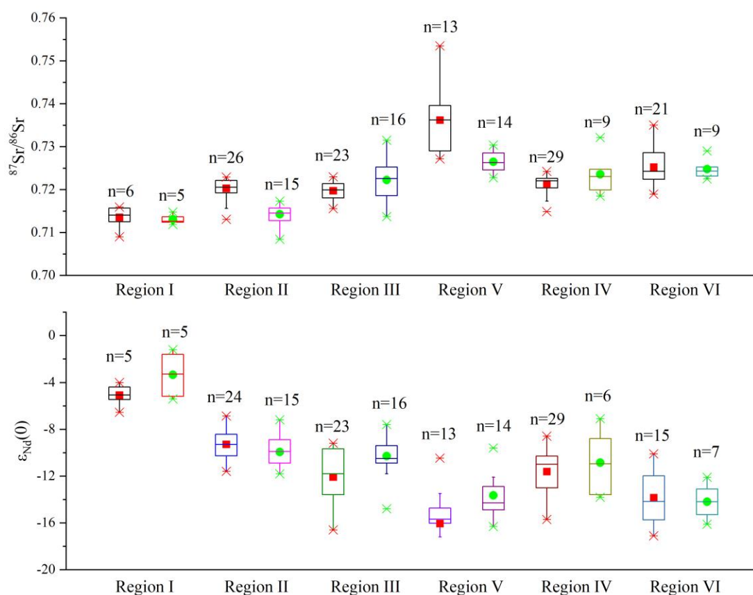
Fig. 3. Box plot for the Sr-Nd isotope signatures of Third Pole PSAs and snow samples. Samples are located in each PSA region based on the data from Table 2 (the number of samples for each sub-region are presented ( n > 5 )). The horizontal line within the box is the median, and the squares are the mean Sr-Nd values (red rectangles for sand or soil samples and green solid circles for snow samples). The interquartile range is represented by the lower and upper boundaries of the boxes, and whiskers indicate confidence intervals of 1.5 times the interquartile range.
