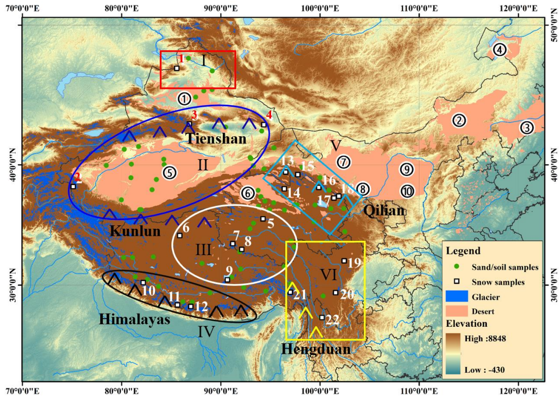
Fig. 2. The glacier and desert distributions in western China (the different coloured oval and rectangular shapes represent the six sub-regions (PSAs and glaciers) (Tienshan, Kunlun, Qilian, Himalayas and Hengduan Mountains) in the Third Pole; numbers and white squares represent 22 glaciers (snow samples were collected from these glaciers), for which the names of glaciers are shown in Table 2. The numbered circles represent the ten deserts or sandy areas in China (1. Gurbantunggut Desert, 2. Onqin Daga sandy land, 3. Horqin sandy land, 4. Hunlun Buir sandy land, 5. Taklimakan Desert, 6. Qaidam Desert, 7. Badain Jaran Desert, 8. Tengger Desert, 9. Hobq Desert, 10. Mu Us Desert). The green solid circles represent sand and soil
