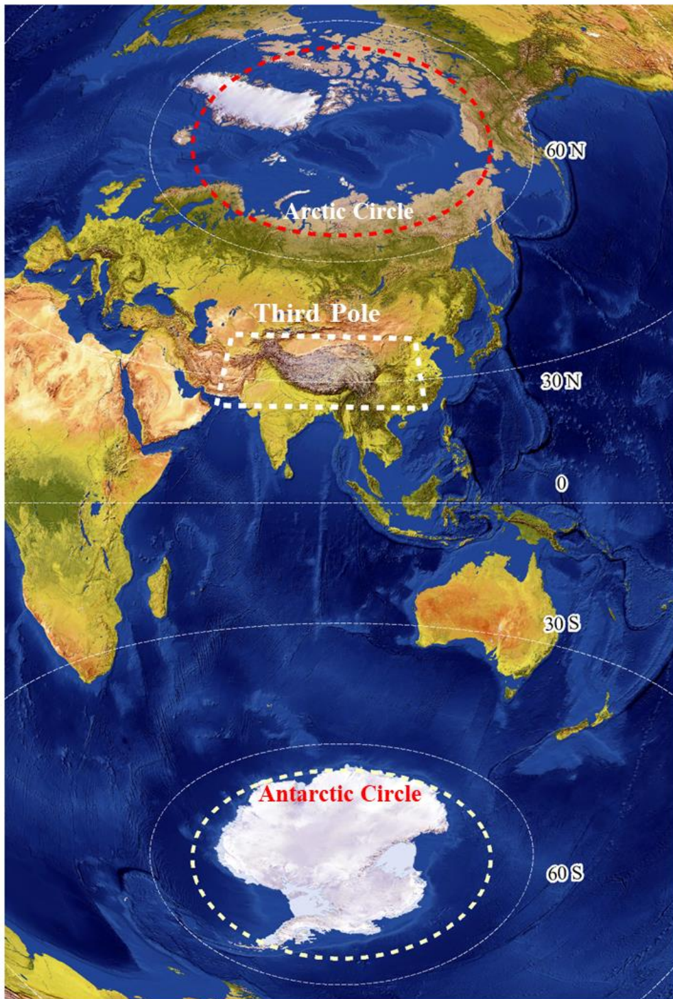
Fig. 1. Map of the sampling regions in the three poles (Third Pole: covering the high mountainous area in Asia, data were collected in the area of 40^{\circ} to 23^{\circ} N and 106^{\circ} to 61^{\circ} E, Li et al., 2020; Arctic: from the high Arctic to the sub-Arctic areas, data were collected from >60^{\circ} N in this region); and Antarctica: data were collected from >60^{\circ} S
