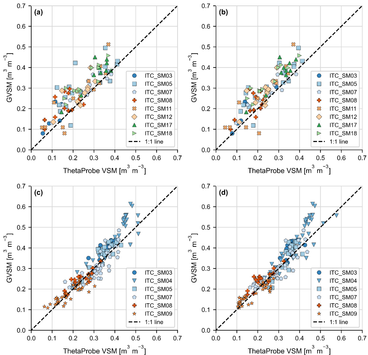
Figure 6: Scatter plots of the ThetaProbe VSM against GVSM collected during the 2009 (a and b) and 2015 (c and d) field campaigns. In subplots a) and c) are the ThetaProbe VSM readings taken next to a GVSM measurement. In subplots b) and d) are the mean of the ThetaProbe VSM readings taken at a sampling point.
