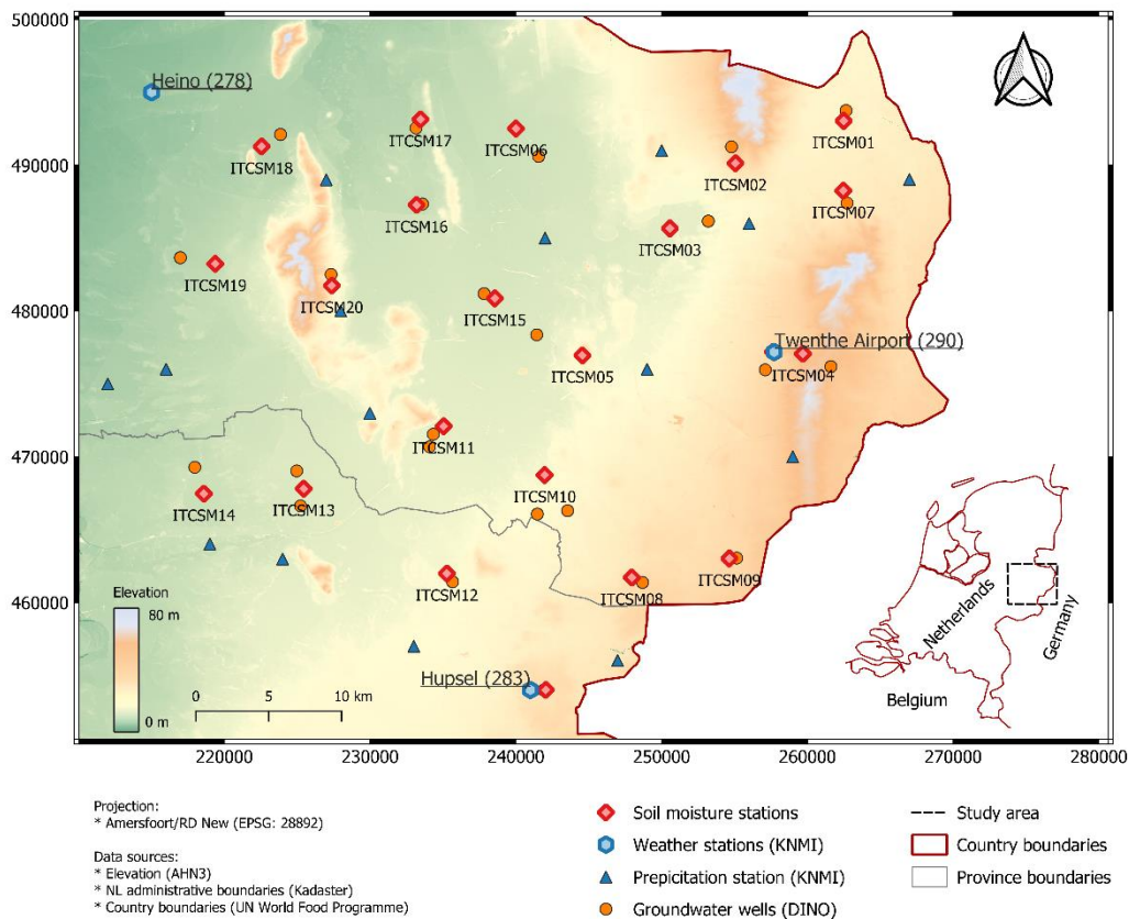
815 Figure 1: The topography of the study area (source: 5 m spatial resolution AHN3; AHN, 2019) and the locations of the soil moisture/temperature monitoring stations, KNMI automated weather stations (underlined with ID in parenthesis), KNMI precipitation stations and groundwater monitoring wells available in DINO Loket.
