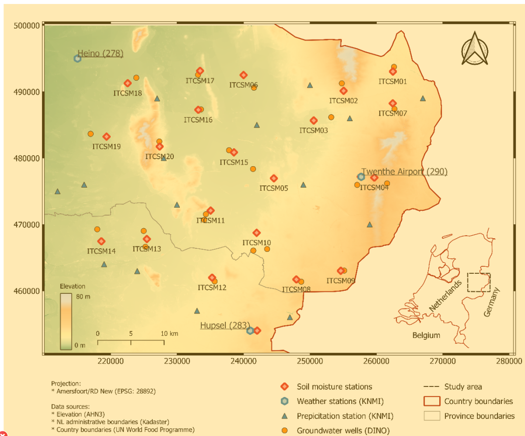
830 Figure 4: The topography of the study area (source: 5 m spatial resolution AHN3; AHN, 2019) and the locations of the soil moisture/temperature monitoring stations, KNMI automated weather stations (underlined with ID in parenthesis), KNMI precipitation stations and groundwater monitoring wells available in DINO Loket.
