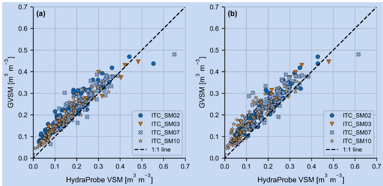
855 Figure 7: Scatter plots with the HydraProbe VSM against the GVSM collected during the 2016 and 2017 field campaigns. In subplot a) is the HydraProbe VSM reading taken next to the GVSM measurement. In subplot b) is the mean of the HydraProbe VSM readings taken at the sampling point.
