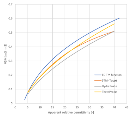
Figure R1: \varepsilon_r against VSM using the mineral soil calibrations provided for the EC-TM, 5TM, ThetaProbe and HydraProbe.
