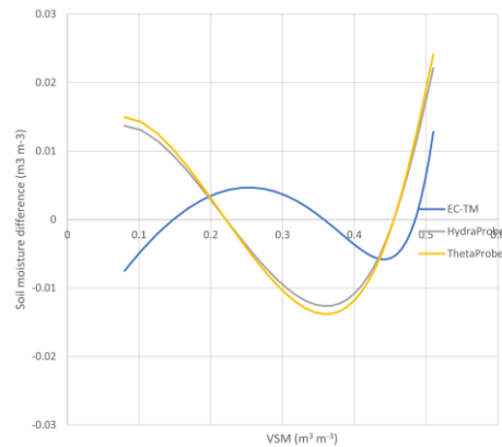
Figure R3: VSM difference between the EC-TM, ThetaProbe and HydraProbe VSM and the 5TM VSM matched through application of established linear fits.
