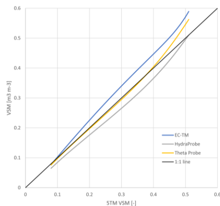
Figure R2: EC-TM, ThetaProbe and HydraProbe VSM against the 5TM VSM.
