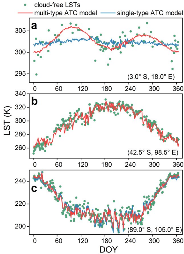
240 Fig. 3. Comparison of reconstructing under-cloud LSTs with multi-type and single-type ATC models at different latitudes. (a), (b), and (c) show three examples of ATC modelling at low-latitudes, mid-latitudes, and high-latitudes for cloud-free Terra-day LST in 2019. The green circles, blue lines, and red lines denote the cloud-free observations and LSTs simulated by the single- and multi-type ATC models, respectively. Note that for (b) the results of the single- and multi-type ATC models are identical since they both use the ATC model with single-sinusoidal function.
