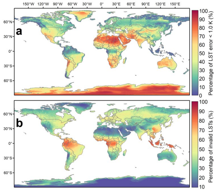
665 Fig. A2. Uncertainties of the downloaded MODIS MXD11C1 V6 LSTs. (a) shows the percentage of LSTs with a retrieval error less than 1.0 K; and (b) displays the percentage of invalid data ( \approx clouds).
