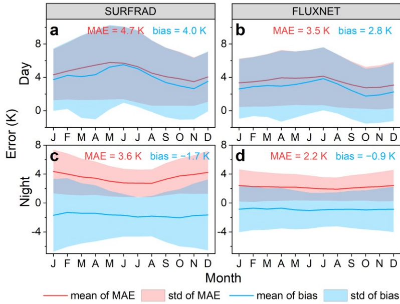
Fig. 5. Validations of reconstructed under-cloud LSTs at Aqua and Terra day and night overpass times based exclusively on in situ data. The under-cloud LSTs were reconstructed with the ATC model. (a) and (b) show monthly mean errors obtained for daytime overpasses (including Aqua-day and Terra-day) for SURFRAD and FLUXNET data, respectively; (c) and (d) show the same for the nighttime overpasses (including Aqua-night and Terra-night).
