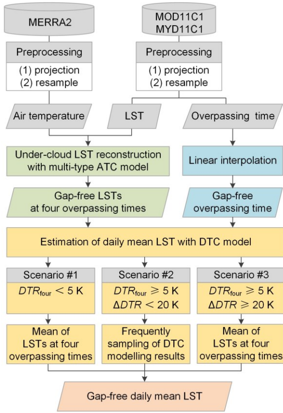
Fig. 2. Flowchart of the IADTC framework. DTR_{\text{four}} refers to diurnal temperature range (DTR) calculated as the maximum minus the minimum from the gap-free LSTs at the four overpassing times; DTR_{\text{DTC}} refers to the DTR calculated from the hourly LSTs modelled with the DTC model. \Delta DTR refers to the absolute difference between DTR_{\text{four}} and DTR_{\text{DTC}} .
