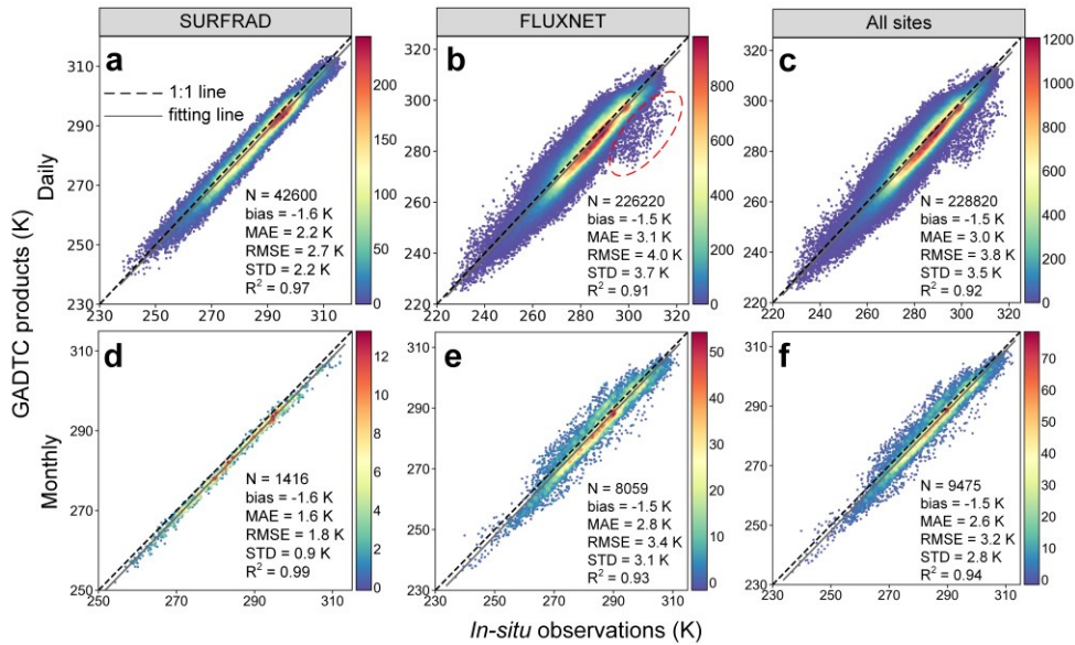
Fig. 8. GADTC products versus in situ observations. (a), (b), and (c) compare the daily mean LST over the SURFRAD, FLUXNET, and combined sites, respectively; and (d), (e), and (f) show the corresponding results for monthly mean LST. The biases were calculated by the GADTC products minus the in situ measurements. The red ellipse in (b) highlights the cases with notably large errors.
