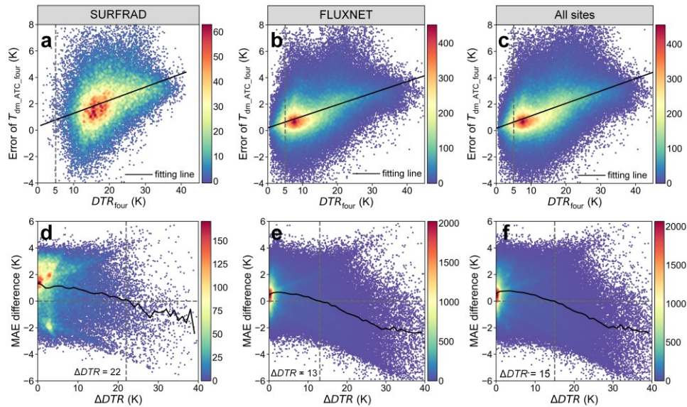
Fig. 11. Threshold determination for the two criteria in Fig. 2Fig-2. (a), (b) and (c) display the errors of T_{dm\_ATC\_four} ( T_{dm\_ATC\_four} minus T_{dm\_true} ) depending on DTR_{four} for SURFRAD, FLUXNET, and combined data, respectively; and (d), (e) and (f) display the MAE differences between T_{dm\_ATC\_four} and T_{dm\_ATC\_DTC} (i.e., the MAE of T_{dm\_ATC\_four} minus the MAE of T_{dm\_ATC\_DTC} ) depending on the \Delta DTR for SURFRAD, FLUXNET, and combined data, respectively. The black lines in (d), (e) and (f) denote the averaged MAE difference within every unit along the x-axis.
