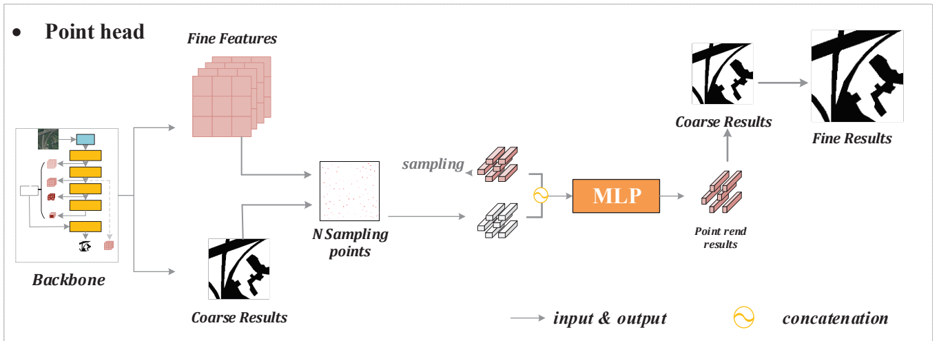
Figure 7. Structure of the enhanced-Coordinate-attention (ECA)-module point head in UGSNet. Given the fine features and the coarse UGS results from the backbone, the point head will firstly collect N sampling points with lowest certainty to construct point-wise features, which will be input into a MLP for classification and help obtain fine UGS results.
