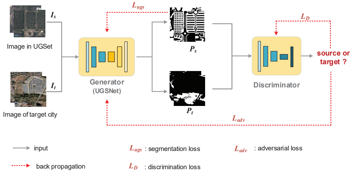
Figure 5. Flowchart of the proposed deep learning framework for UGS mapping (The "Image in UGSet" were retrieved from GF-2/Gaofen-2 2019, whiel while the "Image of target city" © Google Earth 2020). The red dashed lines denote the loss of back propagation for model optimization. The L_{ugs} , L_D , and L_{adv} represent the segmentation loss, the discrimination loss, and the adversarial loss, as described in Sect. 3.3.
