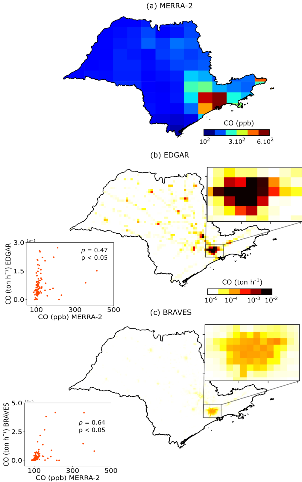
Figure 10. CO spatial distribution provided by a) MERRA-2, b) EDGAR, and c) BRAVES. Scatter plots of CO vehicle emission and CO hourly surface concentrations in SP on 01/01/2015 at 8:00.
