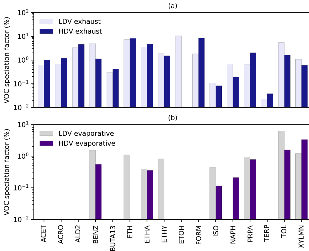
Figure 5. VOC chemical speciation factor for (a) exhaust and (b) evaporative emissions from light and heavy vehicle article. Data derived from US EPA SPECIATE 5.1 (US EPA, 2020; Eyth et al. 2020).
