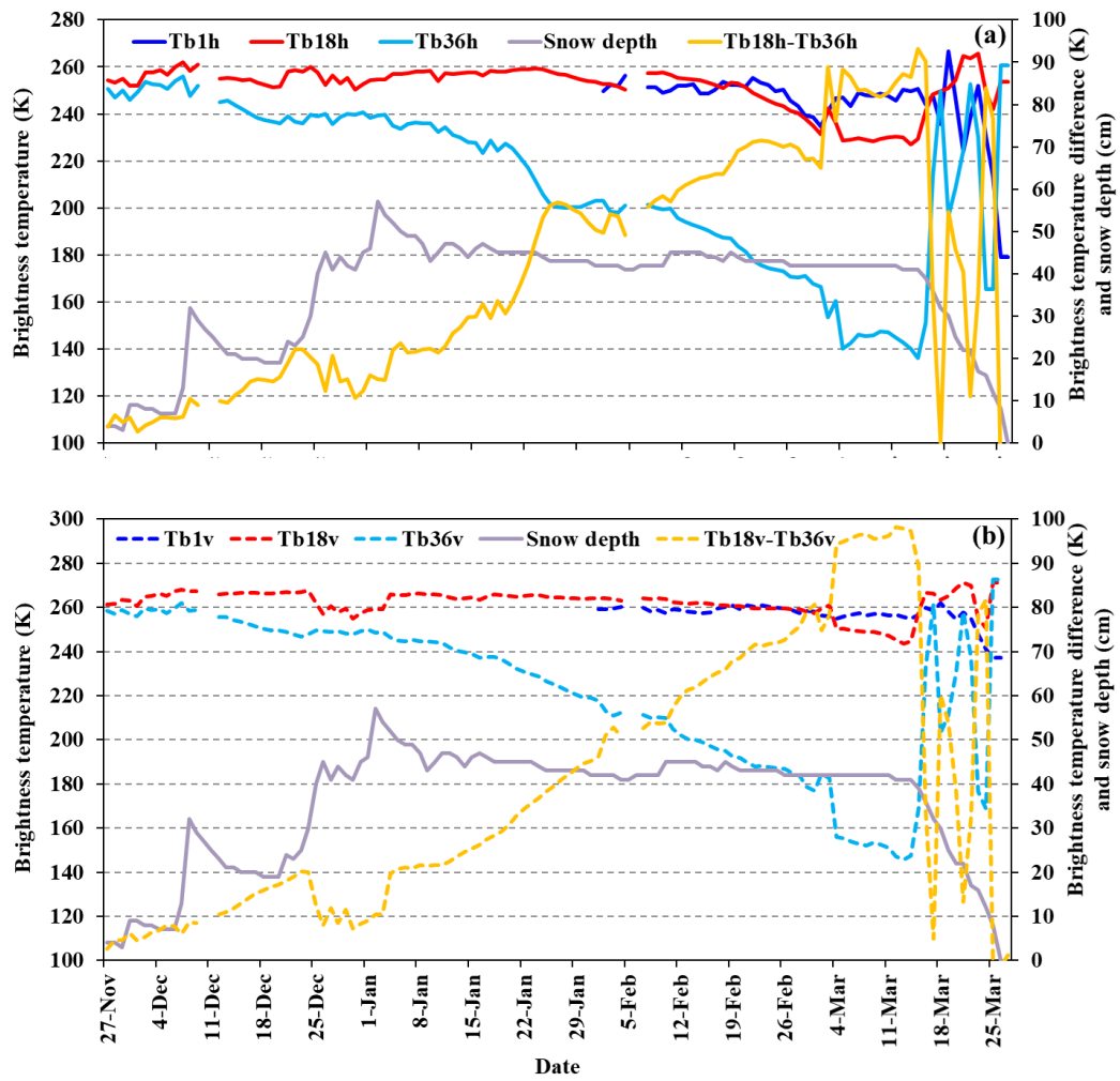
381 Figure 12. Daily variations in brightness temperatures at 1.4 GHz, 18 GHz and 36 GHz, for horizontal 382 (Tb1h, Tb18h, Tb36h) and vertical polarizations (Tb1v, Tb18v, Tb36v), the differences between Tb18h and 383 Tb36h (Tb18h - Tb36h), and between Tb18v and Tb36v (Tb18v - Tb36v), at 1:00 am local time, from 384 November 27, 2015 to March 26, 2016. (a) for horizontal polarization, and (b) for vertical polarization.
