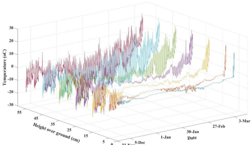
345 346 Figure 10. Minutely variation in snow temperatures at 0 cm (snow/soil interface), 5 cm, 15 cm, 25 cm, 35 cm, 347 45 cm and 55 cm above ground during experiment period
