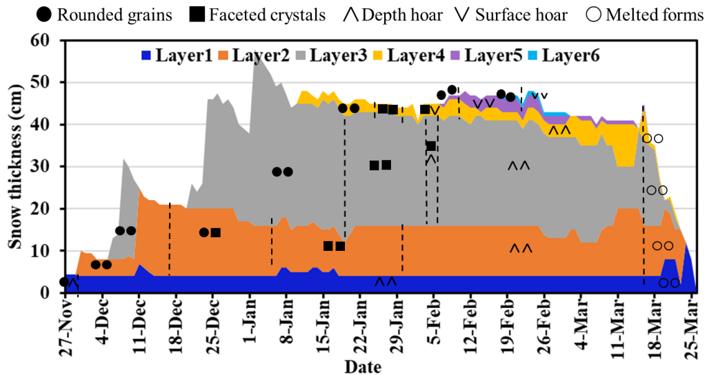
314 315 Figure 7. Daily variation in snow layers and grain shape in each layer from November 27, 2015 to March 25, 316 2016.
