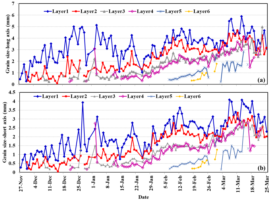
318 319 Figure 8. Daily variation in grain size within each layer from November 27, 2015 to March 25, 2016. The layer 320 thicknesses are presented in figure 7.
