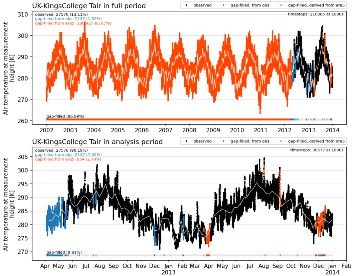
Figure 3: Forcing timeseries with gap filling. Example shown for air temperature (Tair) at Kings College, London (UK-KingsCollege); (a) full forcing period, including 10 years of ERA5-derived data (red) prior to observations (black) used for model spin up, and (b) focus period used for analysis. Gaps are first filled from nearby tower measurements where available, and short gaps ( \leq 2 hours) are linearly interpolated (blue). Remaining gaps are filled using the ERA5-derived timeseries which is seasonally and diurnally bias corrected using site observations. White lines show seven day mean values. Similar plots are available for other sites within the site data collection (Lipson et al., 2022).
