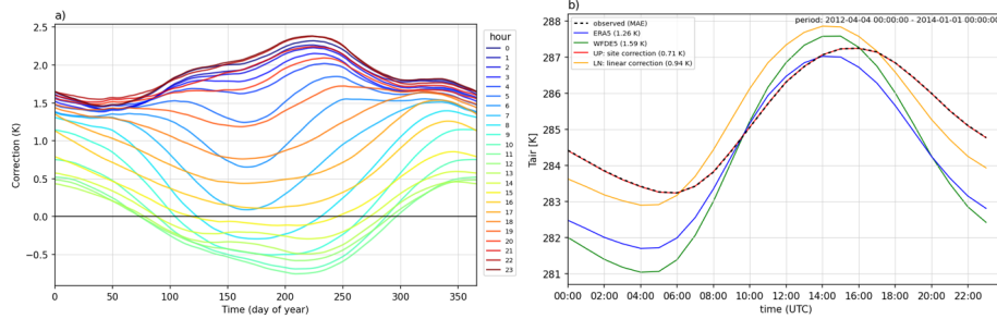
Figure 4: Urban-PLUMBER reanalysis bias correction methods. Demonstrated using air temperature ( T_{air} ) for the grid containing the King’s College London site (UK-KingsCollege). (a) hourly (colour) bias calculated for each day of a ‘representative’ year and applied to entire ERA5 timeseries; (b) diurnal hourly mean Urban-PLUMBER correction (UP, red), observations (black), original ERA5 data (blue), WFDE5 bias corrected data (green) and linear bias correction method used in FLUXNET (LN, yellow). Our new UP method has smaller mean absolute errors (MAE) overall, and can correct both pattern and phase errors of ERA5 (Section 3).
