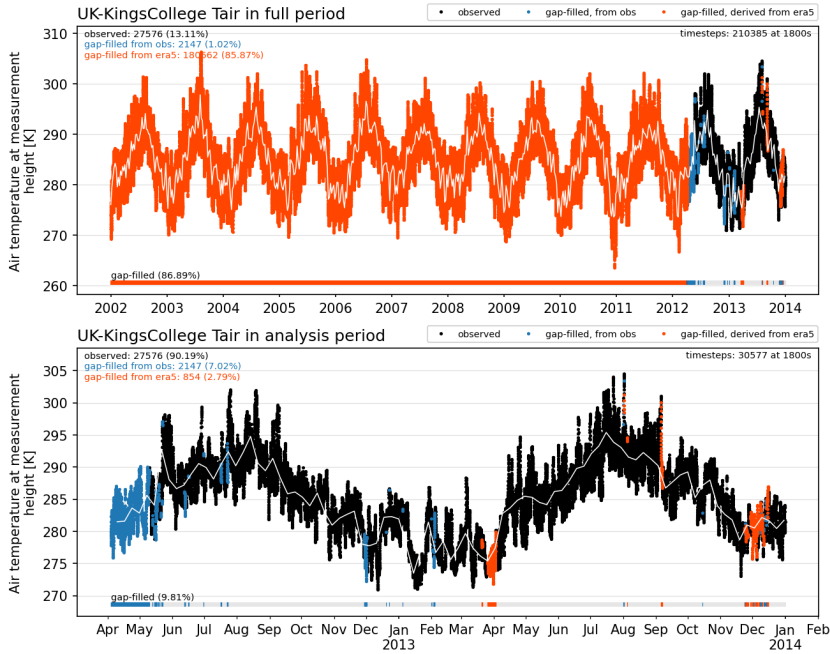
170 Figure 3: Forcing timeseries with gap filling. Example shown for air temperature ( T_{air} ) at Kings College, London (UK-KingsCollege); (a) full forcing period, including 10 years of ERA5-derived data (red) prior to observations (black) used for model spin up, and (b) focus period used for analysis. Gaps are first filled from nearby tower measurements where available, and short gaps ( \leq 2 hours) are linearly interpolated (blue). Remaining gaps are filled using the ERA5-derived timeseries which is seasonally and diurnally bias corrected using site observations. White lines show seven day mean values. Similar plots are available for other sites within the site data collection (Lipson et al., 2022).
