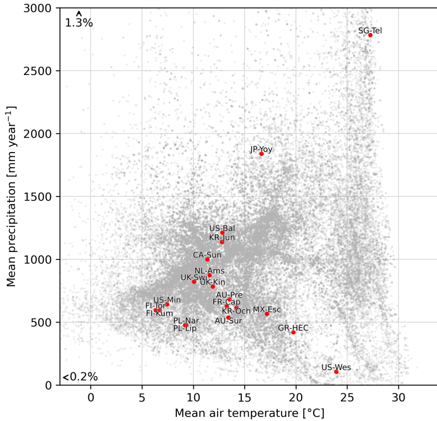
150 Figure 2: Climatology of included sites compared with more than 70,000 global urban areas. Mean temperature and annual precipitation at the 20 tower sites (red, truncated site name, Table 1) from tower observations; global urban locations (grey) from ERA5 surface data (Hersbach et al., 2020, 2018) (2000 – 2010) from grid nearest to locations identified in the Global Rural-Urban Mapping Project (GRUMP) (Center for International Earth Science Information Network - CIESIN - Columbia University et al., 2017). Locations with rainfall above 3000 mm year -1 (1.3% of locations), and mean temperature below -3°C (0.2% of locations) are not shown.
