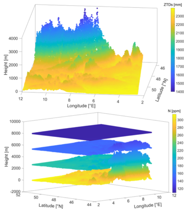
Figure 3. Fields of collocated (top) GNSS ZTDs and (bottom) refractivities.
